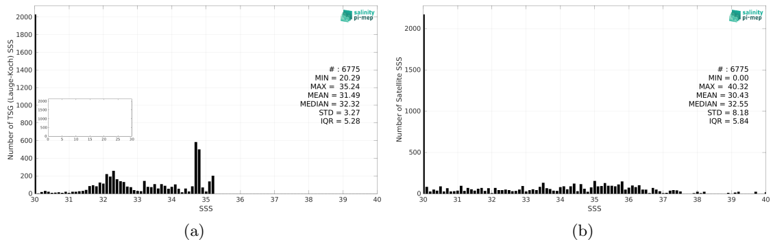
Figure 2: Histograms of SSS from TSG (Lauge-Koch) (a) and SMAP SSS L2 v5.0 (JPL) (b) considering all match-up pairs per bins of 0.1 over the Arctic Ocean Pi-MEP region and for the full satellite product period.
