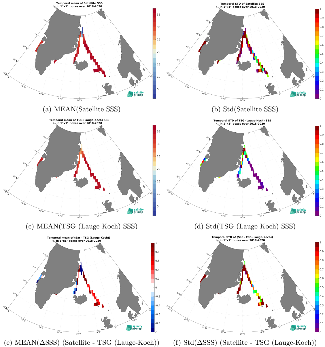
Figure 6: Temporal mean (left) and Std (right) of SSS from SMAP SSS L2 v5.0 (JPL) (top), TSG (Lauge-Koch) (middle), and of \Delta SSS (Satellite - TSG (Lauge-Koch)). Only match-up pairs are used to generate these maps.
