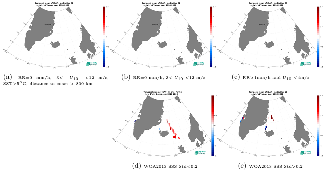
Figure 12: Temporal mean gridded over spatial boxes of size 1^{\circ}\times 1^{\circ} of \Delta\text{SSS} (SMAP SSS L2 v5.0 (JPL) - TSG (Lauge-Koch)) for 5 different subdatasets corresponding to:RR=0 mm/h, 3 < U_{10} < 12 m/s, SST > 5^{\circ}\text{C} , distance to coast > 800 km (a), RR=0 mm/h, 3 < U_{10} < 12 m/s (b), RR > 1 mm/h and U_{10} < 4 m/s (c), WOA2013 SSS Std < 0.2 (d), WOA2013 SSS Std > 0.2 (e).
