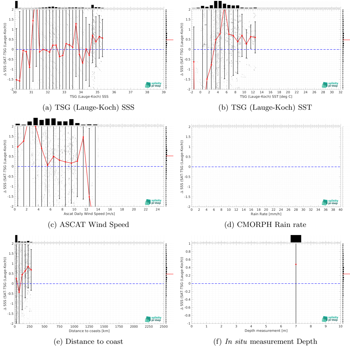
Figure 11: \Delta SSS (Satellite - TSG (Laugé-Koch)) sorted as function of TSG (Laugé-Koch) SSS values a), TSG (Laugé-Koch) SST b), ASCAT Wind speed c), CMORPH rain rate d), distance to coast (e) and in situ measurement depth (f). In all plots the median and Std of \Delta SSS for each bin is indicated by the red curves and black vertical thick bars ( \pm 1 Std)
