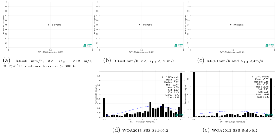
Figure 13: Normalized histogram of \Delta SSS (SMAP SSS L2 v5.0 (JPL) - TSG (Laue-Koch)) for 5 different subdatasets corresponding to: RR=0 mm/h, 3 < U_{10} < 12 m/s, SST > 5°C, distance to coast > 800 km (a), RR=0 mm/h, 3 < U_{10} < 12 m/s (b), RR > 1mm/h and U_{10} < 4 m/s (c), WOA2013 SSS Std < 0.2 (d), WOA2013 SSS Std > 0.2 (e).
