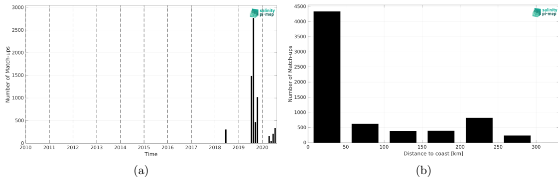
Figure 1: Number of match-ups between TSG (Lauge-Koch) and SMAP SSS L2 v5.0 (JPL) SSS as a function of time (a) and as function of the distance to coast (b) over the Arctic Ocean Pi-MEP region and for the full satellite product period.
