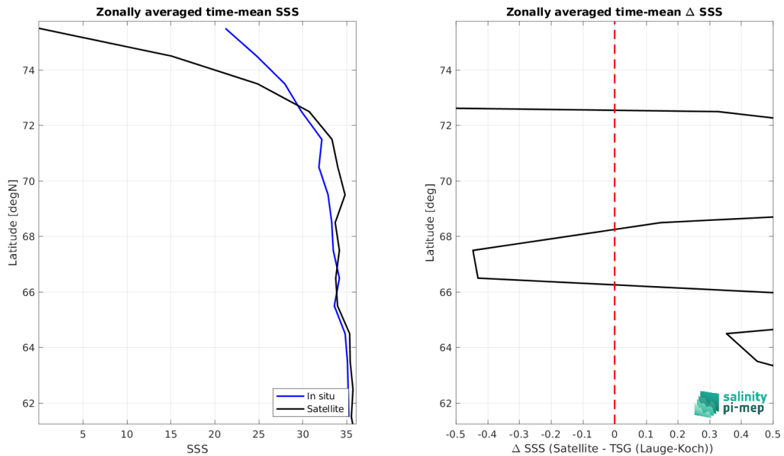
Figure 8: Left panel: Zonal mean SSS from SMAP SSS L2 v5.0 (JPL) satellite product (black) and from TSG (Lauge-Koch) (blue). Right panel: Zonal mean of \Delta SSS (Satellite - TSG (Lauge-Koch)) for all the collected Pi-MEP match-up pairs estimated over the full satellite product period.
