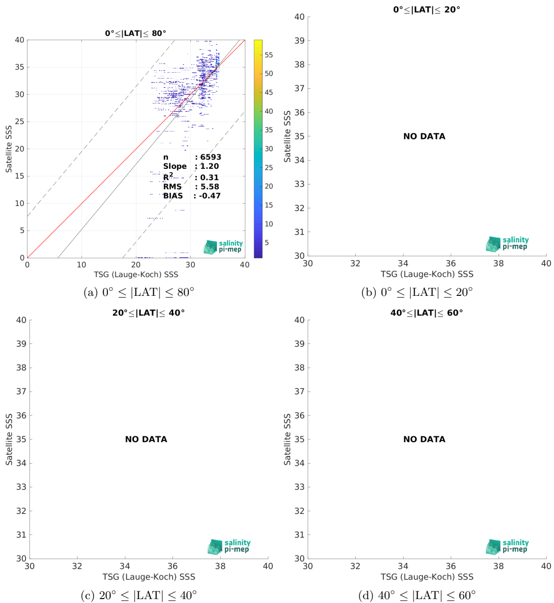
Figure 9: Contour maps of the concentration of SMAP SSS L2 v5.0 (JPL) SSS (y-axis) versus TSG (Lauge-Koch) SSS (x-axis) at match-up pairs for different latitude bands. For each plot, the red line shows x=y . The black thin and dashed lines indicate a linear fit through the data cloud and the \pm 95\% confidence levels, respectively. The number match-up pairs n , the slope and R^2 coefficient of the linear fit, the root mean square (RMS) and the mean bias between satellite and in situ data are indicated for each latitude band in each plots.
