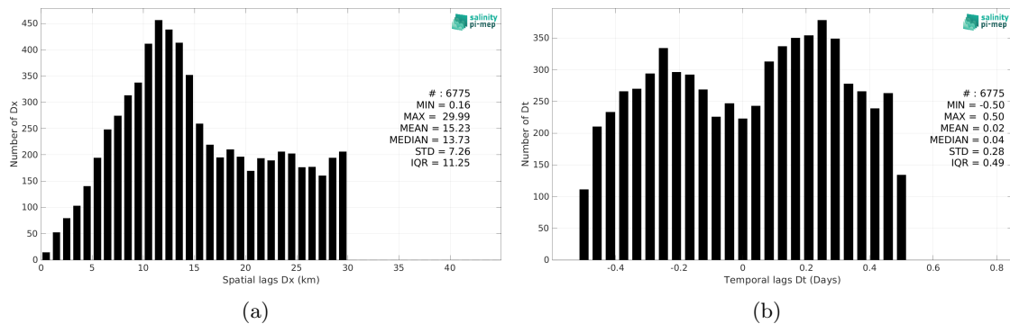
Figure 5: Histograms of the spatial (a) and temporal (b) lags between the location/time of the TSG (Lauge-Koch) measurement and the date of the corresponding SMAP SSS L2 v5.0 (JPL) SSS pixel.
