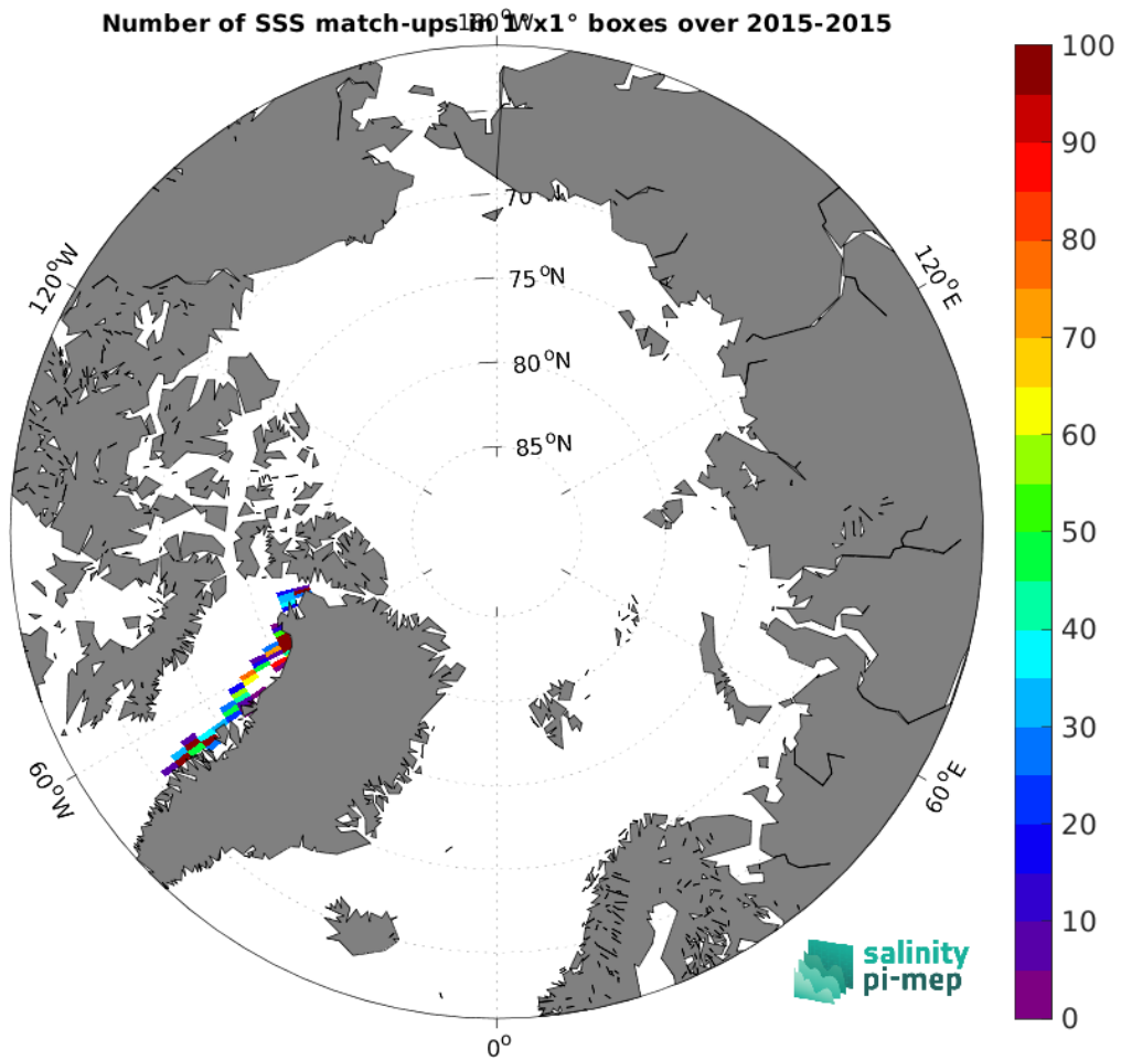
Figure 4: Number of SSS match-ups between TSG (GOSUD-Sailing-ship) SSS and the SMAP SSS L2 v5.0 (JPL) SSS product for the Arctic Ocean Pi-MEP region over 1^\circ \times 1^\circ boxes and for the full satellite product period.
