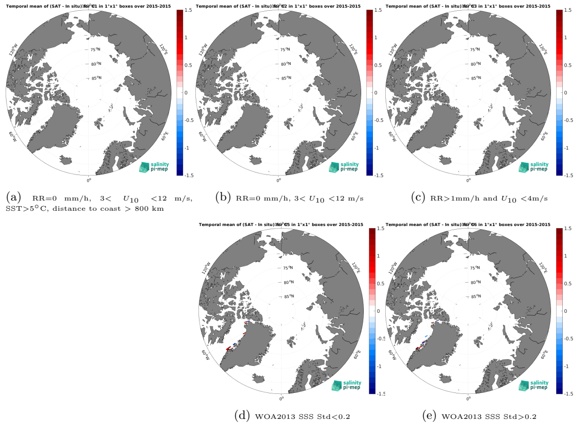
Figure 12: Temporal mean gridded over spatial boxes of size 1^{\circ} \times 1^{\circ} of \Delta SSS (SMAP SSS L2 v5.0 (JPL) - TSG (GOSUD-Sailing-ship)) for 5 different subdatasets corresponding to: RR=0 mm/h, 3 < U_{10} < 12 m/s, SST > 5°C, distance to coast > 800 km (a), RR=0 mm/h, 3 < U_{10} < 12 m/s (b), RR > 1mm/h and U_{10} < 4 m/s (c), WOA2013 SSS Std < 0.2 (d), WOA2013 SSS Std > 0.2 (e).
