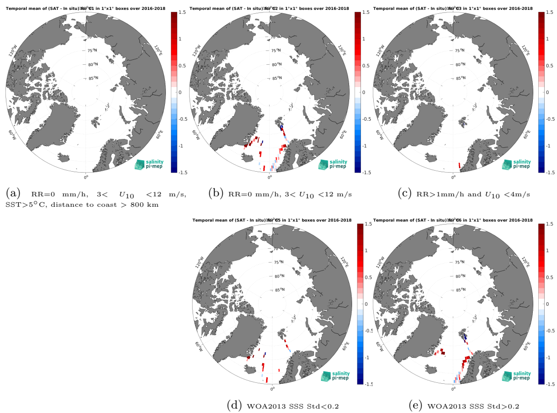
Figure 14: Temporal mean gridded over spatial boxes of size 1^\circ \times 1^\circ of \Delta\text{SSS} (SMAP SSS L2 v5.0 (JPL) - TSG (GOSUD-Research-vessel)) for 5 different subdatasets corresponding to:RR=0 mm/h, 3 < U_{10} < 12 m/s, SST > 5°C, distance to coast > 800 km (a), RR=0 mm/h, 3 < U_{10} < 12 m/s (b), RR > 1mm/h and U_{10} < 4 m/s (c), WOA2013 SSS Std < 0.2 (d), WOA2013 SSS Std > 0.2 (e).
