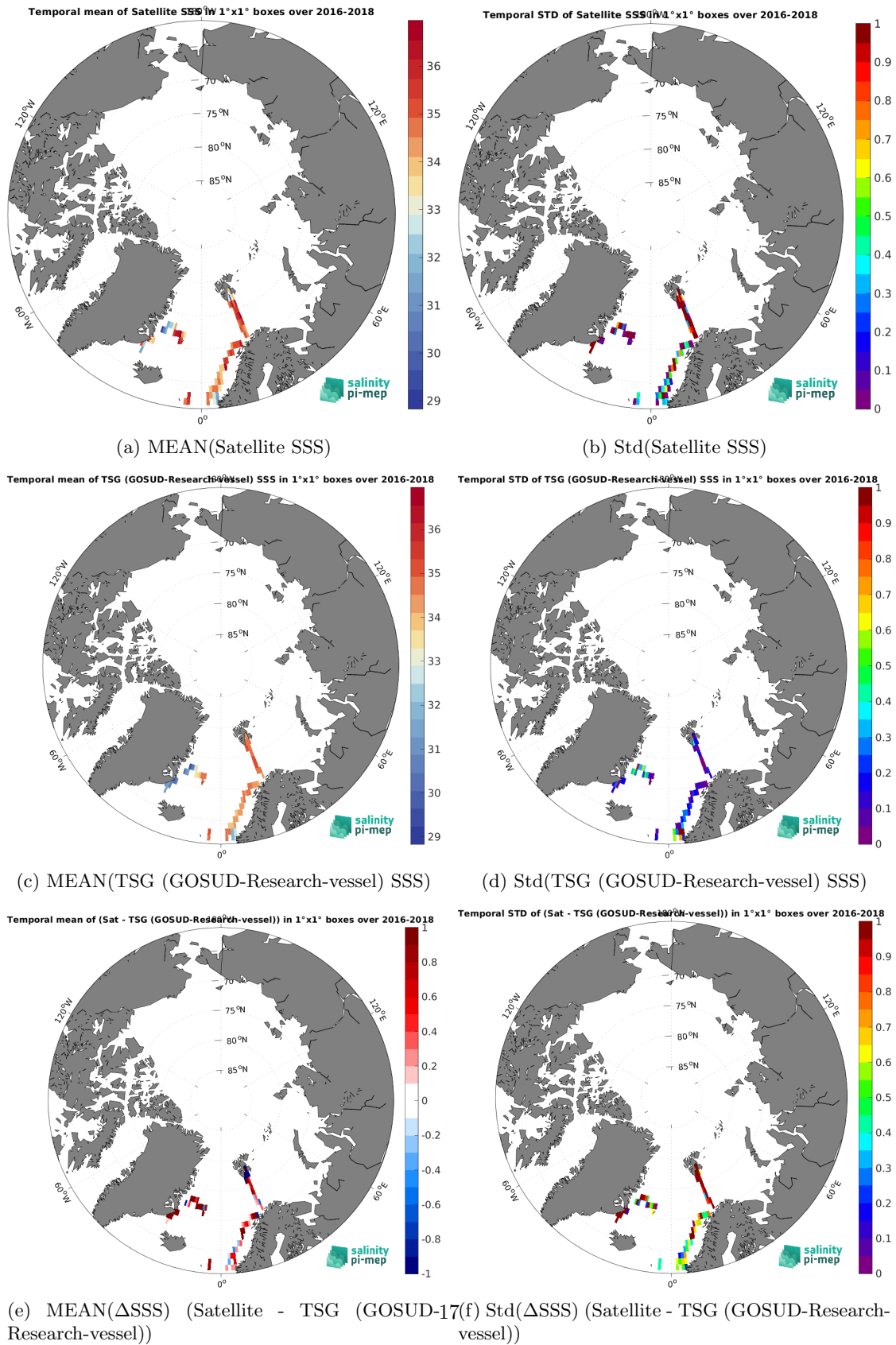
Figure 7: Temporal mean (left) and Std (right) of SSS from SMAP SSS L2 v5.0 (JPL) (top), TSG (GOSUD-Research-vessel) (middle), and of \Delta SSS (Satellite - TSG (GOSUD-Research-vessel)). Only match-up pairs are used to generate these maps.
