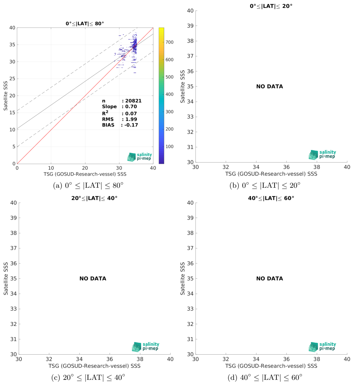
Figure 10: Contour maps of the concentration of SMAP SSS L2 v5.0 (JPL) SSS (y-axis) versus TSG (GOSUD-Research-vessel) SSS (x-axis) at match-up pairs for different latitude bands. For each plot, the red line shows x=y . The black thin and dashed lines indicate a linear fit through the data cloud and the \pm 95\% confidence levels, respectively. The number match-up pairs n , the slope and R^2 coefficient of the linear fit, the root mean square (RMS) and the mean bias between satellite and in situ data are indicated for each latitude band in each plots.
