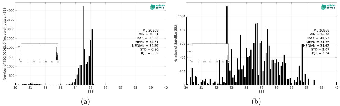
Figure 3: Histograms of SSS from TSG (GOSUD-Research-vessel) (a) and SMAP SSS L2 v5.0 (JPL) (b) considering all match-up pairs per bins of 0.1 over the Arctic Ocean Pi-MEP region and for the full satellite product period.
