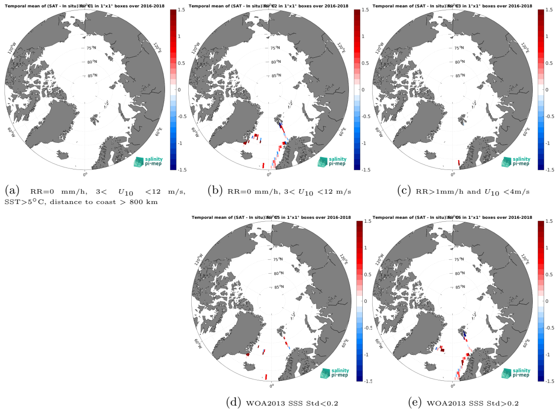
Figure 14: Temporal mean gridded over spatial boxes of size 1^\circ \times 1^\circ of \Delta SSS (SMAP SSS L2 v5.0 (JPL) - TSG (GOSUD-Research-vessel)) for 5 different subdatasets corresponding to:RR=0 mm/h, 3 < U_{10} < 12 m/s, SST > 5°C, distance to coast > 800 km (a), RR=0 mm/h, 3 < U_{10} < 12 m/s (b), RR > 1mm/h and U_{10} < 4 m/s (c), WOA2013 SSS Std < 0.2 (d), WOA2013 SSS Std > 0.2 (e).
