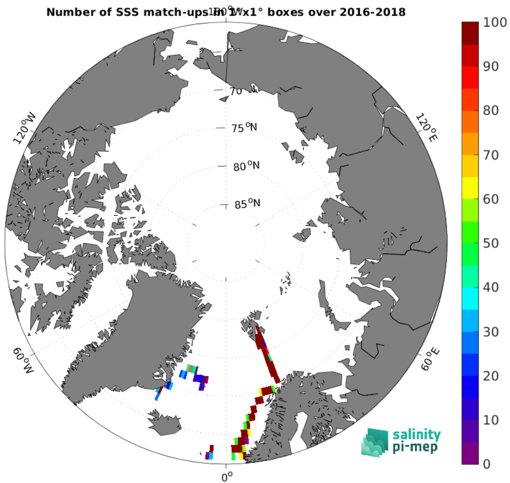
Figure 5: Number of SSS match-ups between TSG (GOSUD-Research-vessel) SSS and the SMAP SSS L2 v5.0 (JPL) SSS product for the Arctic Ocean Pi-MEP region over 1^\circ \times 1^\circ boxes and for the full satellite product period.
