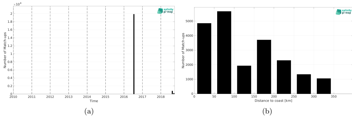
Figure 2: Number of match-ups between TSG (GOSUD-Research-vessel) and SMAP SSS L2 v5.0 (JPL) SSS as a function of time (a) and as function of the distance to coast (b) over the Arctic Ocean Pi-MEP region and for the full satellite product period.
