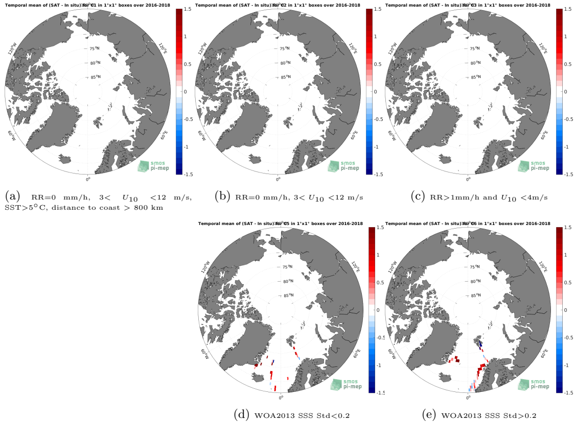
Figure 12: Temporal mean gridded over spatial boxes of size 1^\circ \times 1^\circ of \Delta SSS (SMAP SSS L2 v5.0 (JPL) - TSG (GOSUD-Research-vessel)) for 5 different subdatasets corresponding to:RR=0 mm/h, 3 < U_{10} < 12 m/s, SST>5°C, distance to coast > 800 km (a), RR=0 mm/h, 3 < U_{10} < 12 m/s (b), RR>1mm/h and U_{10} < 4 m/s (c), WOA2013 SSS Std<0.2 (d), WOA2013 SSS Std>0.2 (e).
