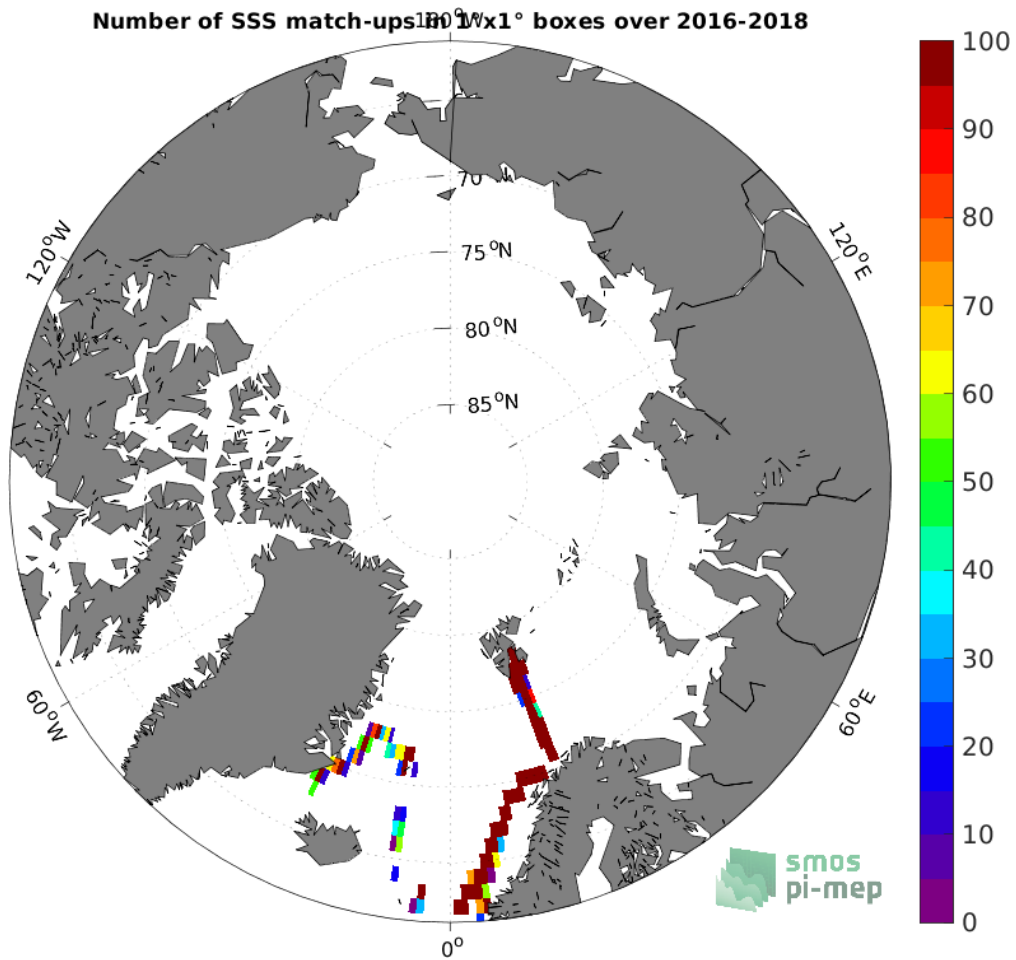
Figure 4: Number of SSS match-ups between TSG (GOSUD-Research-vessel) SSS and the SMAP SSS L2 v5.0 (JPL) SSS product for the Arctic Ocean Pi-MEP region over 1^{\circ} \times 1^{\circ} boxes and for the full satellite product period.
