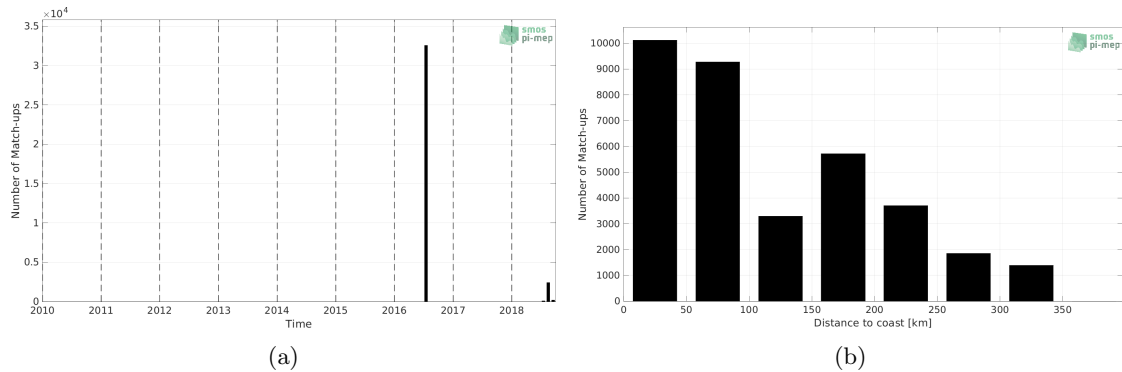
Figure 1: Number of match-ups between TSG (GOSUD-Research-vessel) and SMAP SSS L2 v5.0 (JPL) SSS as a function of time (a) and as function of the distance to coast (b) over the Arctic Ocean Pi-MEP region and for the full satellite product period.
