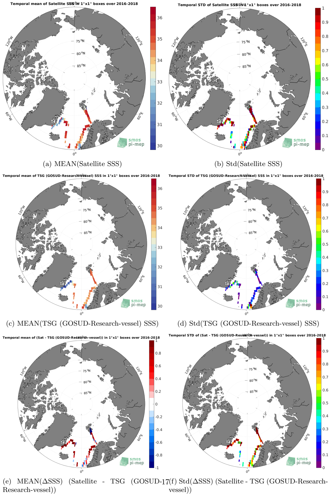
Figure 6: Temporal mean (left) and Std (right) of SSS from SMAP SSS L2 v5.0 (JPL) (top), TSG (GOSUD-Research-vessel) (middle), and of \Delta SSS (Satellite - TSG (GOSUD-Research-vessel)). Only match-up pairs are used to generate these maps.
