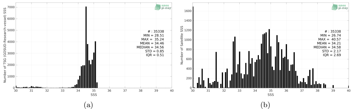
Figure 2: Histograms of SSS from TSG (GOSUD-Research-vessel) (a) and SMAP SSS L2 v5.0 (JPL) (b) considering all match-up pairs per bins of 0.1 over the Arctic Ocean Pi-MEP region and for the full satellite product period.
