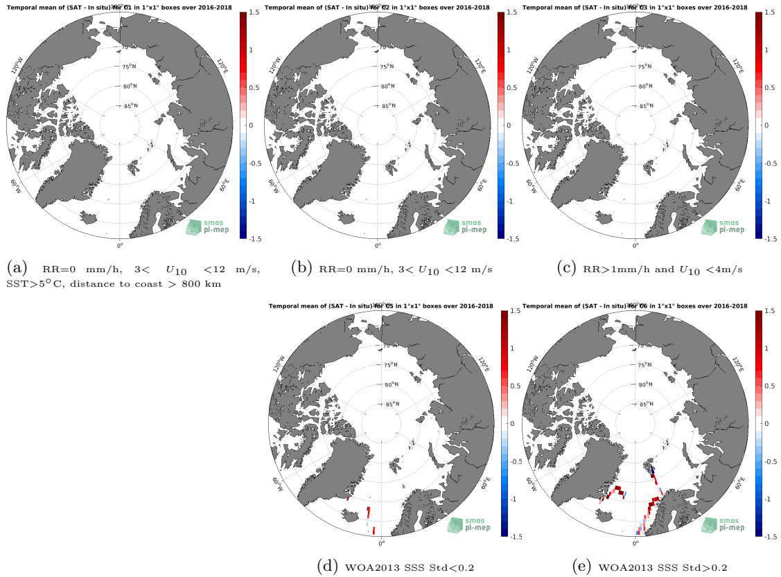
Figure 12: Temporal mean gridded over spatial boxes of size 1°x1° of \Delta SSS (SMAP SSS L2 v5.0 (JPL) - TSG (GOSUD-Research-vessel)) for 5 different subdatasets corresponding to: RR=0 mm/h, 3 < U_{10} < 12 m/s, SST > 5°C, distance to coast > 800 km (a), RR=0 mm/h, 3 < U_{10} < 12 m/s (b), RR > 1mm/h and U_{10} < 4 m/s (c), WOA2013 SSS Std < 0.2 (d), WOA2013 SSS Std > 0.2 (e).
