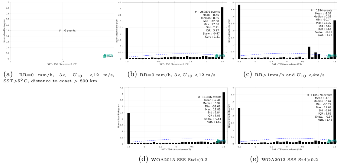
Figure 15: Normalized histogram of \Delta SSS (SMAP SSS L2 v5.0 (JPL) - TSG (Amundsen)) for 5 different subdatasets corresponding to: RR=0 mm/h, 3 < U_{10} < 12 m/s, SST>5°C, distance to coast > 800 km (a), RR=0 mm/h, 3 < U_{10} < 12 m/s (b), RR>1mm/h and U_{10} < 4 m/s (c), WOA2013 SSS Std<0.2 (d), WOA2013 SSS Std>0.2 (e).
