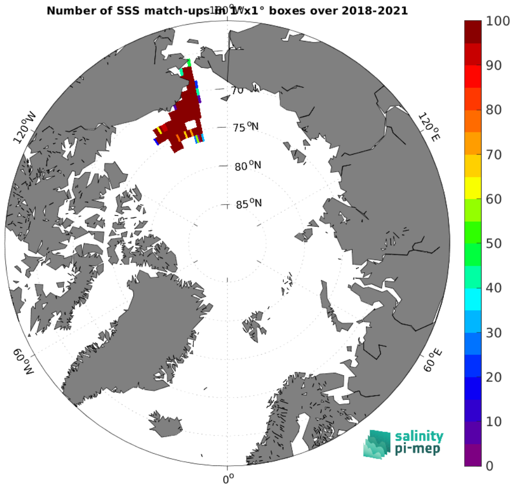
Figure 5: Number of SSS match-ups between Saildrone SSS and the SMAP SSS L2 v5.0 (JPL) SSS product for the Arctic Ocean Pi-MEP region over 1^\circ \times 1^\circ boxes and for the full satellite product period.
