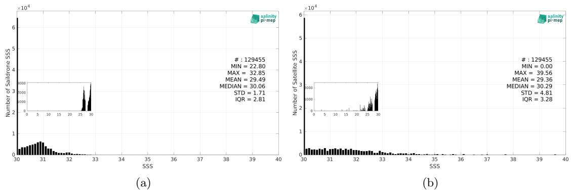
Figure 3: Histograms of SSS from Sairdronne (a) and SMAP SSS L2 v5.0 (JPL) (b) considering all match-up pairs per bins of 0.1 over the Arctic Ocean Pi-MEP region and for the full satellite product period.
