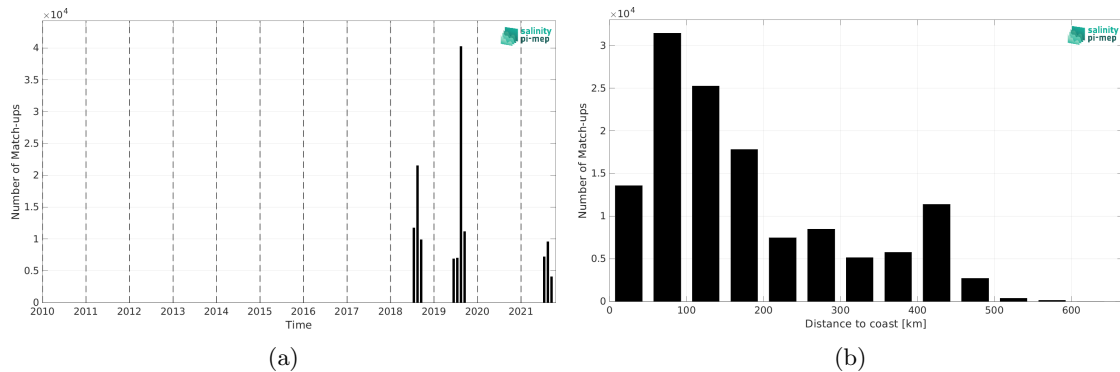
Figure 2: Number of match-ups between Sairdronne and SMAP SSS L2 v5.0 (JPL) SSS as a function of time (a) and as function of the distance to coast (b) over the Arctic Ocean Pi-MEP region and for the full satellite product period.
