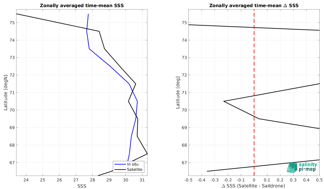
Figure 9: Left panel: Zonal mean SSS from SMAP SSS L2 v5.0 (JPL) satellite product (black) and from Saildrone (blue). Right panel: Zonal mean of \Delta SSS (Satellite - Saildrone) for all the collected Pi-MEP match-up pairs estimated over the full satellite product period.
