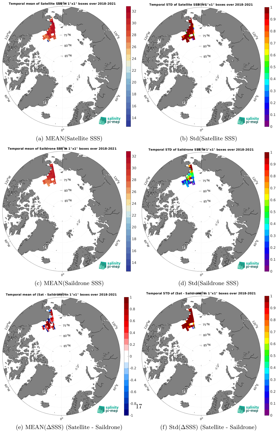
Figure 7: Temporal mean (left) and Std (right) of SSS from SMAP SSS L2 v5.0 (JPL) (top), Saildrone (middle), and of \Delta SSS (Satellite - Saildrone). Only match-up pairs are used to generate these maps.
