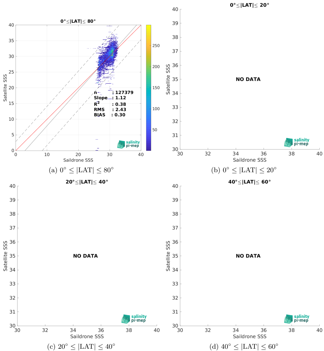
Figure 10: Contour maps of the concentration of SMAP SSS L2 v5.0 (JPL) SSS (y-axis) versus Saildrone SSS (x-axis) at match-up pairs for different latitude bands. For each plot, the red line shows x=y . The black thin and dashed lines indicate a linear fit through the data cloud and the \pm 95\% confidence levels, respectively. The number match-up pairs n , the slope and R^2 coefficient of the linear fit, the root mean square (RMS) and the mean bias between satellite and in situ data are indicated for each latitude band in each plots.
