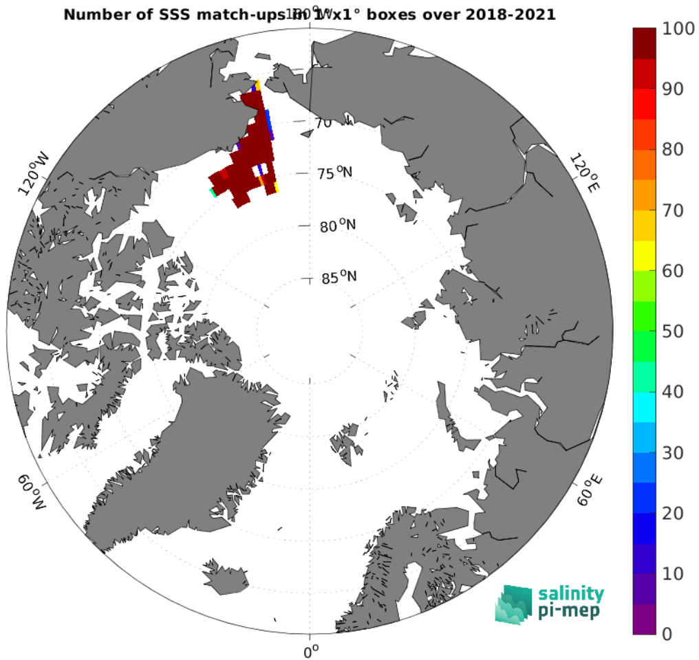
Figure 4: Number of SSS match-ups between Saildrone SSS and the SMAP SSS L2 v5.0 (JPL) SSS product for the Arctic Ocean Pi-MEP region over 1^\circ \times 1^\circ boxes and for the full satellite product period.
