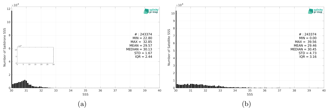
Figure 2: Histograms of SSS from Sairdrone (a) and SMAP SSS L2 v5.0 (JPL) (b) considering all match-up pairs per bins of 0.1 over the Arctic Ocean Pi-MEP region and for the full satellite product period.
