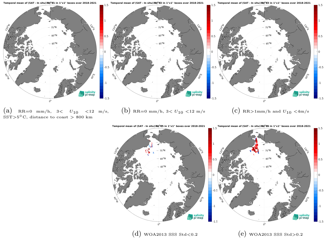
Figure 12: Temporal mean gridded over spatial boxes of size 1^{\circ}\times 1^{\circ} of \Delta\text{SSS} (SMAP SSS L2 v5.0 (JPL) - Saikrone) for 5 different subdatasets corresponding to:RR=0 mm/h, 3 < U_{10} < 12 m/s, SST >5^{\circ}\text{C} , distance to coast > 800 km (a), RR=0 mm/h, 3 < U_{10} < 12 m/s (b), RR >1 mm/h and U_{10} < 4 m/s (c), WOA2013 SSS Std <0.2 (d), WOA2013 SSS Std >0.2 (e).
