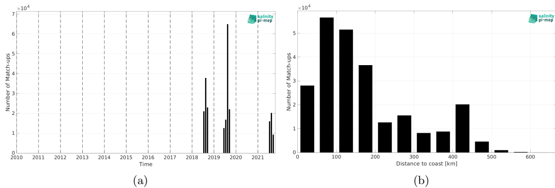
Figure 1: Number of match-ups between Sairdrone and SMAP SSS L2 v5.0 (JPL) SSS as a function of time (a) and as function of the distance to coast (b) over the Arctic Ocean Pi-MEP region and for the full satellite product period.
