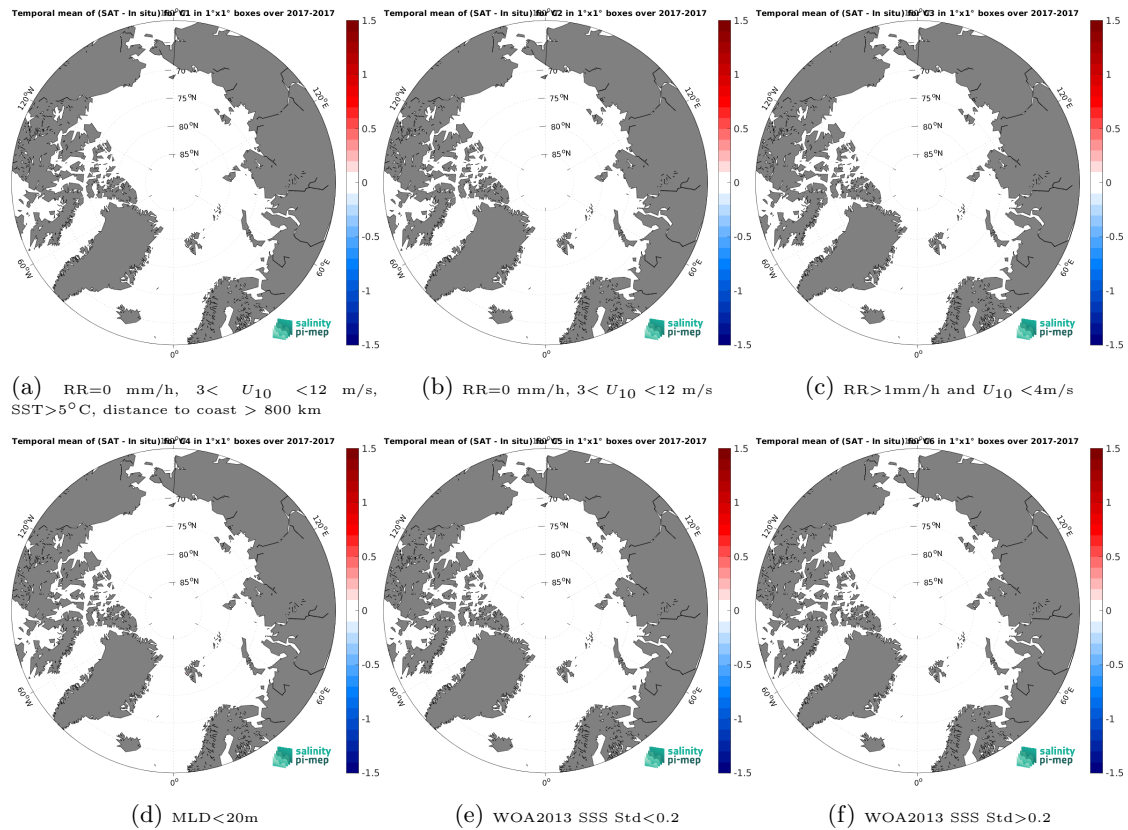
Figure 14: Temporal mean gridded over spatial boxes of size 1^\circ \times 1^\circ of \Delta\text{SSS} (SMAP SSS L2 v5.0 (JPL) - Marine mammals) for 6 different subdatasets corresponding to:RR=0 mm/h, 3 < U_{10} < 12 m/s, SST>5°C, distance to coast > 800 km (a), RR=0 mm/h, 3 < U_{10} < 12 m/s (b), RR>1mm/h and U_{10} < 4 m/s (c),MLD<20m (d),WOA2013 SSS Std<0.2 (e),WOA2013 SSS Std>0.2 (f).
