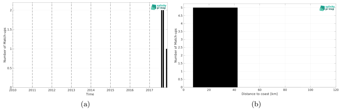
Figure 2: Number of match-ups between Marine mammals and SMAP SSS L2 v5.0 (JPL) SSS as a function of time (a) and as function of the distance to coast (b) over the Arctic Ocean Pi-MEP region and for the full satellite product period.
