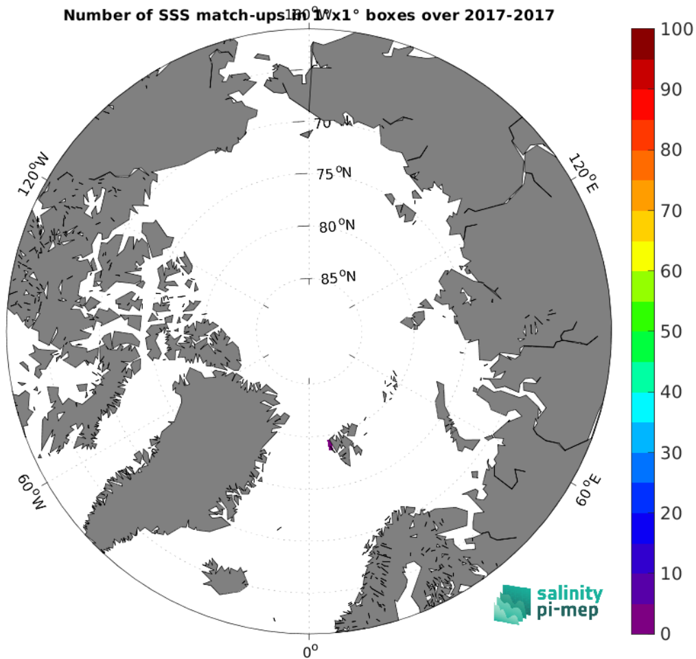
Figure 5: Number of SSS match-ups between Marine mammals SSS and the SMAP SSS L2 v5.0 (JPL) SSS product for the Arctic Ocean Pi-MEP region over 1^\circ \times 1^\circ boxes and for the full satellite product period.
