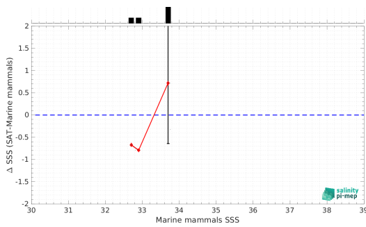
(a) Marine mammals SSS
