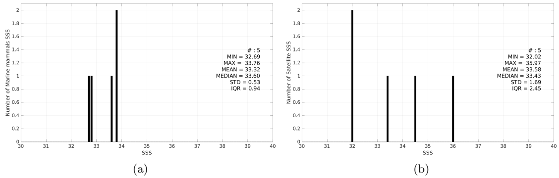
Figure 3: Histograms of SSS from Marine mammals (a) and SMAP SSS L2 v5.0 (JPL) (b) considering all match-up pairs per bins of 0.1 over the Arctic Ocean Pi-MEP region and for the full satellite product period.
