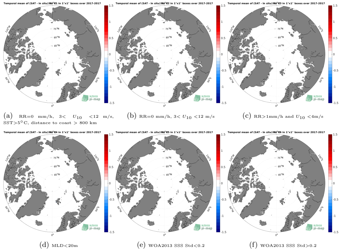
Figure 12: Temporal mean gridded over spatial boxes of size 1^{\circ}\times 1^{\circ} of \Delta\text{SSS} (SMAP SSS L2 v5.0 (JPL) - Marine mammals) for 6 different subdatasets corresponding to:RR=0 mm/h, 3 < U_{10} < 12 m/s, SST > 5^{\circ}\text{C} , distance to coast > 800 km (a), RR=0 mm/h, 3 < U_{10} < 12 m/s (b), RR > 1\text{mm/h} and U_{10} < 4\text{m/s} (c),MLD < 20\text{m} (d),WOA2013 SSS Std < 0.2 (e),WOA2013 SSS Std > 0.2 (f).
