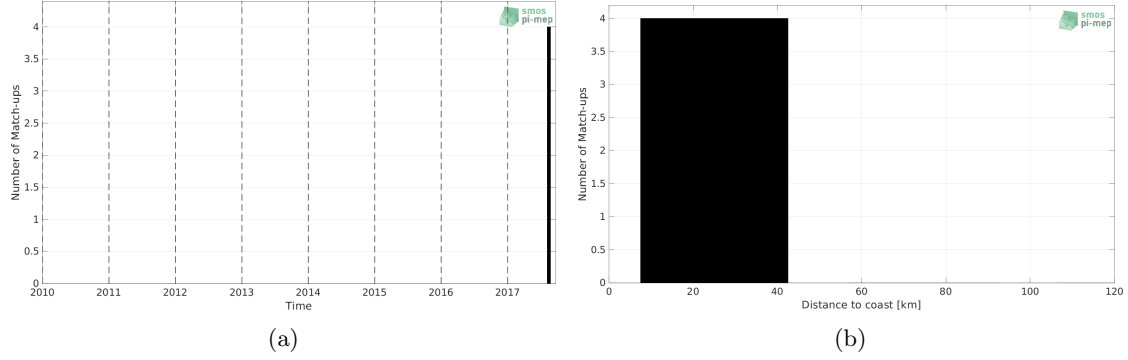
Figure 1: Number of match-ups between Marine mammals and SMAP SSS L2 v5.0 (JPL) SSS as a function of time (a) and as function of the distance to coast (b) over the Arctic Ocean Pi-MEP region and for the full satellite product period.
