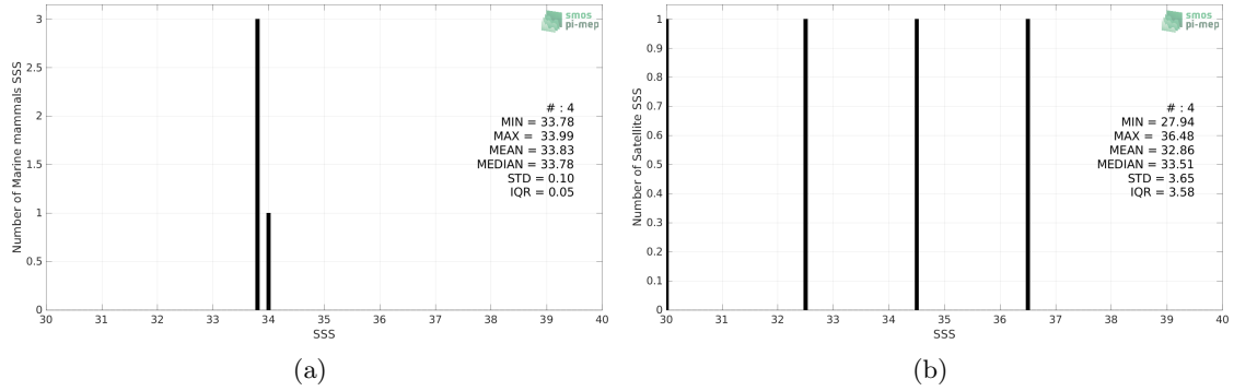
Figure 2: Histograms of SSS from Marine mammals (a) and SMAP SSS L2 v5.0 (JPL) (b) considering all match-up pairs per bins of 0.1 over the Arctic Ocean Pi-MEP region and for the full satellite product period.
