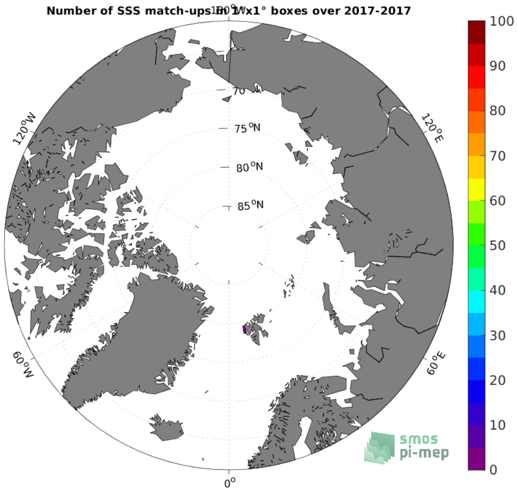
Figure 4: Number of SSS match-ups between Marine mammals SSS and the SMAP SSS L2 v5.0 (JPL) SSS product for the Arctic Ocean Pi-MEP region over 1^{\circ} \times 1^{\circ} boxes and for the full satellite product period.
