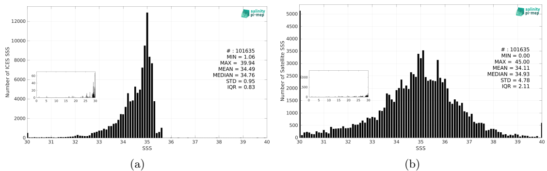
Figure 3: Histograms of SSS from ICES (a) and SMAP SSS L2 v5.0 (JPL) (b) considering all match-up pairs per bins of 0.1 over the Arctic Ocean Pi-MEP region and for the full satellite product period.
