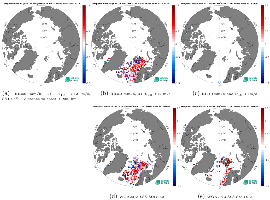
Figure 14: Temporal mean gridded over spatial boxes of size 1^\circ \times 1^\circ of \Delta SSS (SMAP SSS L2 v5.0 (JPL) - ICES) for 5 different subdatasets corresponding to:RR=0 mm/h, 3 < U_{10} < 12 m/s, SST>5°C, distance to coast > 800 km (a), RR=0 mm/h, 3 < U_{10} < 12 m/s (b), RR>1mm/h and U_{10} < 4 m/s (c), WOA2013 SSS Std<0.2 (d), WOA2013 SSS Std>0.2 (e).
