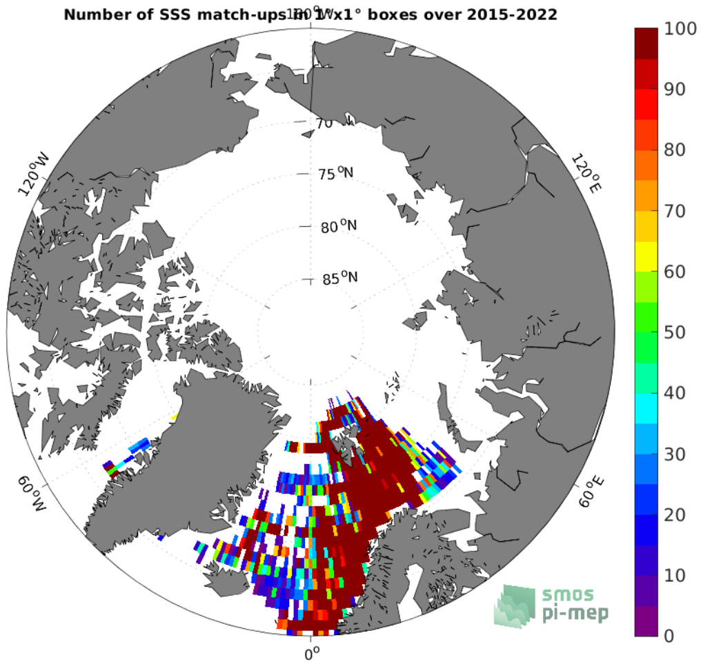
Figure 4: Number of SSS match-ups between ICES SSS and the SMAP SSS L2 v5.0 (JPL) SSS product for the Arctic Ocean Pi-MEP region over 1^\circ \times 1^\circ boxes and for the full satellite product period.
