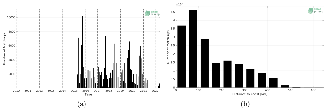
Figure 1: Number of match-ups between ICES and SMAP SSS L2 v5.0 (JPL) SSS as a function of time (a) and as function of the distance to coast (b) over the Arctic Ocean Pi-MEP region and for the full satellite product period.
