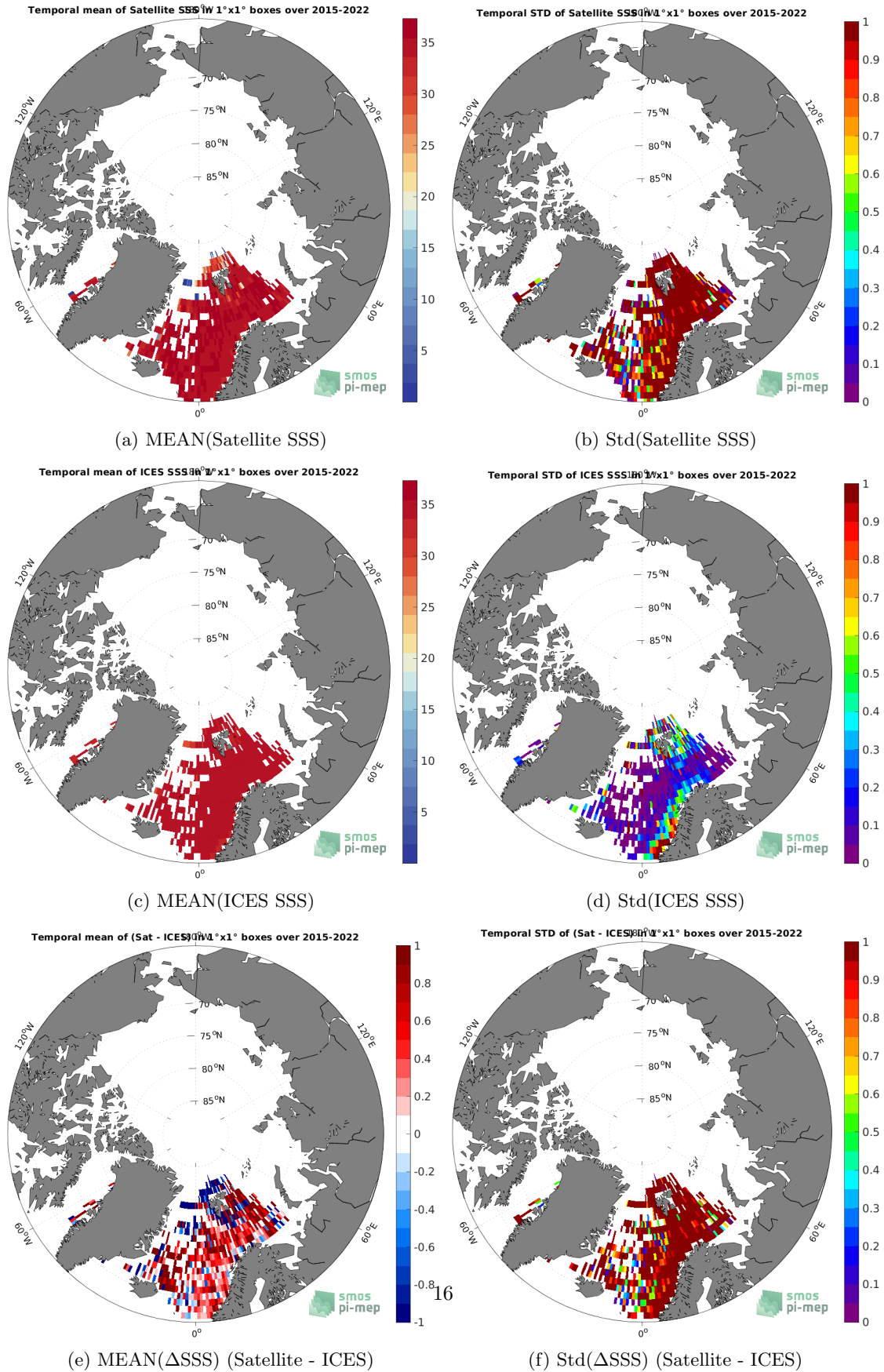
Figure 6: Temporal mean (left) and Std (right) of SSS from SMAP SSS L2 v5.0 (JPL) (top), ICES (middle), and of \Delta SSS (Satellite - ICES). Only match-up pairs are used to generate these maps.
