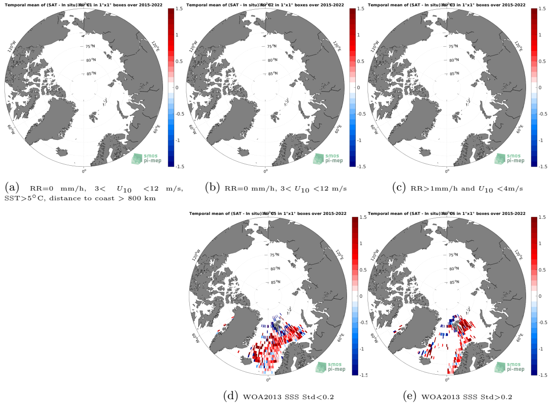
Figure 12: Temporal mean gridded over spatial boxes of size 1^{\circ}\times 1^{\circ} of \Delta\text{SSS} (SMAP SSS L2 v5.0 (JPL) - ICES) for 5 different subdatasets corresponding to:RR=0 mm/h, 3 < U_{10} < 12 m/s, SST >5^{\circ}\text{C} , distance to coast > 800 km (a), RR=0 mm/h, 3 < U_{10} < 12 m/s (b), RR >1 mm/h and U_{10} < 4 m/s (c), WOA2013 SSS Std <0.2 (d), WOA2013 SSS Std >0.2 (e).
