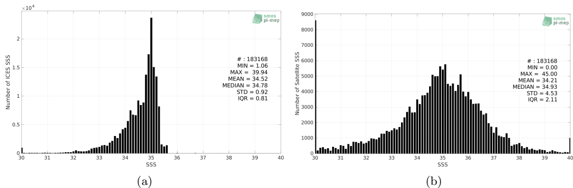
Figure 2: Histograms of SSS from ICES (a) and SMAP SSS L2 v5.0 (JPL) (b) considering all match-up pairs per bins of 0.1 over the Arctic Ocean Pi-MEP region and for the full satellite product period.
