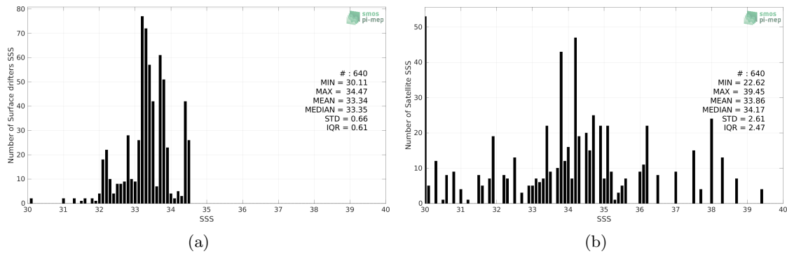
Figure 2: Histograms of SSS from Surface drifters (a) and SMAP SSS L2 v5.0 (JPL) (b) considering all match-up pairs per bins of 0.1 over the Arctic Ocean Pi-MEP region and for the full satellite product period.
