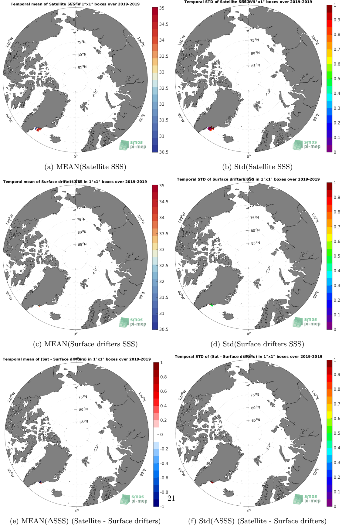
Figure 5: Temporal mean (left) and Std (right) of SSS from SMAP SSS L2 v5.0 (JPL) (top), Surface drifters (middle), and of \Delta SSS (Satellite - Surface drifters). Only match-up pairs are used to generate these maps.
