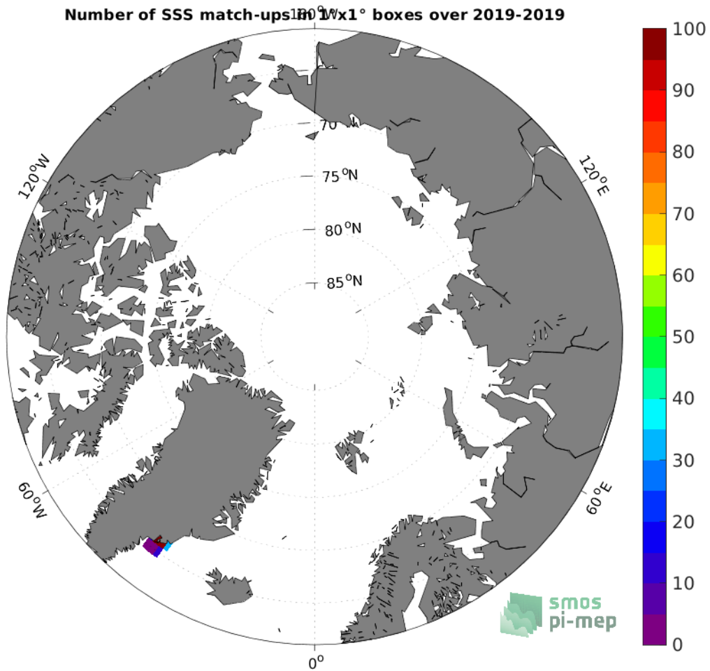
Figure 3: Number of SSS match-ups between Surface drifters SSS and the SMAP SSS L2 v5.0 (JPL) SSS product for the Arctic Ocean Pi-MEP region over 1^{\circ} \times 1^{\circ} boxes and for the full satellite product period.
