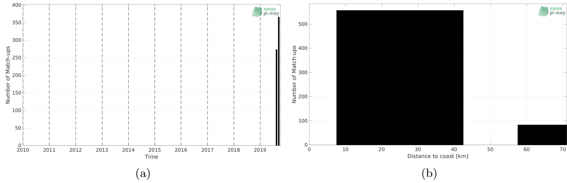
Figure 1: Number of match-ups between Surface drifters and SMAP SSS L2 v5.0 (JPL) SSS as a function of time (a) and as function of the distance to coast (b) over the Arctic Ocean Pi-MEP region and for the full satellite product period.
