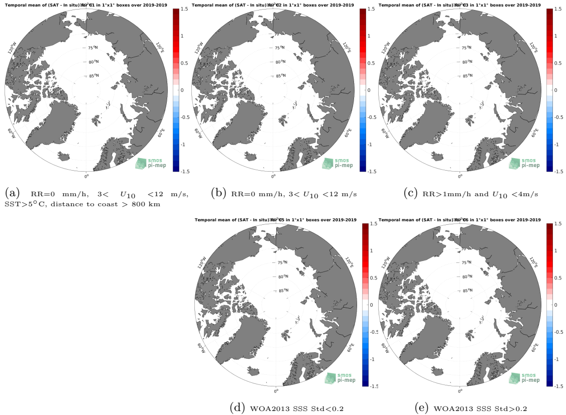
Figure 11: Temporal mean gridded over spatial boxes of size 1^{\circ}\times 1^{\circ} of \Delta\text{SSS} (SMAP SSS L2 v5.0 (JPL) - Surface drifters) for 5 different subdatasets corresponding to:RR=0 mm/h, 3 < U_{10} < 12 m/s, SST >5^{\circ}\text{C} , distance to coast > 800 km (a), RR=0 mm/h, 3 < U_{10} < 12 m/s (b), RR >1 mm/h and U_{10} < 4 m/s (c), WOA2013 SSS Std <0.2 (d), WOA2013 SSS Std >0.2 (e).
