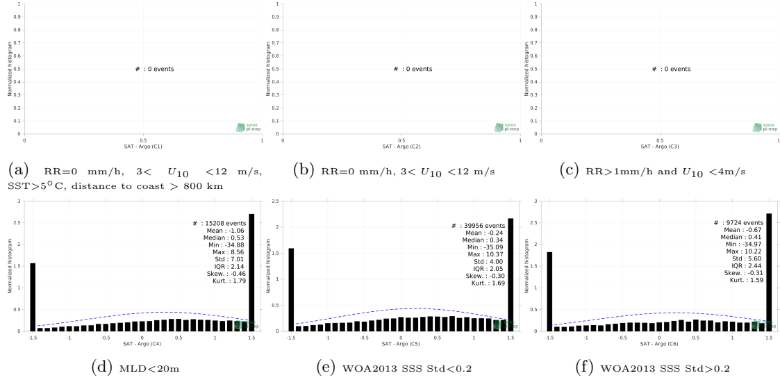
Figure 13: Normalized histogram of \Delta\text{SSS} (SMAP SSS L2 v5.0 (JPL) - Argo) for 6 different subdatasets corresponding to: RR=0 mm/h, 3 < U_{10} < 12 m/s, SST > 5^\circ\text{C} , distance to coast > 800 km (a), RR=0 mm/h, 3 < U_{10} < 12 m/s (b), RR > 1\text{mm/h} and U_{10} < 4\text{m/s} (c), MLD < 20\text{m} (d), WOA2013 SSS Std < 0.2 (e), WOA2013 SSS Std > 0.2 (f).
