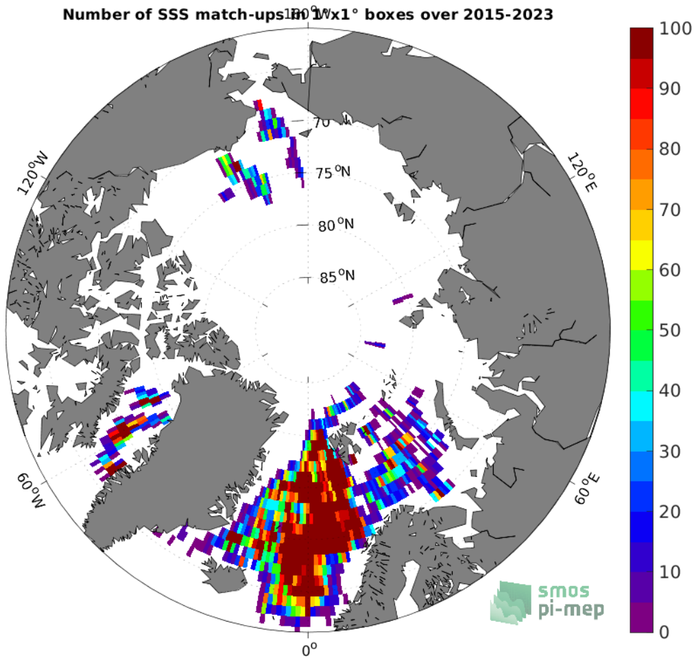
Figure 4: Number of SSS match-ups between Argo SSS and the SMAP SSS L2 v5.0 (JPL) SSS product for the Arctic Ocean Pi-MEP region over 1^{\circ} \times 1^{\circ} boxes and for the full satellite product period.
