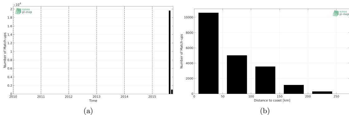
Figure 1: Number of match-ups between TSG-SAMOS and SMAP-L2-JPL-V4 SSS as a function of time (a) and as function of the distance to coast (b) over the Arctic Ocean Pi-MEP region and for the full satellite product period.
