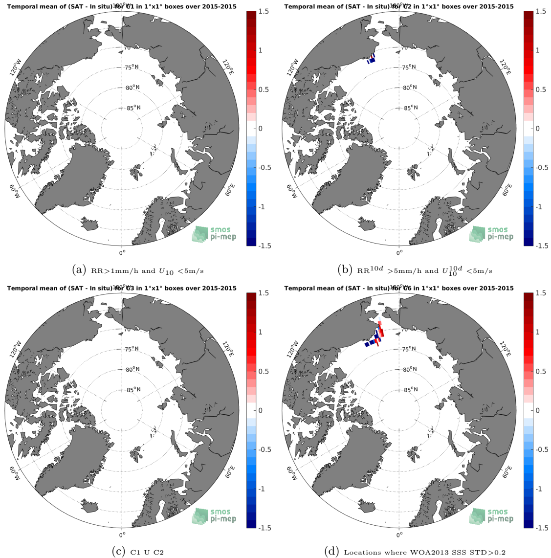
Figure 12: Temporal mean gridded over spatial boxes of size 1^\circ \times 1^\circ of \Delta SSS (SMAP-L2-JPL-V4 - TSG-SAMOS) for 4 different subdatasets corresponding to: RR > 1\text{mm/h} and U_{10} < 5\text{m/s} (a), RR^{10d} > 5\text{mm/h} and U_{10}^{10d} < 5\text{m/s} (b), C1 U C2 (c), Locations where WOA2013 SSS STD > 0.2 (d).
