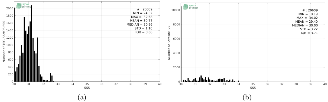
Figure 2: Histograms of SSS from TSG-SAMOS (a) and SMAP-L2-JPL-V4 (b) considering all match-up pairs per bins of 0.1 over the Arctic Ocean Pi-MEP region and for the full satellite product period.
