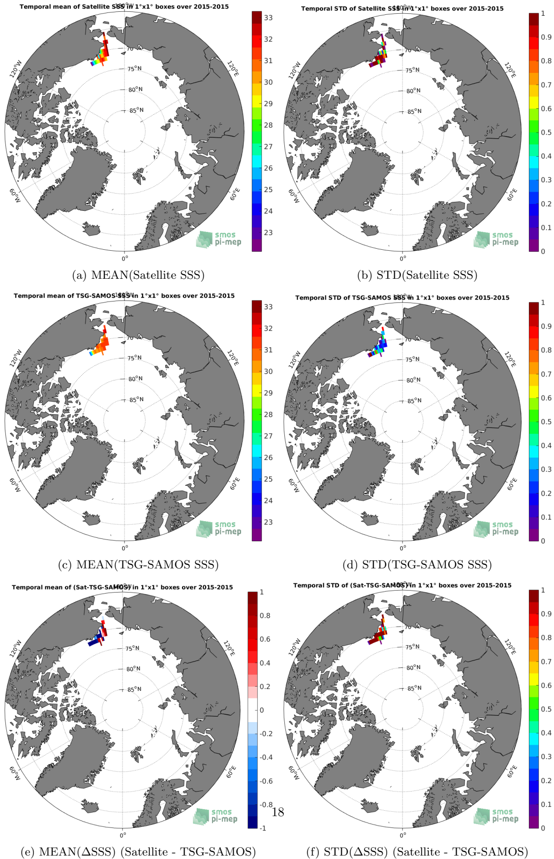
Figure 6: Temporal mean (left) and STD (right) of SSS from SMAP-L2-JPL-V4 (top), TSG-SAMOS (middle), and of \Delta SSS (Satellite - TSG-SAMOS). Only match-up pairs are used to generate these maps.
