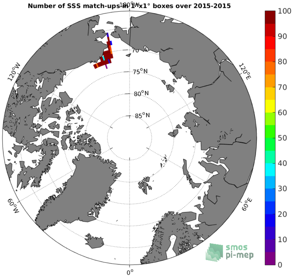
Figure 4: Number of SSS match-ups between TSG-SAMOS SSS and the SMAP-L2-JPL-V4 SSS product for the Arctic Ocean Pi-MEP region over 1^\circ \times 1^\circ boxes and for the full satellite product period.
