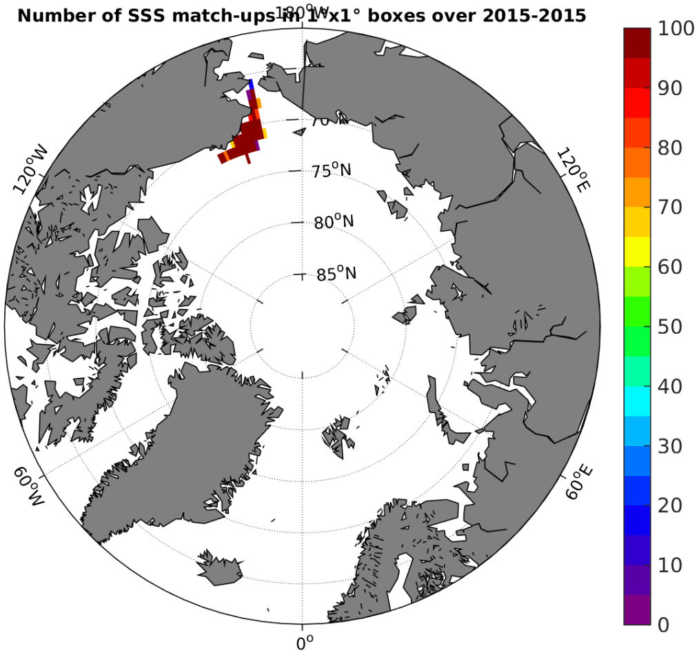
Figure 4: Number of SSS match-ups between TSG-SAMOS SSS and the SMAP-L2-JPL-V4 SSS product for the Arctic Ocean Pi-MEP region over 1°x1° boxes and for the full satellite product period.
