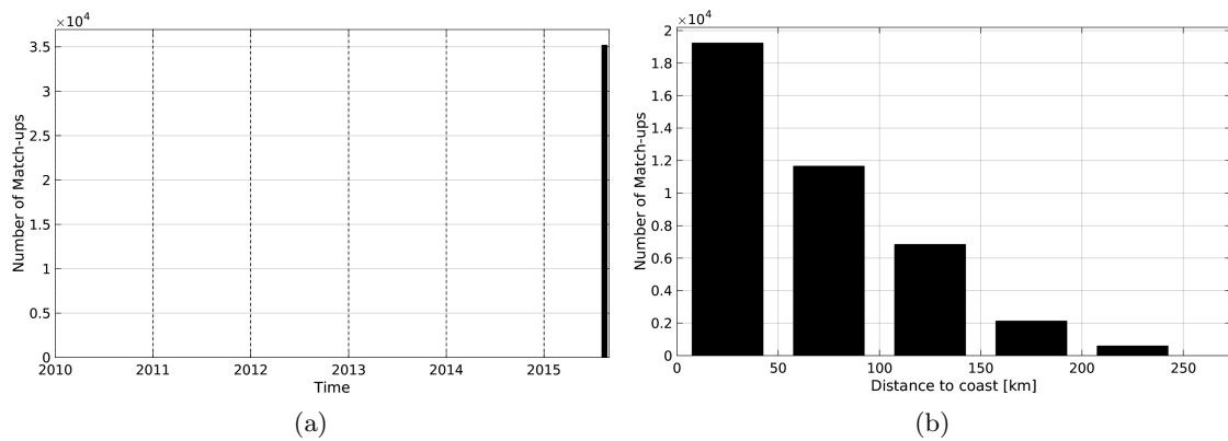
Figure 1: Number of match-ups between TSG-SAMOS and SMAP-L2-JPL-V4 SSS as a function of time (a) and as function of the distance to coast (b) over the Arctic Ocean Pi-MEP region and for the full satellite product period.
