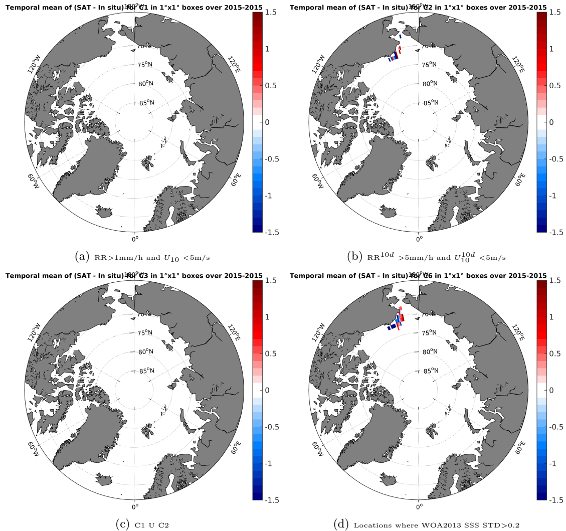
Figure 12: Temporal mean gridded over spatial boxes of size 1°x1° of \Delta SSS (SMAP-L2-JPL-V4 - TSG-SAMOS) for 4 different subdatasets corresponding to:RR>1mm/h and U_{10} < 5\text{m/s} (a), RR^{10d} > 5\text{mm/h} and U_{10}^{10d} < 5\text{m/s} (b), C1 U C2 (c),Locations where WOA2013 SSS STD>0.2 (d).
