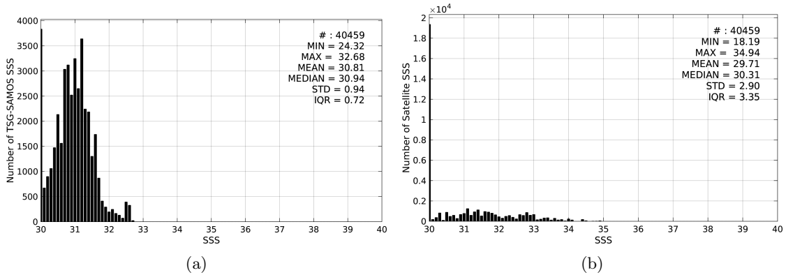
Figure 2: Histograms of SSS from TSG-SAMOS (a) and SMAP-L2-JPL-V4 (b) considering all match-up pairs per bins of 0.1 over the Arctic Ocean Pi-MEP region and for the full satellite product period.
