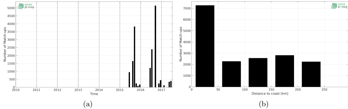
Figure 1: Number of match-ups between TSG-LEGOS-DM and SMAP-L2-JPL-V4 SSS as a function of time (a) and as function of the distance to coast (b) over the Arctic Ocean Pi-MEP region and for the full satellite product period.
