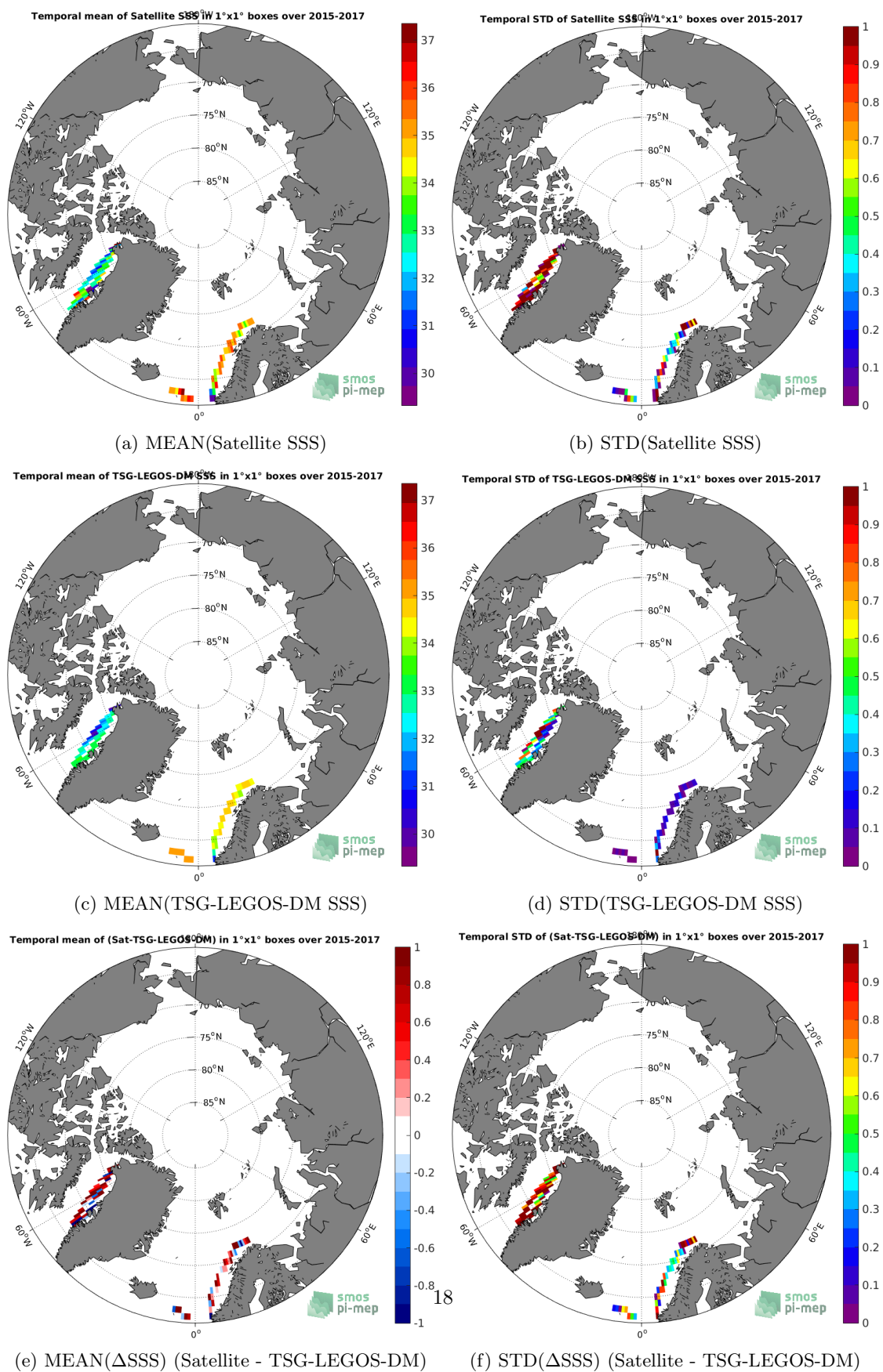
Figure 6: Temporal mean (left) and STD (right) of SSS from SMAP-L2-JPL-V4 (top), TSG-LEGOS-DM (middle), and of \Delta SSS (Satellite - TSG-LEGOS-DM). Only match-up pairs are used to generate these maps.
