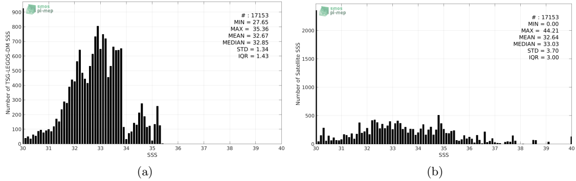
Figure 2: Histograms of SSS from TSG-LEGOS-DM (a) and SMAP-L2-JPL-V4 (b) considering all match-up pairs per bins of 0.1 over the Arctic Ocean Pi-MEP region and for the full satellite product period.
