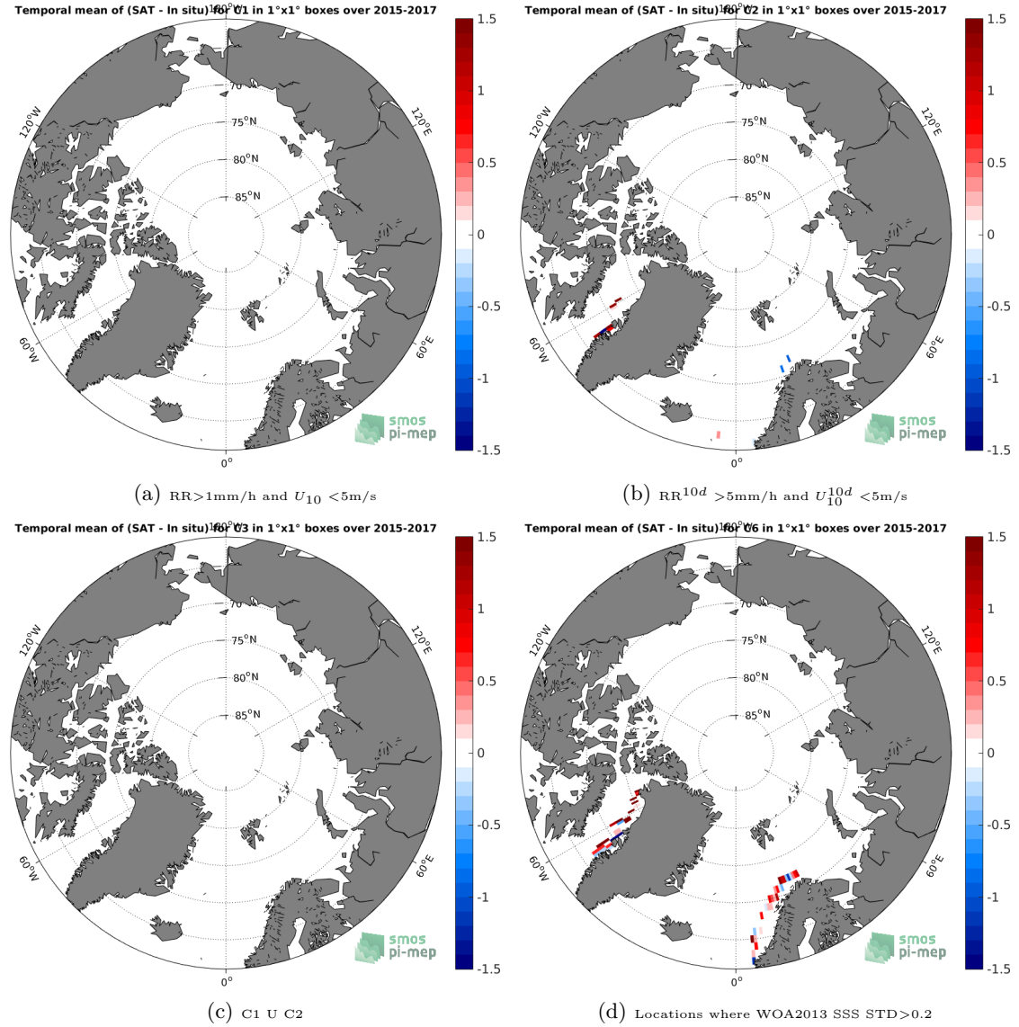
Figure 12: Temporal mean gridded over spatial boxes of size 1^\circ \times 1^\circ of \Delta SSS (SMAP-L2-JPL-V4 - TSG-LEGOS-DM) for 4 different subdatasets corresponding to: RR > 1\text{mm/h} and U_{10} < 5\text{m/s} (a), RR^{10d} > 5\text{mm/h} and U_{10}^{10d} < 5\text{m/s} (b), C1 U C2 (c), Locations where WOA2013 SSS STD > 0.2 (d).
