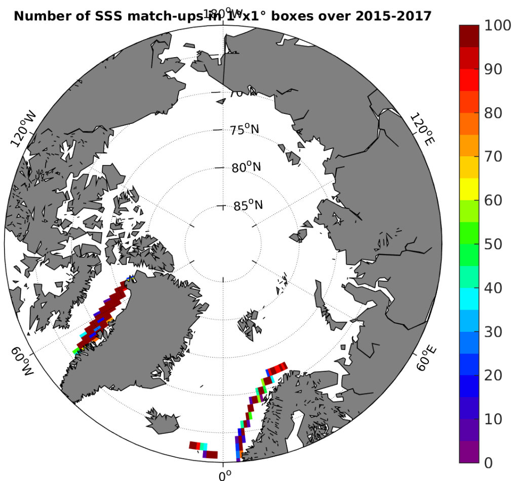
Figure 4: Number of SSS match-ups between TSG-LEGOS-DM SSS and the SMAP-L2-JPL-V4 SSS product for the Arctic Ocean Pi-MEP region over 1°x1° boxes and for the full satellite product period.
