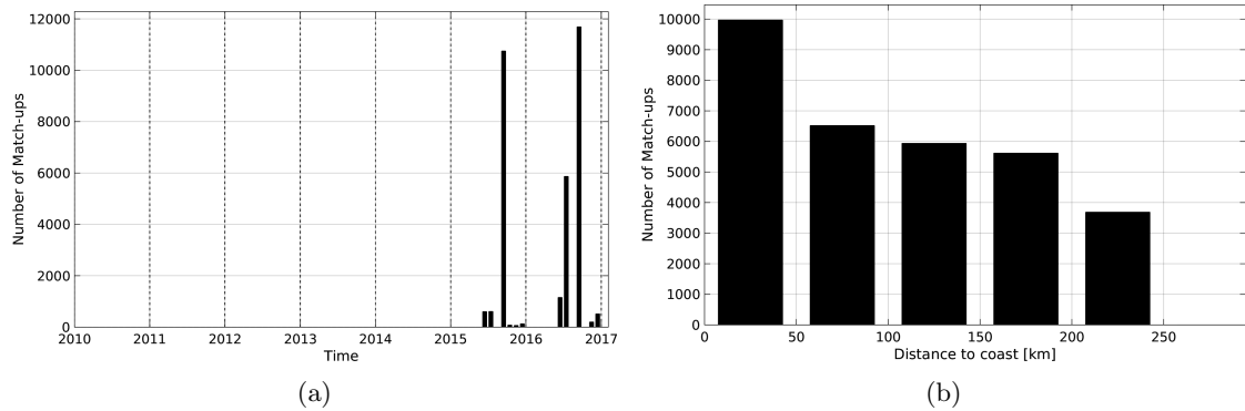
Figure 1: Number of match-ups between TSG-LEGOS-DM and SMAP-L2-JPL-V4 SSS as a function of time (a) and as function of the distance to coast (b) over the Arctic Ocean Pi-MEP region and for the full satellite product period.
