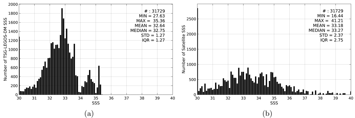
Figure 2: Histograms of SSS from TSG-LEGOS-DM (a) and SMAP-L2-JPL-V4 (b) considering all match-up pairs per bins of 0.1 over the Arctic Ocean Pi-MEP region and for the full satellite product period.
