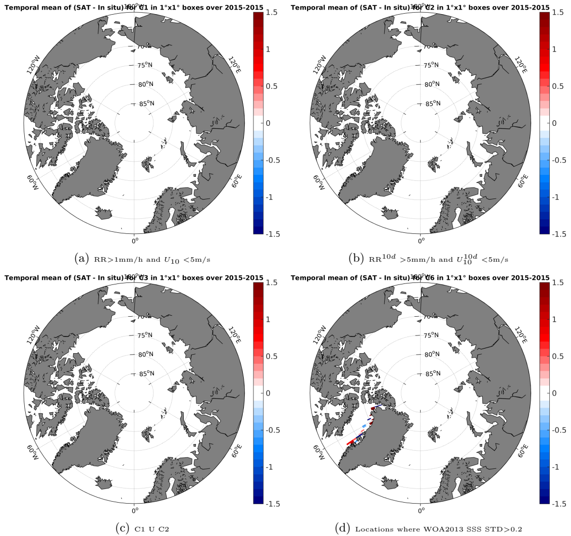
Figure 12: Temporal mean gridded over spatial boxes of size 1^\circ \times 1^\circ of \Delta SSS (SMAP-L2-JPL-V4 - TSG-GOSUD-Sailing-ship) for 4 different subdatasets corresponding to:RR >1 mm/h and U_{10} < 5 m/s (a), RR^{10d} > 5 mm/h and U_{10}^{10d} < 5 m/s (b), C1 U C2 (c), Locations where WOA2013 SSS STD >0.2 (d).
