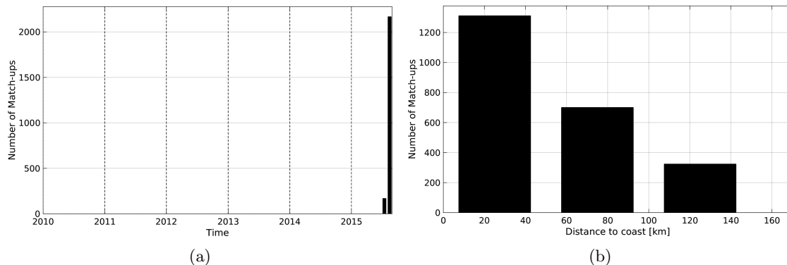
Figure 1: Number of match-ups between TSG-GOSUD-Sailing-ship and SMAP-L2-JPL-V4 SSS as a function of time (a) and as function of the distance to coast (b) over the Arctic Ocean Pi-MEP region and for the full satellite product period.
