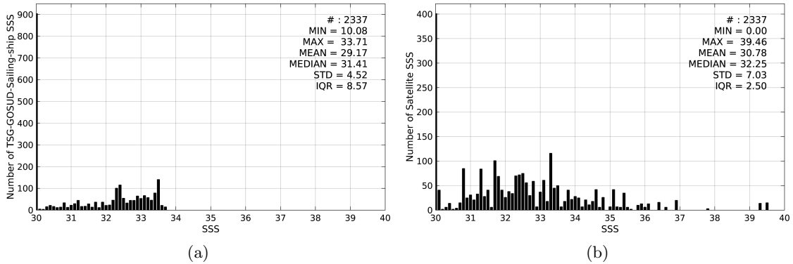
Figure 2: Histograms of SSS from TSG-GOSUD-Sailing-ship (a) and SMAP-L2-JPL-V4 (b) considering all match-up pairs per bins of 0.1 over the Arctic Ocean Pi-MEP region and for the full satellite product period.
