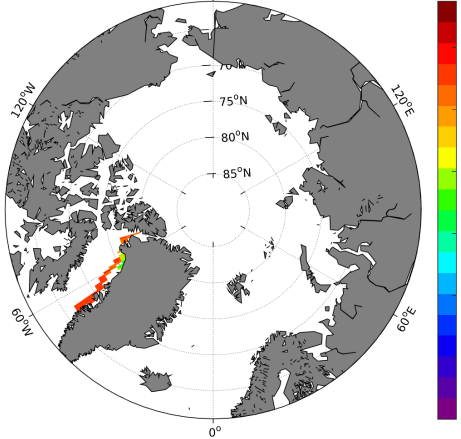
(c) MEAN(TSG-GOSUD-Sailing-ship SSS)
