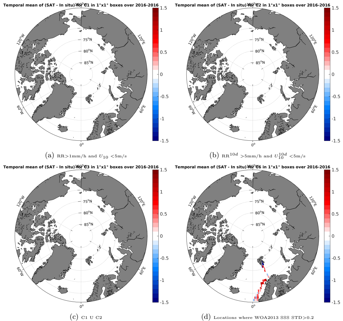
Figure 12: Temporal mean gridded over spatial boxes of size 1^\circ \times 1^\circ of \Delta SSS (SMAP-L2-JPL-V4 - TSG-GOSUD-Research-vessel) for 4 different subdatasets corresponding to:RR >1 mm/h and U_{10} < 5 m/s (a), RR^{10d} > 5 mm/h and U_{10}^{10d} < 5 m/s (b), C1 U C2 (c),Locations where WOA2013 SSS STD >0.2 (d).
