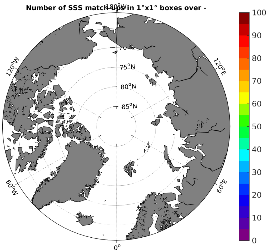
Figure 4: Number of SSS match-ups between Sea mammals SSS and the SMAP-L2-JPL-V4 SSS product for the Arctic Ocean Pi-MEP region over 1°x1° boxes and for the full satellite product period.
