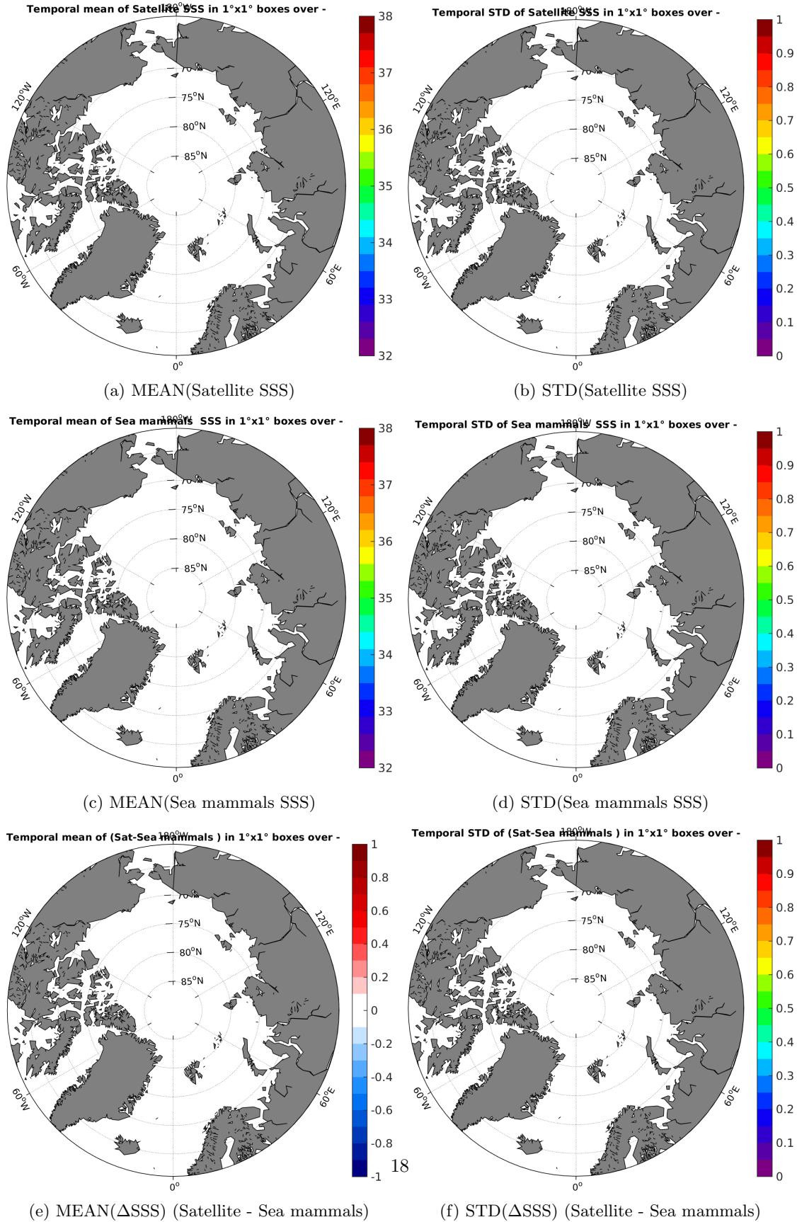
Figure 6: Temporal mean (left) and STD (right) of SSS from SMAP-L2-JPL-V4 (top), Sea mammals (middle), and of \Delta SSS (Satellite - Sea mammals). Only match-up pairs are used to generate these maps.
