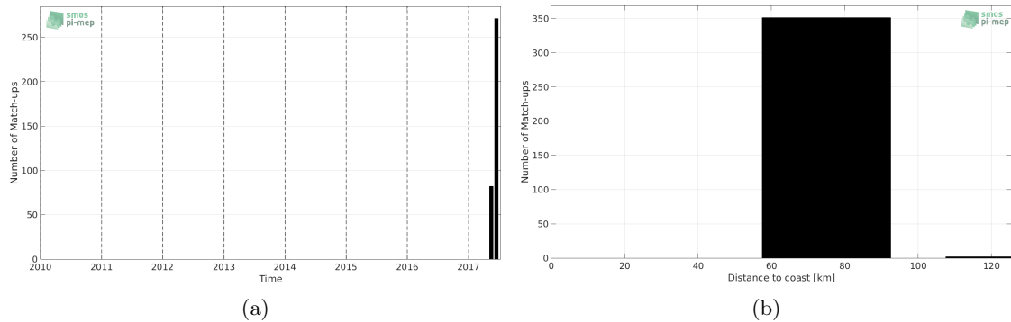
Figure 1: Number of match-ups between Surface drifters and SMAP-L2-JPL-V4 SSS as a function of time (a) and as function of the distance to coast (b) over the Arctic Ocean Pi-MEP region and for the full satellite product period.
