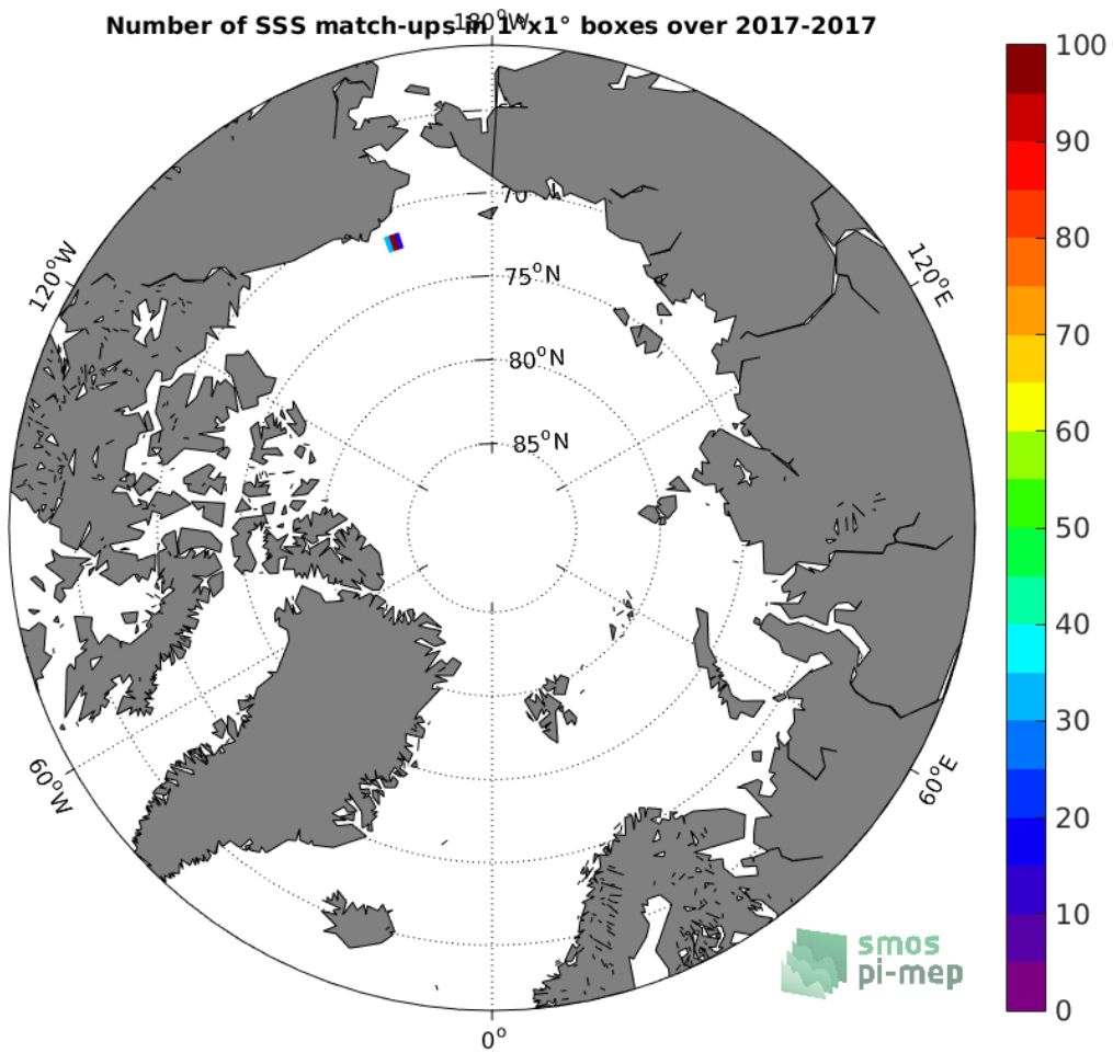
Figure 3: Number of SSS match-ups between Surface drifters SSS and the SMAP-L2-JPL-V4 SSS product for the Arctic Ocean Pi-MEP region over 1^\circ \times 1^\circ boxes and for the full satellite product period.
