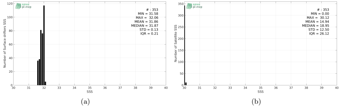
Figure 2: Histograms of SSS from Surface drifters (a) and SMAP-L2-JPL-V4 (b) considering all match-up pairs per bins of 0.1 over the Arctic Ocean Pi-MEP region and for the full satellite product period.
