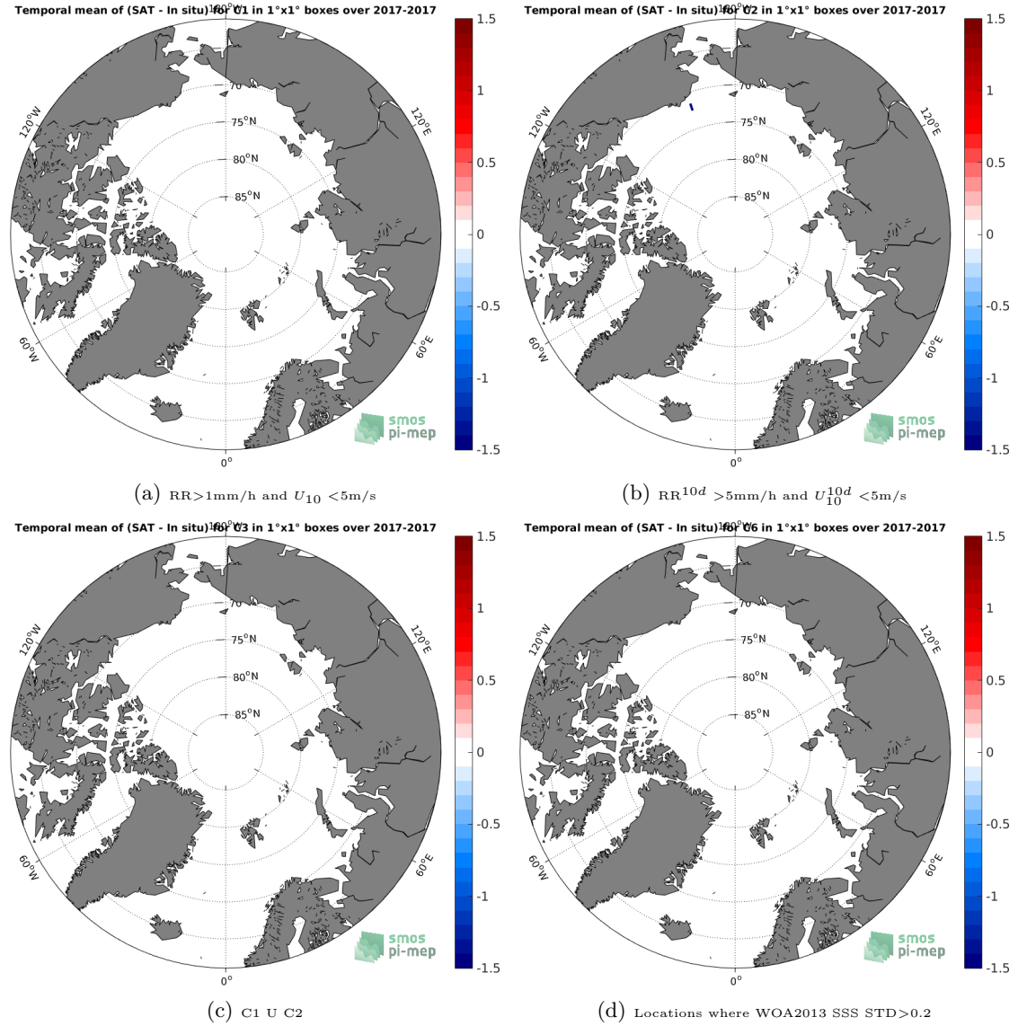
Figure 11: Temporal mean gridded over spatial boxes of size 1^\circ \times 1^\circ of \Delta SSS (SMAP-L2-JPL-V4 - Surface drifters) for 4 different subdatasets corresponding to: RR > 1\text{mm/h} and U_{10} < 5\text{m/s} (a), RR^{10d} > 5\text{mm/h} and U_{10}^{10d} < 5\text{m/s} (b), C1 U C2 (c), Locations where WOA2013 SSS STD > 0.2 (d).
