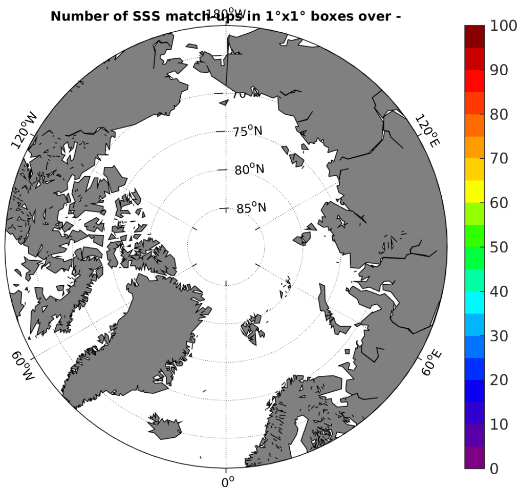
Figure 3: Number of SSS match-ups between Surface drifters SSS and the SMAP-L2-JPL-V4 SSS product for the Arctic Ocean Pi-MEP region over 1°x1° boxes and for the full satellite product period.
