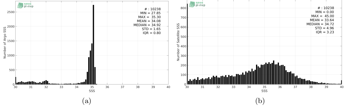
Figure 2: Histograms of SSS from Argo (a) and SMAP-L2-JPL-V4 (b) considering all match-up pairs per bins of 0.1 over the Arctic Ocean Pi-MEP region and for the full satellite product period.
