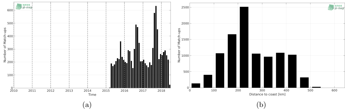
Figure 1: Number of match-ups between Argo and SMAP-L2-JPL-V4 SSS as a function of time (a) and as function of the distance to coast (b) over the Arctic Ocean Pi-MEP region and for the full satellite product period.
