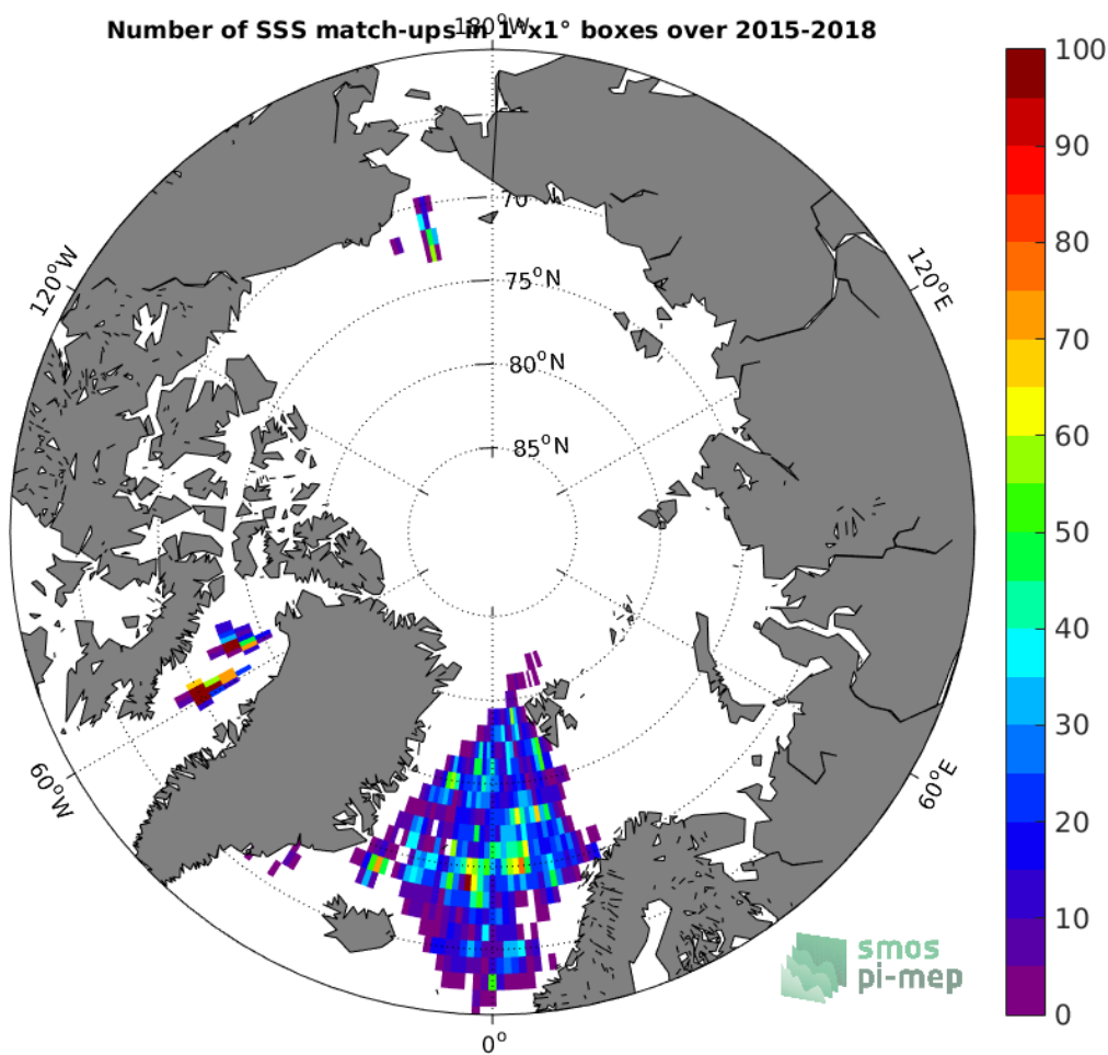
Figure 4: Number of SSS match-ups between Argo SSS and the SMAP-L2-JPL-V4 SSS product for the Arctic Ocean Pi-MEP region over 1^\circ \times 1^\circ boxes and for the full satellite product period.
