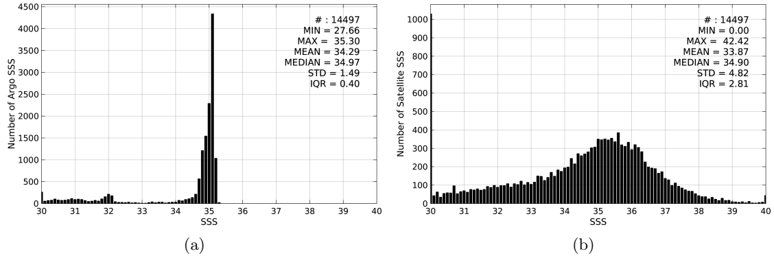
Figure 2: Histograms of SSS from Argo (a) and SMAP-L2-JPL-V4 (b) considering all match-up pairs per bins of 0.1 over the Arctic Ocean Pi-MEP region and for the full satellite product period.
