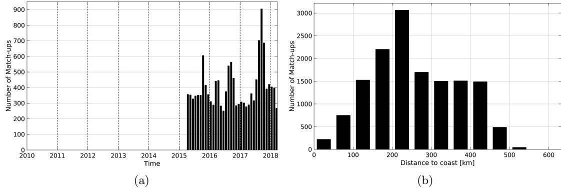
Figure 1: Number of match-ups between Argo and SMAP-L2-JPL-V4 SSS as a function of time (a) and as function of the distance to coast (b) over the Arctic Ocean Pi-MEP region and for the full satellite product period.
