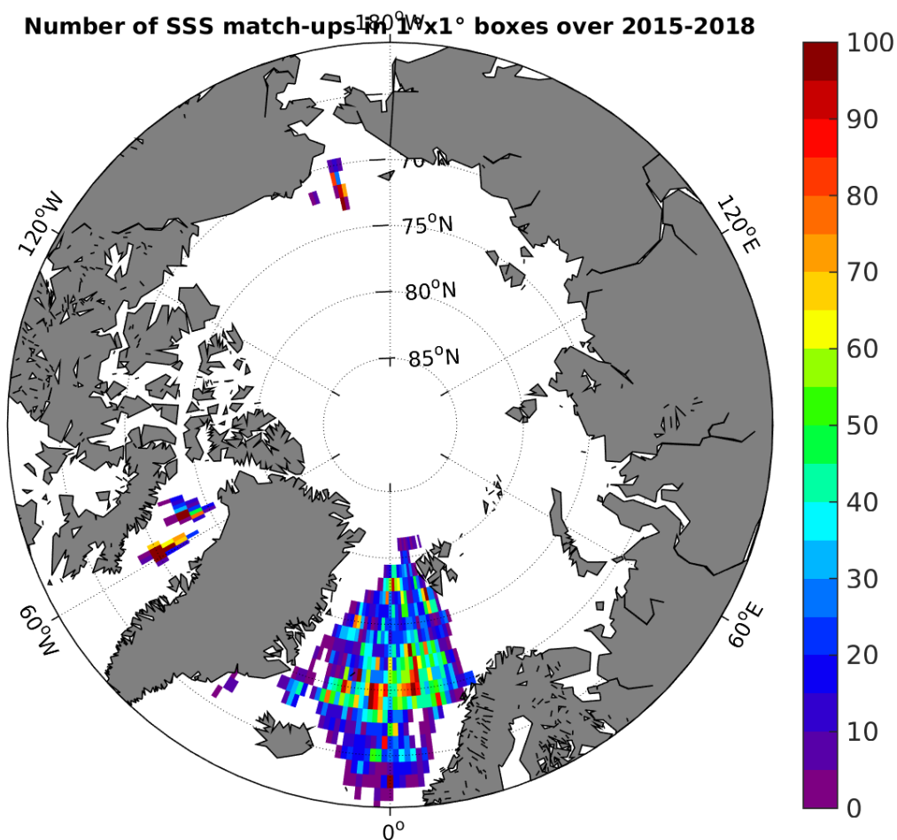
Figure 4: Number of SSS match-ups between Argo SSS and the SMAP-L2-JPL-V4 SSS product for the Arctic Ocean Pi-MEP region over 1°x1° boxes and for the full satellite product period.
