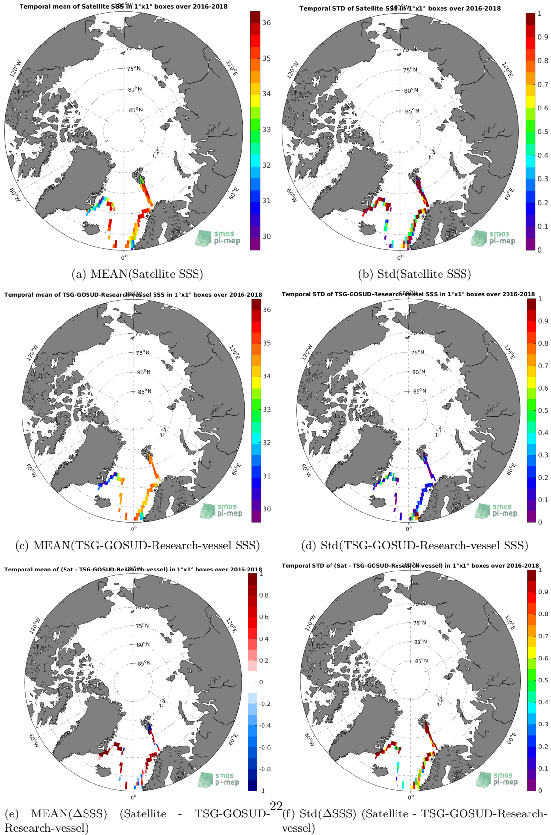
Figure 6: Temporal mean (left) and Std (right) of SSS from SMAP-L2-JPL-V4.3 (top), TSG-GOSUD-Research-vessel (middle), and of \Delta SSS (Satellite - TSG-GOSUD-Research-vessel). Only match-up pairs are used to generate these maps.
