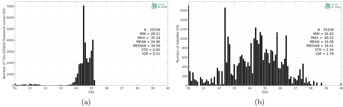
Figure 2: Histograms of SSS from TSG-GOSUD-Research-vessel (a) and SMAP-L2-JPL-V4.3 (b) considering all match-up pairs per bins of 0.1 over the Arctic Ocean Pi-MEP region and for the full satellite product period.
