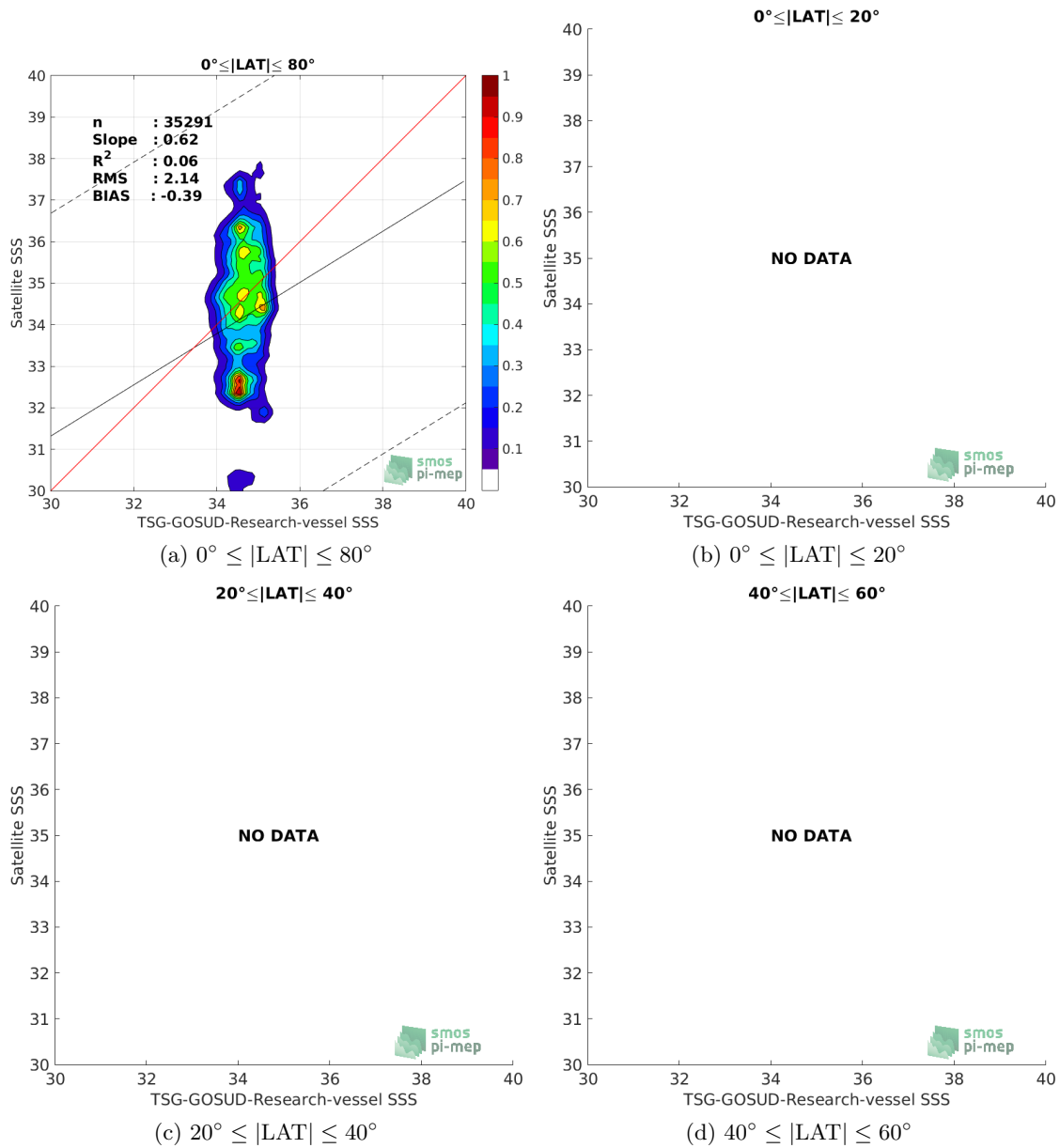
Figure 9: Contour maps of the concentration of SMAP-L2-JPL-V4.3 SSS (y-axis) versus TSG-GOSUD-Research-vessel SSS (x-axis) at match-up pairs for different latitude bands. For each plot, the red line shows x=y . The black thin and dashed lines indicate a linear fit through the data cloud and the \pm 95\% confidence levels, respectively. The number match-up pairs n , the slope and R^2 coefficient of the linear fit, the root mean square (RMS) and the mean bias between satellite and in situ data are indicated for each latitude band in each plots.
