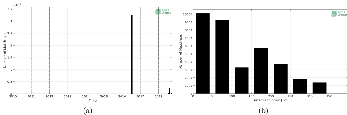
Figure 1: Number of match-ups between TSG-GOSUD-Research-vessel and SMAP-L2-JPL-V4.3 SSS as a function of time (a) and as function of the distance to coast (b) over the Arctic Ocean Pi-MEP region and for the full satellite product period.
