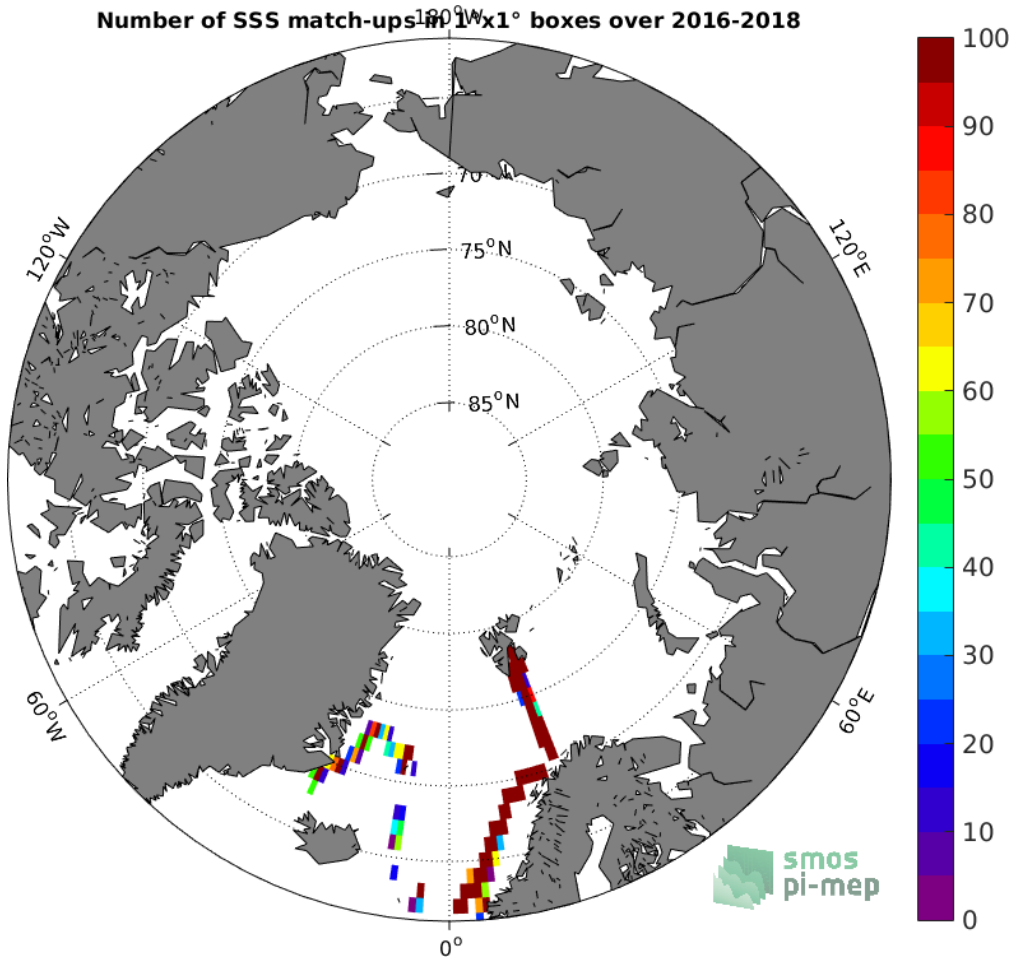
Figure 4: Number of SSS match-ups between TSG-GOSUD-Research-vessel SSS and the SMAP-L2-JPL-V4.3 SSS product for the Arctic Ocean Pi-MEP region over 1°x1° boxes and for the full satellite product period.
