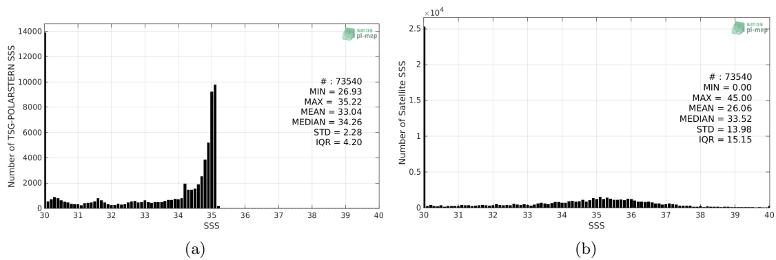
Figure 2: Histograms of SSS from TSG-POLARSTERN (a) and SMAP-L2-JPL-V4.2 (b) considering all match-up pairs per bins of 0.1 over the Arctic Ocean Pi-MEP region and for the full satellite product period.
