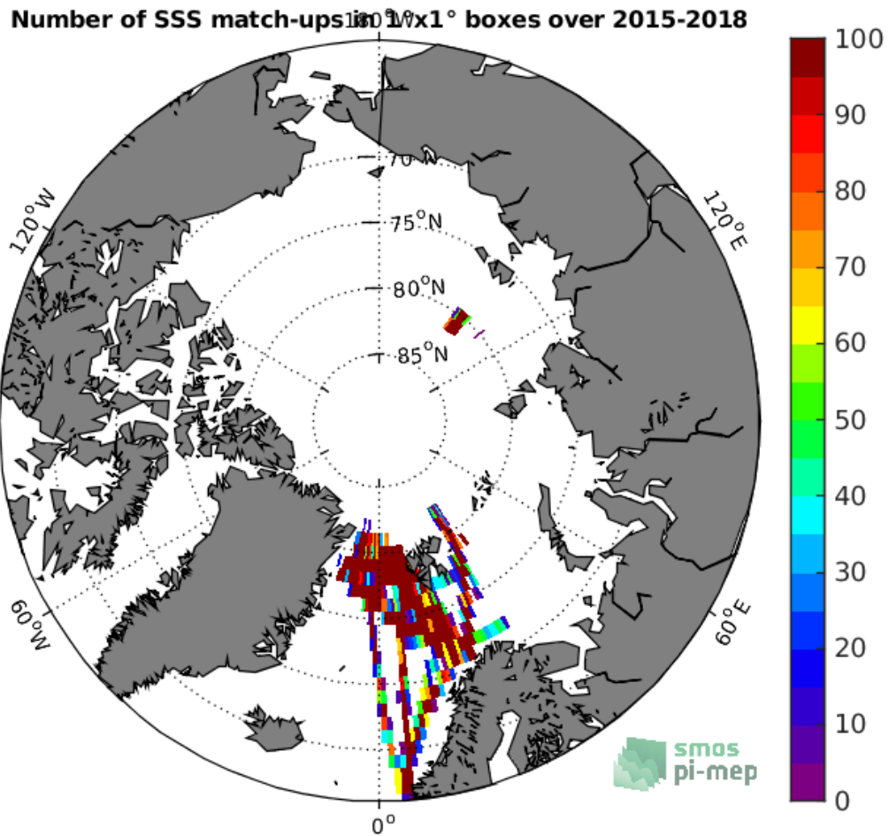
Figure 4: Number of SSS match-ups between TSG-POLARSTERN SSS and the SMAP-L2-JPL-V4.2 SSS product for the Arctic Ocean Pi-MEP region over 1°x1° boxes and for the full satellite product period.
