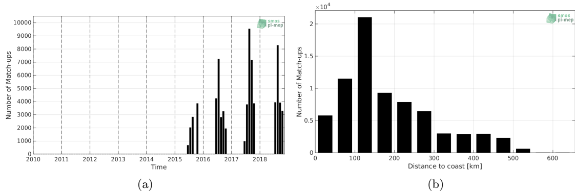
Figure 1: Number of match-ups between TSG-POLARSTERN and SMAP-L2-JPL-V4.2 SSS as a function of time (a) and as function of the distance to coast (b) over the Arctic Ocean Pi-MEP region and for the full satellite product period.
