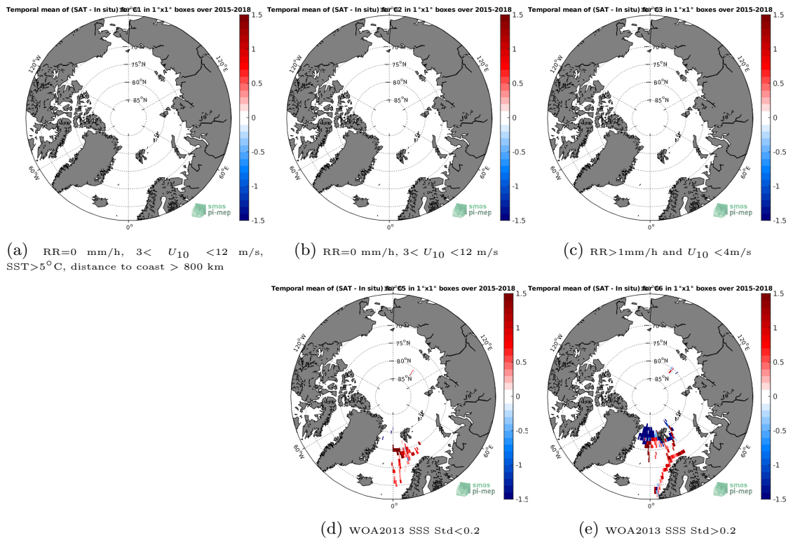
Figure 12: Temporal mean gridded over spatial boxes of size 1^\circ \times 1^\circ of \Delta SSS (SMAP-L2-JPL-V4.2 - TSG-POLARSTERN) for 5 different subdatasets corresponding to:RR=0 mm/h, 3 < U_{10} < 12 m/s, SST >5^\circ C, distance to coast > 800 km (a), RR=0 mm/h, 3 < U_{10} < 12 m/s (b), RR >1 mm/h and U_{10} < 4 m/s (c), WOA2013 SSS Std <0.2 (d), WOA2013 SSS Std >0.2 (e).
