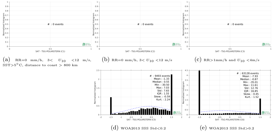
Figure 13: Normalized histogram of \Delta\text{SSS} (SMAP-L2-JPL-V4.2 - TSG-POLARSTERN) for 5 different subdatasets corresponding to: RR=0 mm/h, 3 < U_{10} < 12 m/s, SST >5^{\circ}\text{C} , distance to coast > 800 km (a), RR=0 mm/h, 3 < U_{10} < 12 m/s (b), RR >1 mm/h and U_{10} < 4 m/s (c), WOA2013 SSS Std <0.2 (d), WOA2013 SSS Std >0.2 (e).
