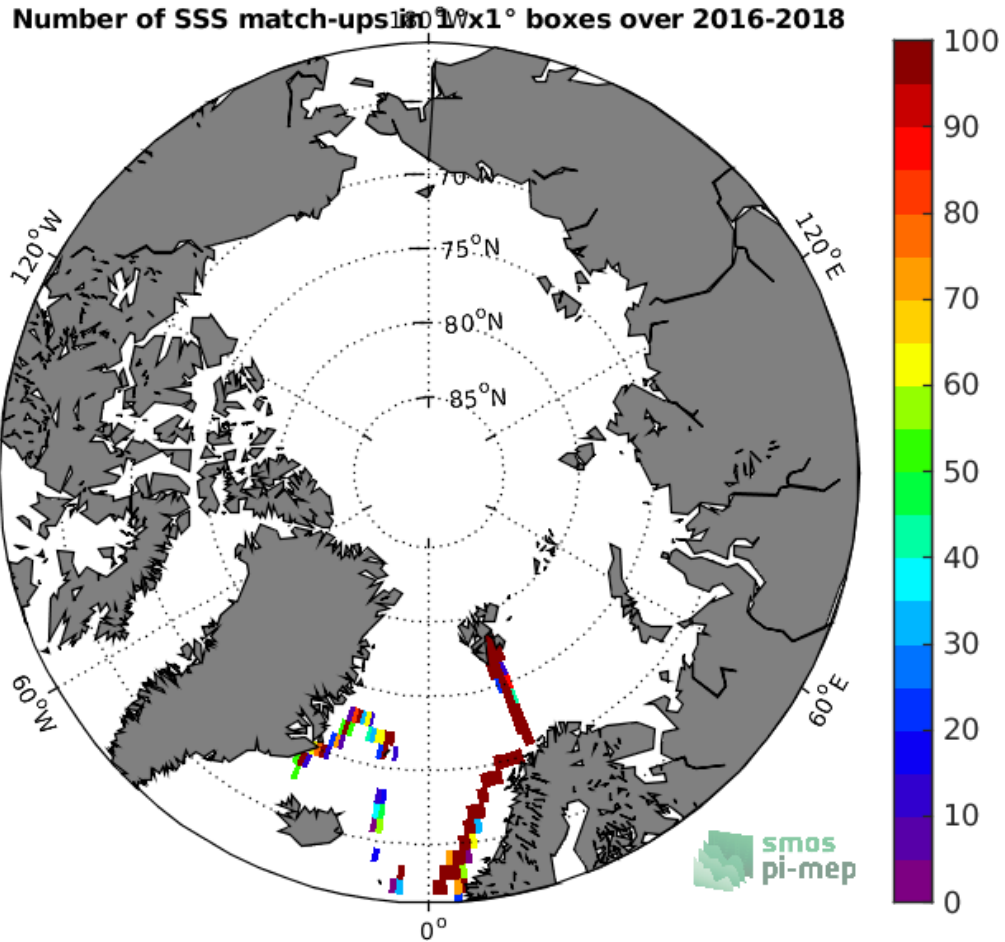
Figure 4: Number of SSS match-ups between TSG-GOSUD-Research-vessel SSS and the SMAP-L2-JPL-V4.2 SSS product for the Arctic Ocean Pi-MEP region over 1°x1° boxes and for the full satellite product period.
