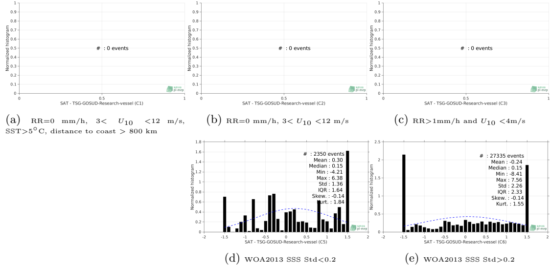
Figure 13: Normalized histogram of \Delta SSS (SMAP-L2-JPL-V4.2 - TSG-GOSUD-Research-vessel) for 5 different subdatasets corresponding to: RR=0 mm/h, 3 < U_{10} < 12 m/s, SST > 5°C, distance to coast > 800 km (a), RR=0 mm/h, 3 < U_{10} < 12 m/s (b), RR > 1mm/h and U_{10} < 4 m/s (c), WOA2013 SSS Std < 0.2 (d), WOA2013 SSS Std > 0.2 (e).
