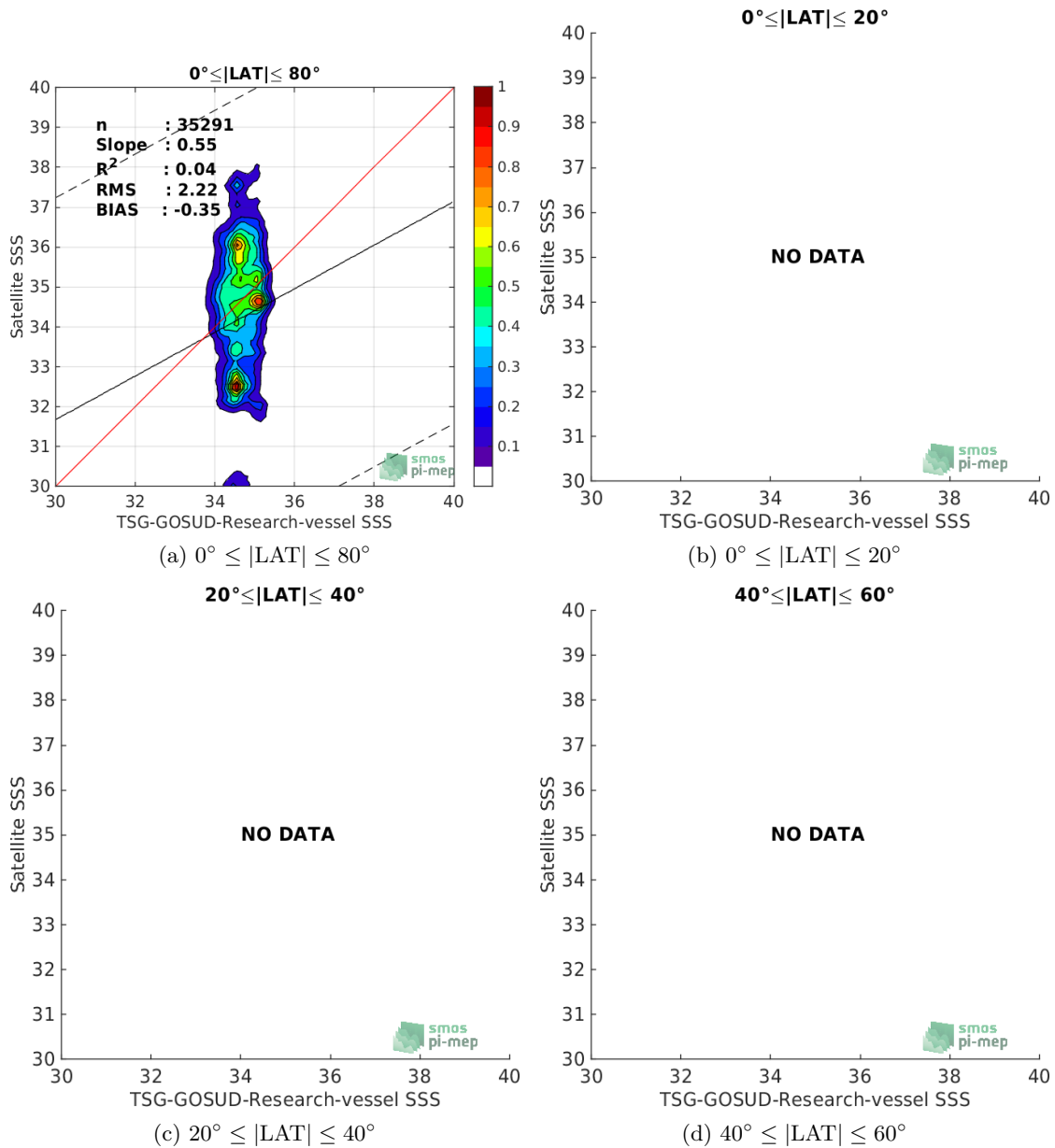
Figure 9: Contour maps of the concentration of SMAP-L2-JPL-V4.2 SSS (y-axis) versus TSG-GOSUD-Research-vessel SSS (x-axis) at match-up pairs for different latitude bands. For each plot, the red line shows x=y . The black thin and dashed lines indicate a linear fit through the data cloud and the \pm 95\% confidence levels, respectively. The number match-up pairs n , the slope and R^2 coefficient of the linear fit, the root mean square (RMS) and the mean bias between satellite and in situ data are indicated for each latitude band in each plots.
