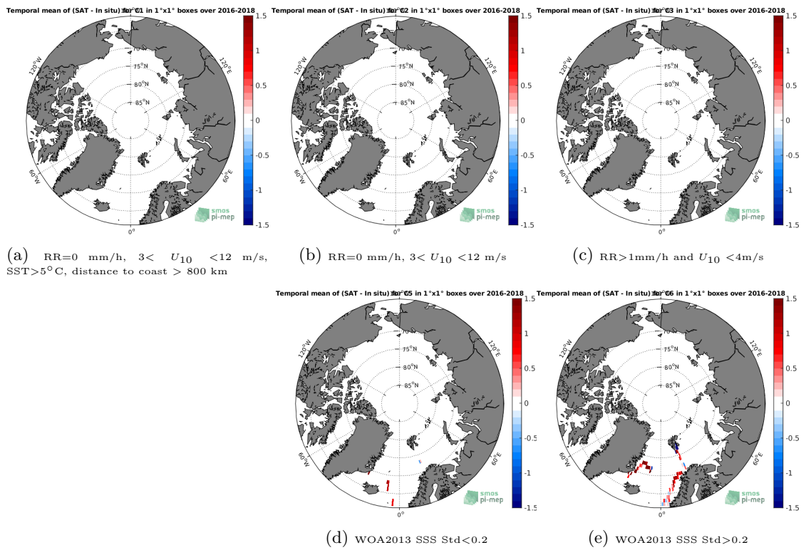
Figure 12: Temporal mean gridded over spatial boxes of size 1^\circ \times 1^\circ of \Delta SSS (SMAP-L2-JPL-V4.2 - TSG-GOSUD-Research-vessel) for 5 different subdatasets corresponding to:RR=0 mm/h, 3 < U_{10} < 12 m/s, SST>5°C, distance to coast > 800 km (a), RR=0 mm/h, 3 < U_{10} < 12 m/s (b), RR>1mm/h and U_{10} < 4 m/s (c), WOA2013 SSS Std<0.2 (d), WOA2013 SSS Std>0.2 (e).
