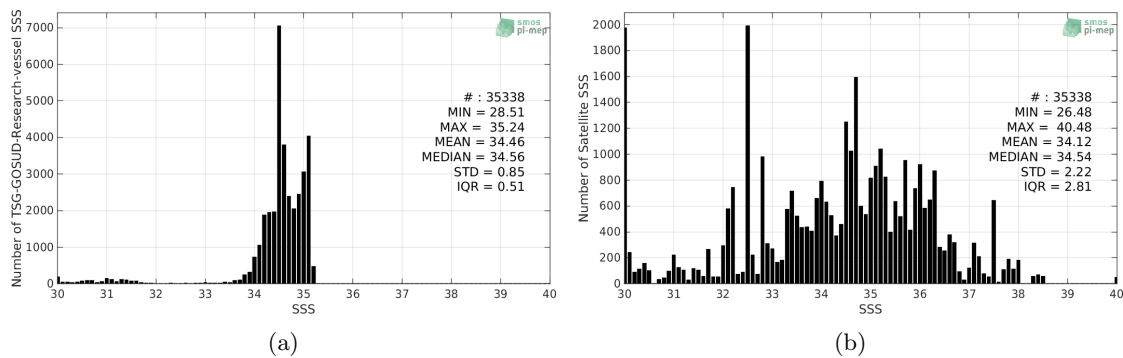
Figure 2: Histograms of SSS from TSG-GOSUD-Research-vessel (a) and SMAP-L2-JPL-V4.2 (b) considering all match-up pairs per bins of 0.1 over the Arctic Ocean Pi-MEP region and for the full satellite product period.
