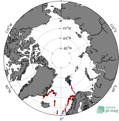
(e) MEAN( \Delta SSS) (Satellite - TSG-GOSUD-Research-vessel)
