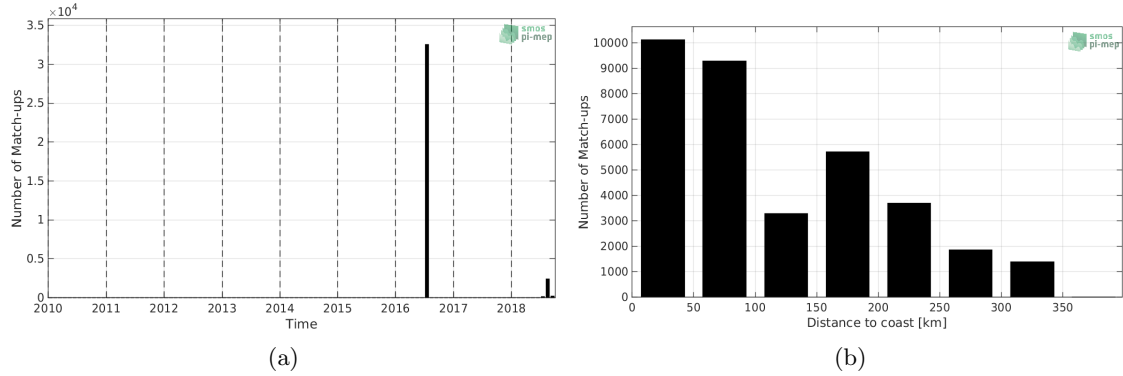
Figure 1: Number of match-ups between TSG-GOSUD-Research-vessel and SMAP-L2-JPL-V4.2 SSS as a function of time (a) and as function of the distance to coast (b) over the Arctic Ocean Pi-MEP region and for the full satellite product period.
