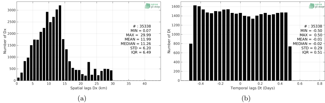
Figure 5: Histograms of the spatial (a) and temporal (b) lags between the time of the TSG-GOSUD-Research-vessel measurements and the date of the corresponding SMAP-L2-JPL-V4.2 SSS product.
