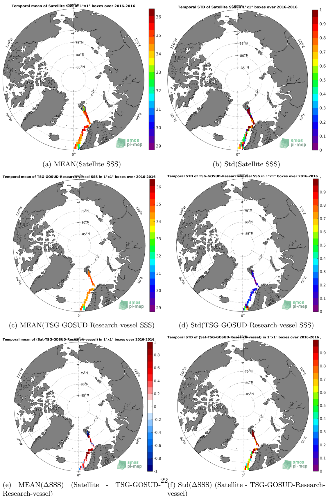
Figure 6: Temporal mean (left) and Std (right) of SSS from SMAP-L2-JPL-V4.2 (top), TSG-GOSUD-Research-vessel (middle), and of \Delta SSS (Satellite - TSG-GOSUD-Research-vessel). Only match-up pairs are used to generate these maps.
