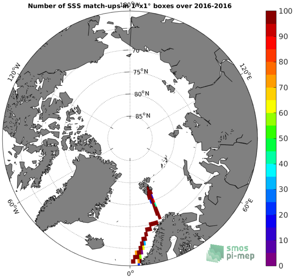
Figure 4: Number of SSS match-ups between TSG-GOSUD-Research-vessel SSS and the SMAP-L2-JPL-V4.2 SSS product for the Arctic Ocean Pi-MEP region over 1^\circ \times 1^\circ boxes and for the full satellite product period.
