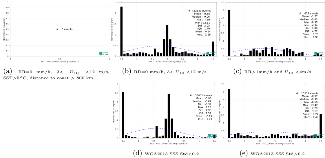
Figure 15: Normalized histogram of \Delta SSS (ISAS v7 - Monthly (Ifremer-LOPS-CMEMS) - TSG (GOSUD-Sailing-ship)) for 5 different subdatasets corresponding to: RR=0 mm/h, 3 < U_{10} < 12 m/s, SST > 5°C, distance to coast > 800 km (a), RR=0 mm/h, 3 < U_{10} < 12 m/s (b), RR > 1mm/h and U_{10} < 4 m/s (c), WOA2013 SSS Std < 0.2 (d), WOA2013 SSS Std > 0.2 (e).
