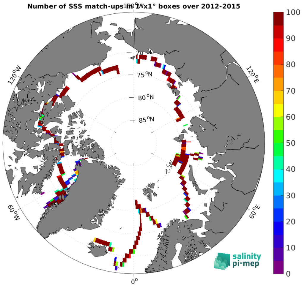
Figure 5: Number of SSS match-ups between TSG (GOSUD-Sailing-ship) SSS and the ISAS v7 - Monthly (Ifremer-LOPS-CMEMS) SSS product for the Arctic Ocean Pi-MEP region over 1^\circ \times 1^\circ boxes and for the full satellite product period.
