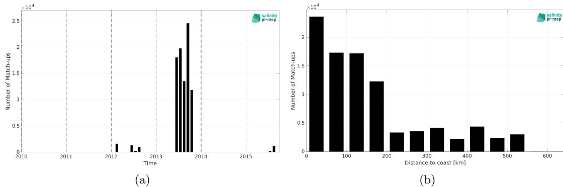
Figure 2: Number of match-ups between TSG (GOSUD-Sailing-ship) and ISAS v7 - Monthly (Ifremer-LOPS-CMEMS) SSS as a function of time (a) and as function of the distance to coast (b) over the Arctic Ocean Pi-MEP region and for the full satellite product period.
