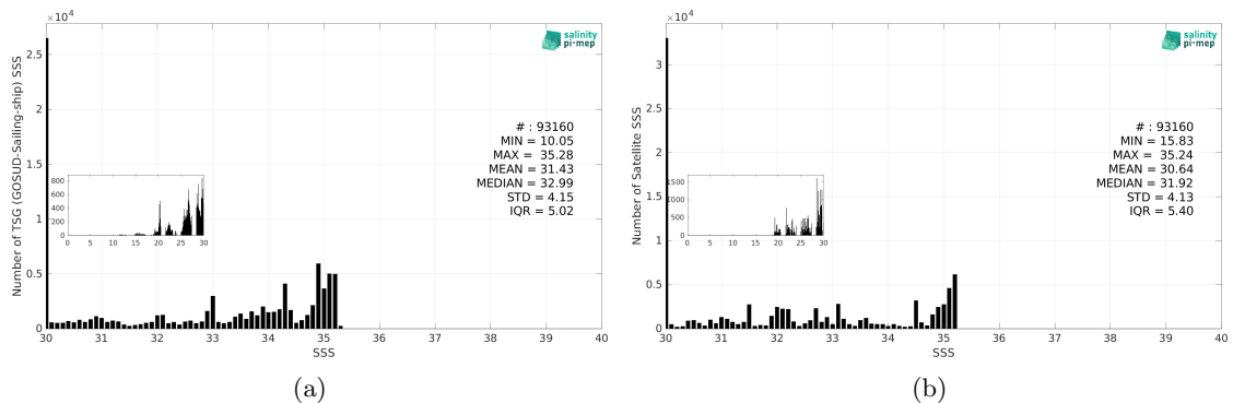
Figure 3: Histograms of SSS from TSG (GOSUD-Sailing-ship) (a) and ISAS v7 - Monthly (Ifremer-LOPS-CMEMS) (b) considering all match-up pairs per bins of 0.1 over the Arctic Ocean Pi-MEP region and for the full satellite product period.
