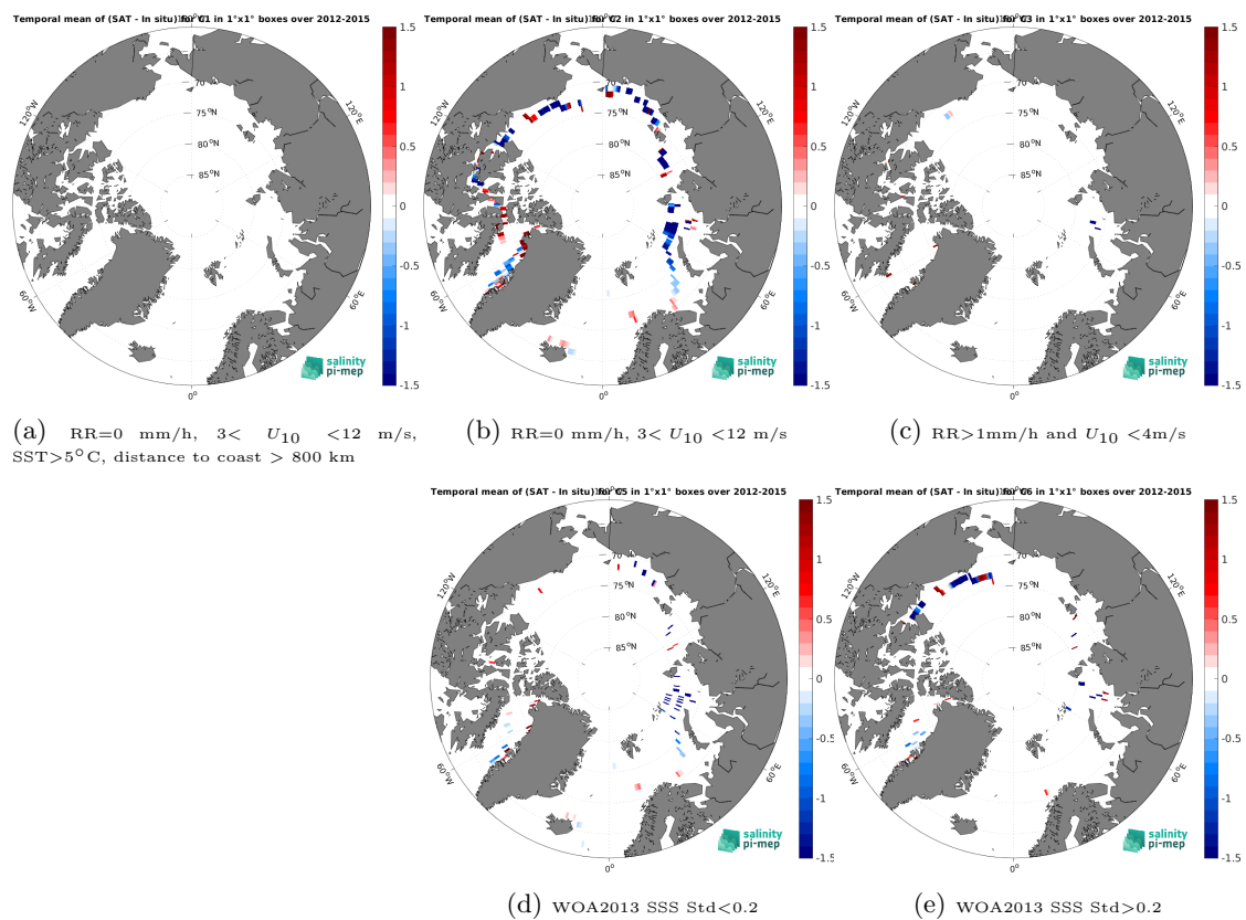
Figure 14: Temporal mean gridded over spatial boxes of size 1^\circ \times 1^\circ of \Delta\text{SSS} (ISAS v7 - Monthly (Ifremer-LOPS-CMEMS) - TSG (GOSUD-Sailing-ship)) for 5 different subdatasets corresponding to:RR=0 mm/h, 3 < U_{10} < 12 m/s, SST>5°C, distance to coast > 800 km (a), RR=0 mm/h, 3 < U_{10} < 12 m/s (b), RR>1mm/h and U_{10} < 4 m/s (c), WOA2013 SSS Std<0.2 (d), WOA2013 SSS Std>0.2 (e).
