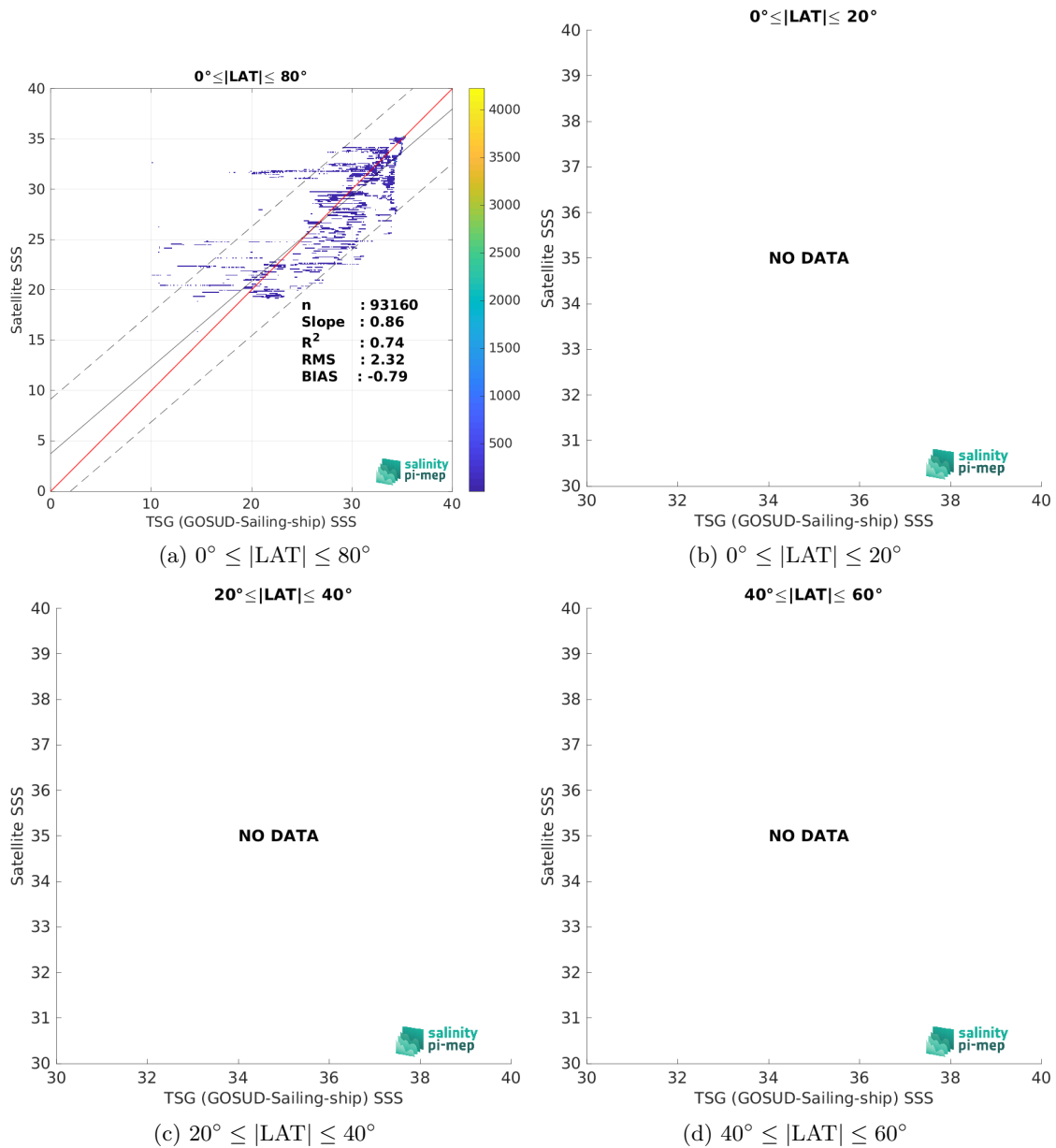
Figure 10: Contour maps of the concentration of ISAS v7 - Monthly (Ifremer-LOPS-CMEMS) SSS (y-axis) versus TSG (GOSUD-Sailing-ship) SSS (x-axis) at match-up pairs for different latitude bands. For each plot, the red line shows x=y . The black thin and dashed lines indicate a linear fit through the data cloud and the \pm 95\% confidence levels, respectively. The number match-up pairs n , the slope and R^2 coefficient of the linear fit, the root mean square (RMS) and the mean bias between satellite and in situ data are indicated for each latitude band in each plots.
