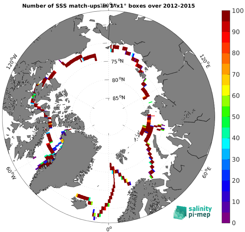
Figure 5: Number of SSS match-ups between TSG (GOSUD-Sailing-ship) SSS and the ISAS SSS product for the Arctic Ocean Pi-MEP region over 1^\circ \times 1^\circ boxes and for the full satellite product period.
