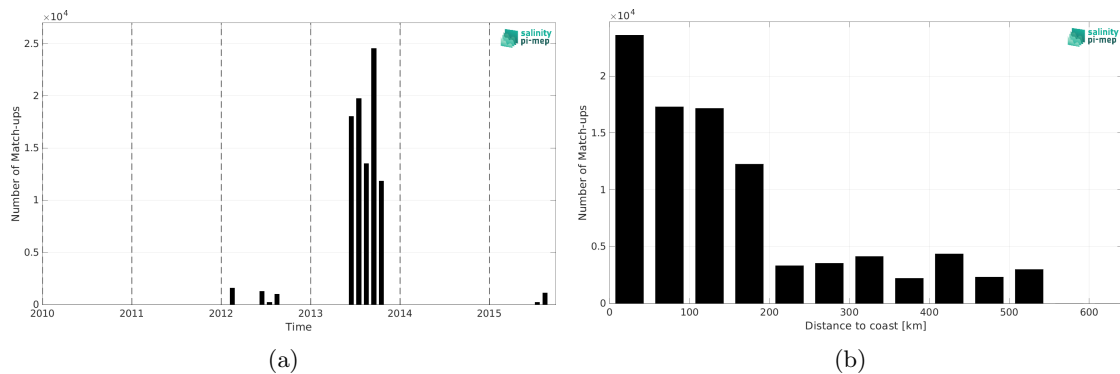
Figure 2: Number of match-ups between TSG (GOSUD-Sailing-ship) and ISAS SSS as a function of time (a) and as function of the distance to coast (b) over the Arctic Ocean Pi-MEP region and for the full satellite product period.
