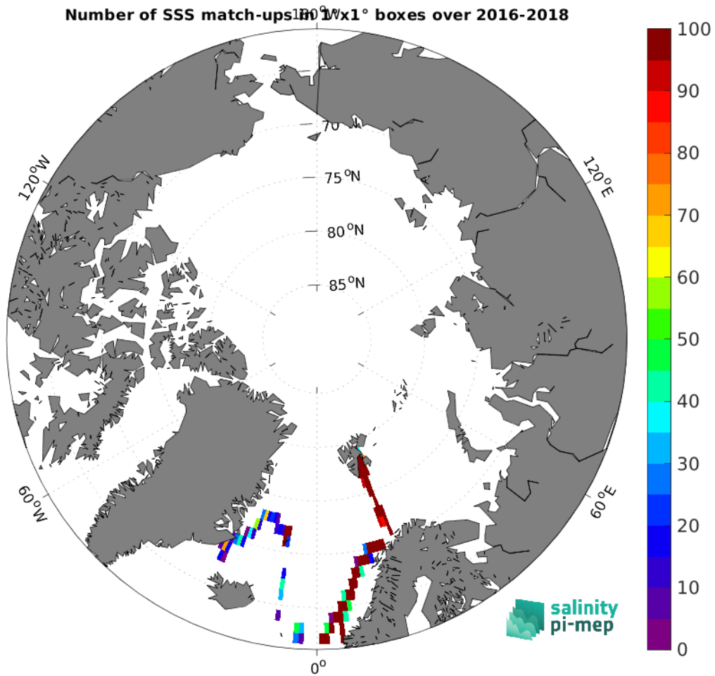
Figure 5: Number of SSS match-ups between TSG (GOSUD-Research-vessel) SSS and the ISAS v7 - Monthly (Ifremer-LOPS-CMEMS) SSS product for the Arctic Ocean Pi-MEP region over 1^\circ \times 1^\circ boxes and for the full satellite product period.
