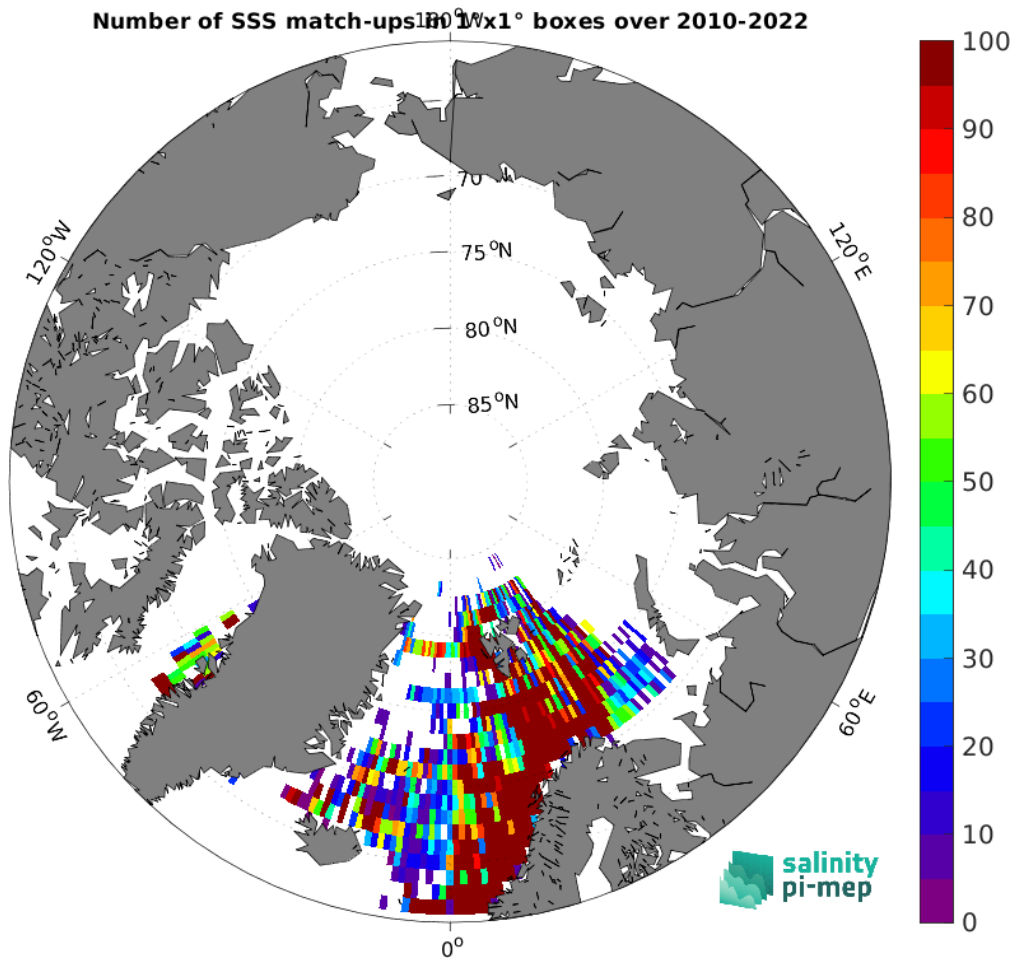
Figure 5: Number of SSS match-ups between ICES SSS and the ISAS v7 - Monthly (Ifremer-LOPS-CMEMS) SSS product for the Arctic Ocean Pi-MEP region over 1^\circ \times 1^\circ boxes and for the full satellite product period.
