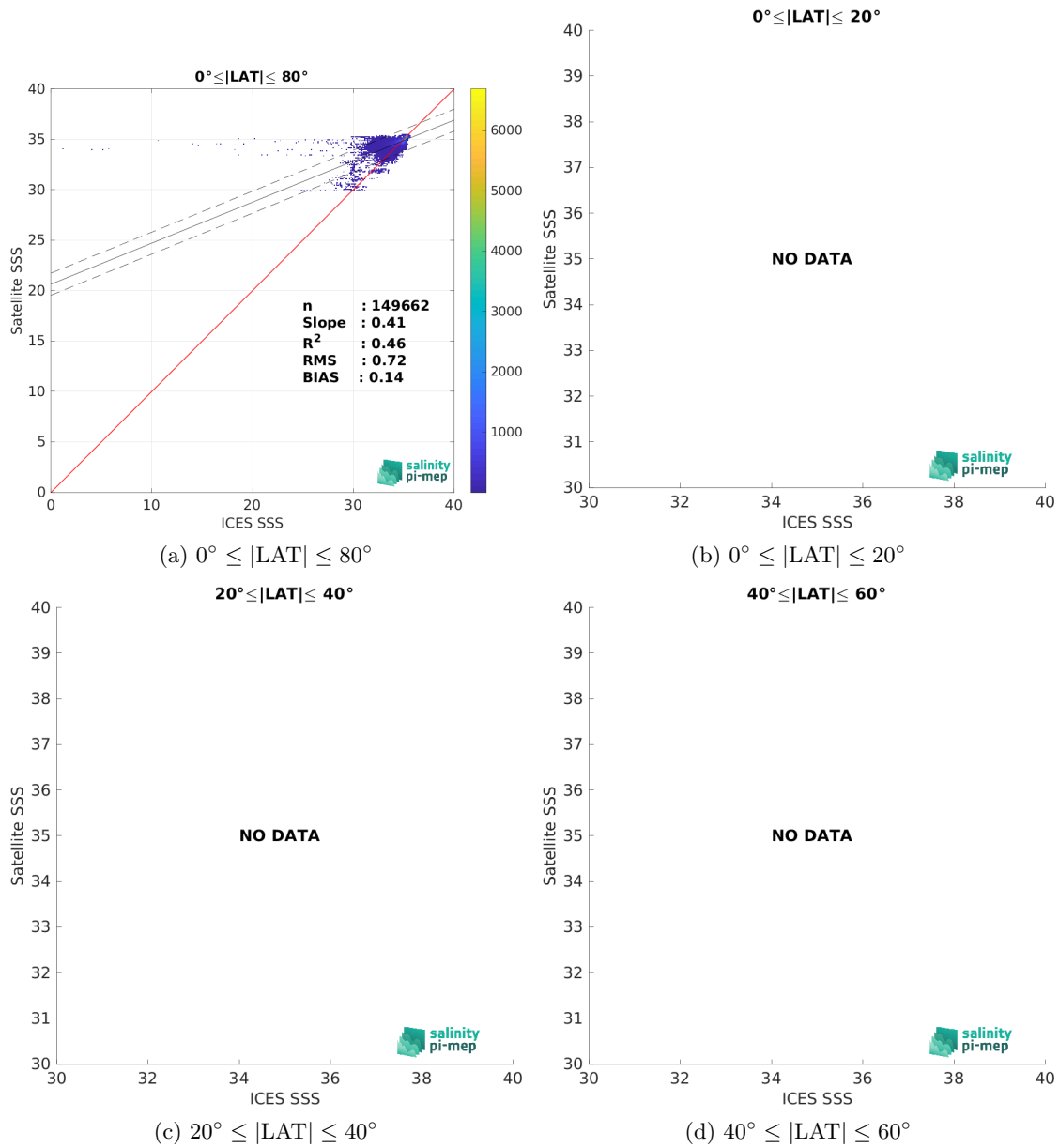
Figure 10: Contour maps of the concentration of ISAS v7 - Monthly (Ifremer-LOPS-CMEMS) SSS (y-axis) versus ICES SSS (x-axis) at match-up pairs for different latitude bands. For each plot, the red line shows x=y . The black thin and dashed lines indicate a linear fit through the data cloud and the \pm 95\% confidence levels, respectively. The number match-up pairs n , the slope and R^2 coefficient of the linear fit, the root mean square (RMS) and the mean bias between satellite and in situ data are indicated for each latitude band in each plots.
