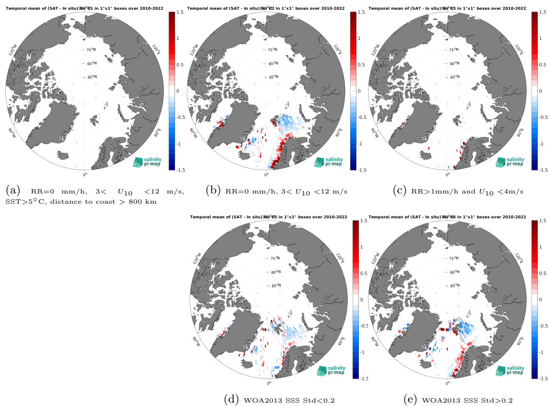
Figure 14: Temporal mean gridded over spatial boxes of size 1^\circ \times 1^\circ of \Delta SSS (ISAS v7 - Monthly (Ifremer-LOPS-CMEMS) - ICES) for 5 different subdatasets corresponding to: RR=0 mm/h, 3 < U_{10} < 12 m/s, SST > 5^\circ\text{C} , distance to coast > 800 km (a), RR=0 mm/h, 3 < U_{10} < 12 m/s (b), RR > 1 mm/h and U_{10} < 4 m/s (c), WOA2013 SSS Std < 0.2 (d), WOA2013 SSS Std > 0.2 (e).
