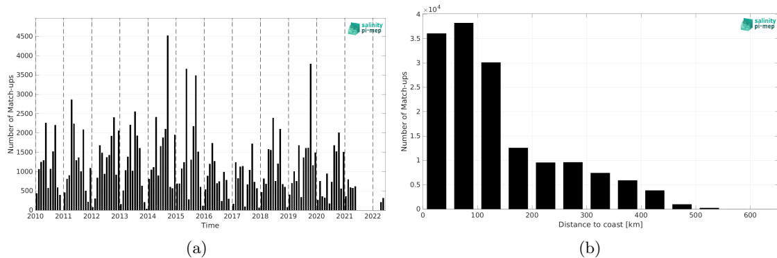
Figure 2: Number of match-ups between ICES and ISAS v7 - Monthly (Ifremer-LOPS-CMEMS) SSS as a function of time (a) and as function of the distance to coast (b) over the Arctic Ocean Pi-MEP region and for the full satellite product period.
