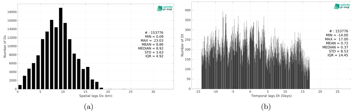
Figure 6: Histograms of the spatial (a) and temporal (b) lags between the location/time of the ICES measurement and the date of the corresponding ISAS SSS pixel.
