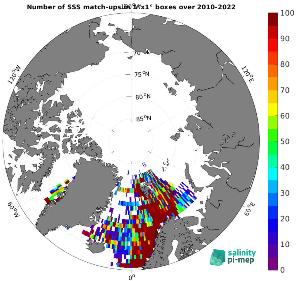
Figure 5: Number of SSS match-ups between ICES SSS and the ISAS SSS product for the Arctic Ocean Pi-MEP region over 1^\circ \times 1^\circ boxes and for the full satellite product period.
