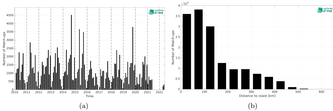
Figure 2: Number of match-ups between ICES and ISAS SSS as a function of time (a) and as function of the distance to coast (b) over the Arctic Ocean Pi-MEP region and for the full satellite product period.
