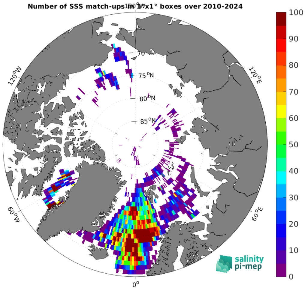
Figure 5: Number of SSS match-ups between Argo SSS and the ISAS v7 - Monthly (Ifremer-LOPS-CMEMS) SSS product for the Arctic Ocean Pi-MEP region over 1^{\circ} \times 1^{\circ} boxes and for the full satellite product period.
