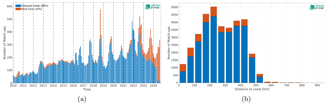
Figure 2: Number of match-ups between Argo and ISAS v7 - Monthly (Ifremer-LOPS-CMEMS) SSS as a function of time (a) and as function of the distance to coast (b) over the Arctic Ocean Pi-MEP region and for the full satellite product period.
