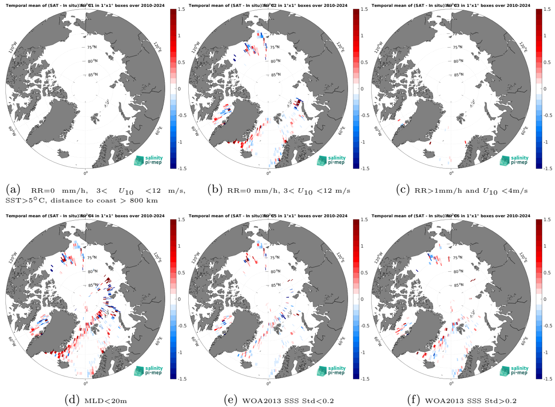
Figure 14: Temporal mean gridded over spatial boxes of size 1^\circ \times 1^\circ of \Delta\text{SSS} (ISAS v7 - Monthly (Ifremer-LOPS-CMEMS) - Argo) for 6 different subdatasets corresponding to:RR=0 mm/h, 3 < U_{10} < 12 m/s, SST>5°C, distance to coast > 800 km (a), RR=0 mm/h, 3 < U_{10} < 12 m/s (b), RR>1mm/h and U_{10} < 4 m/s (c),MLD<20m (d),WOA2013 SSS Std<0.2 (e),WOA2013 SSS Std>0.2 (f).
