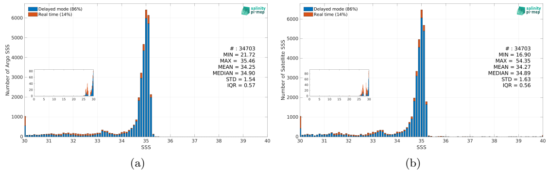
Figure 3: Histograms of SSS from Argo (a) and ISAS v7 - Monthly (Ifremer-LOPS-CMEMS) (b) considering all match-up pairs per bins of 0.1 over the Arctic Ocean Pi-MEP region and for the full satellite product period.
