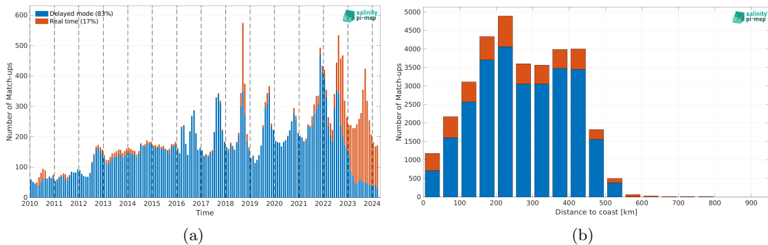
Figure 2: Number of match-ups between Argo and ISAS SSS as a function of time (a) and as function of the distance to coast (b) over the Arctic Ocean Pi-MEP region and for the full satellite product period.
