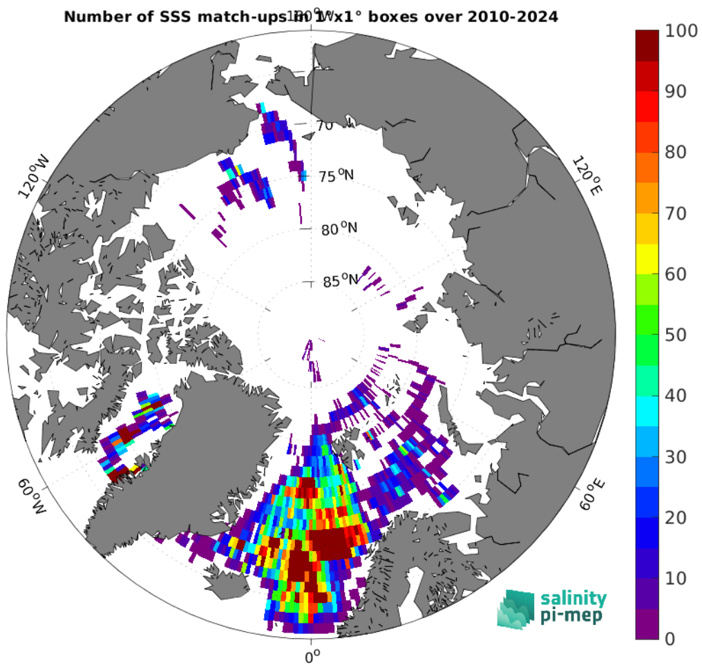
Figure 5: Number of SSS match-ups between Argo SSS and the ISAS SSS product for the Arctic Ocean Pi-MEP region over 1^\circ \times 1^\circ boxes and for the full satellite product period.
