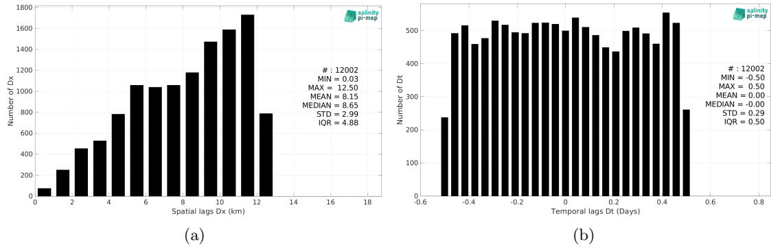
Figure 6: Histograms of the spatial (a) and temporal (b) lags between the location/time of the TSG (SAMOS) measurement and the date of the corresponding CCI SSS L4 POLAR NH Merged-OI v4.41 - 7-day running (ESA) SSS pixel.
