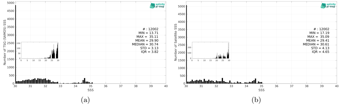
Figure 3: Histograms of SSS from TSG (SAMOS) (a) and CCI SSS L4 POLAR NH Merged-OI v4.41 - 7-day running (ESA) (b) considering all match-up pairs per bins of 0.1 over the Arctic Ocean Pi-MEP region and for the full satellite product period.
