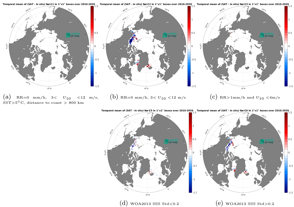
Figure 14: Temporal mean gridded over spatial boxes of size 1^\circ \times 1^\circ of \Delta SSS (CCI SSS L4 POLAR NH Merged-OI v4.41 - 7-day running (ESA) - TSG (SAMOS)) for 5 different subdatasets corresponding to:RR=0 mm/h, 3 < U_{10} < 12 m/s, SST >5^\circ C, distance to coast > 800 km (a), RR=0 mm/h, 3 < U_{10} < 12 m/s (b), RR >1 mm/h and U_{10} < 4 m/s (c), WOA2013 SSS Std <0.2 (d), WOA2013 SSS Std >0.2 (e).
