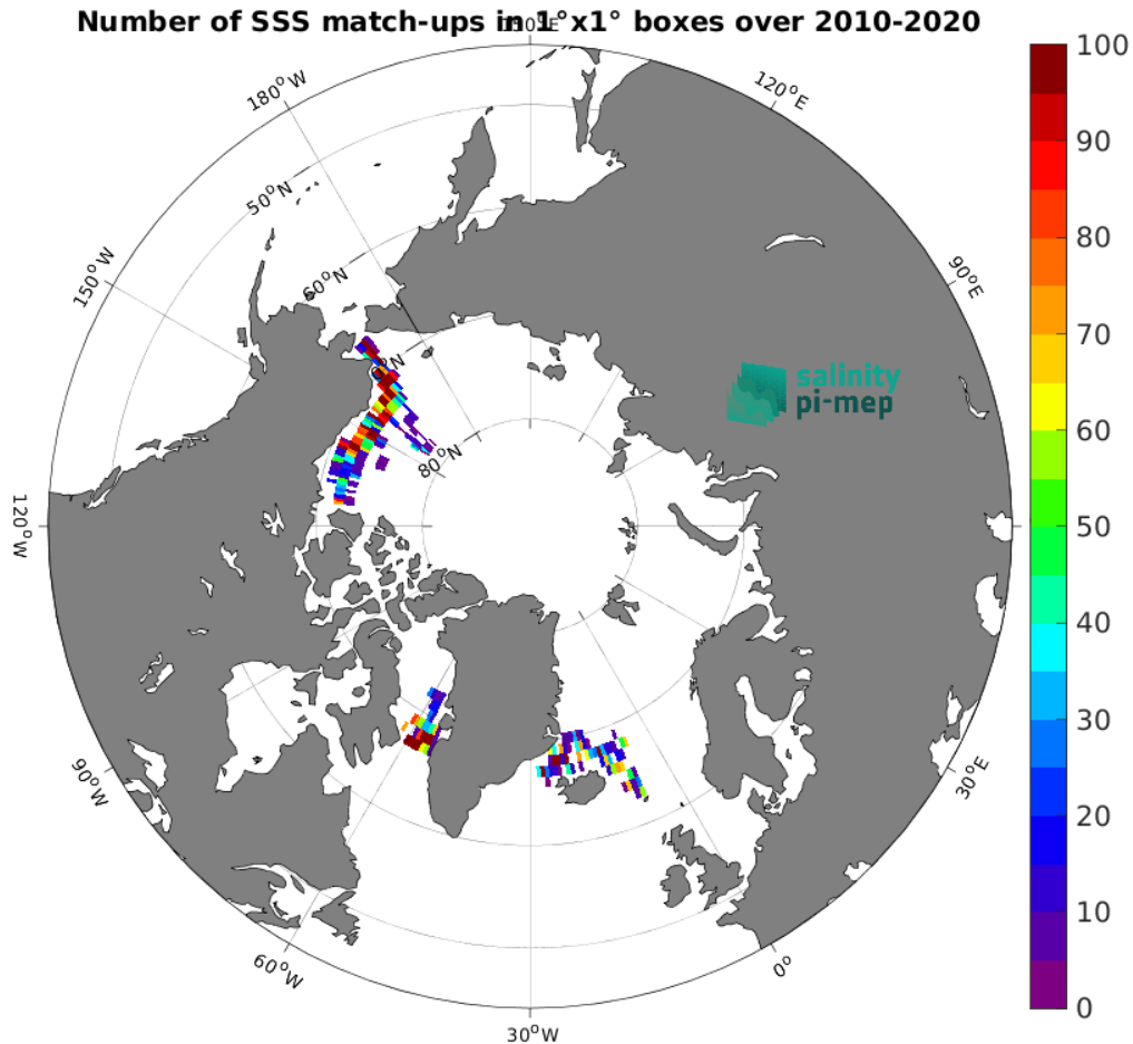
Figure 5: Number of SSS match-ups between TSG (SAMOS) SSS and the CCI SSS L4 POLAR NH Merged-OI v4.41 - 7-day running (ESA) SSS product for the Arctic Ocean Pi-MEP region over 1^\circ \times 1^\circ boxes and for the full satellite product period.
