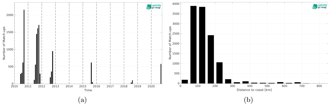
Figure 2: Number of match-ups between TSG (SAMOS) and CCI SSS L4 POLAR NH Merged-OI v4.41 - 7-day running (ESA) SSS as a function of time (a) and as function of the distance to coast (b) over the Arctic Ocean Pi-MEP region and for the full satellite product period.
