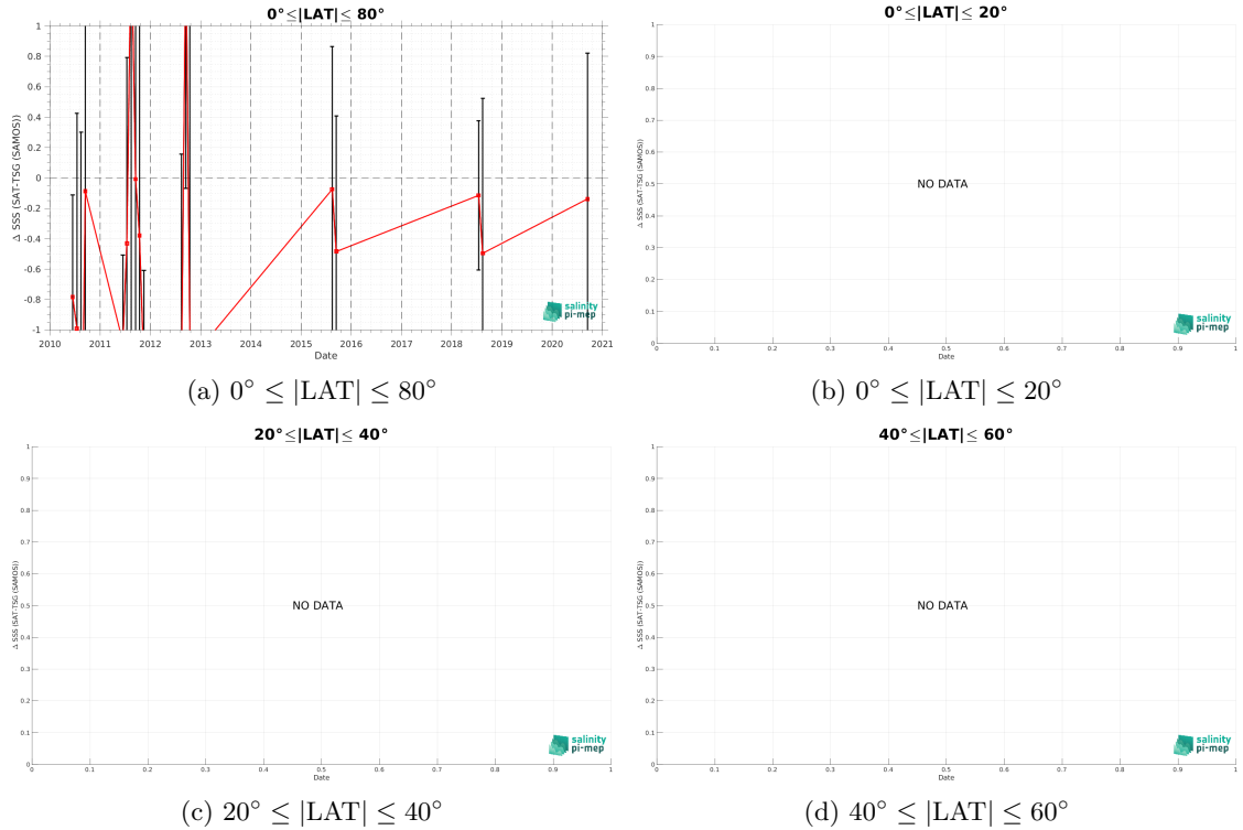
Figure 11: Monthly median (red curves) of \Delta SSS (Satellite - in situ TSG (SAMOS)) and \pm 1 Std (black vertical thick bars) as function of time for all the collected Pi-MEP match-up pairs estimated over the Arctic Ocean Pi-MEP region and for the full satellite product period are shown for different latitude bands: (a) 80^{\circ}\text{S}-80^{\circ}\text{N} , (b) 20^{\circ}\text{S}-20^{\circ}\text{N} , (c) 40^{\circ}\text{S}-20^{\circ}\text{S} and 20^{\circ}\text{N}-40^{\circ}\text{N} and (d) 60^{\circ}\text{S}-40^{\circ}\text{S} and 40^{\circ}\text{N}-60^{\circ}\text{N} .
