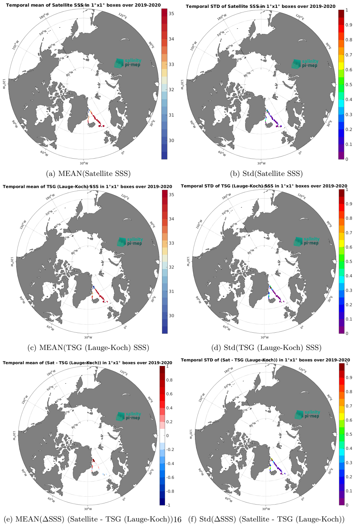
Figure 7: Temporal mean (left) and Std (right) of SSS from CCI SSS L4 POLAR NH Merged-OI v4.41 - 7-day running (ESA) (top), TSG (Lauge-Koch) (middle), and of \Delta SSS (Satellite - TSG (Lauge-Koch)). Only match-up pairs are used to generate these maps.
