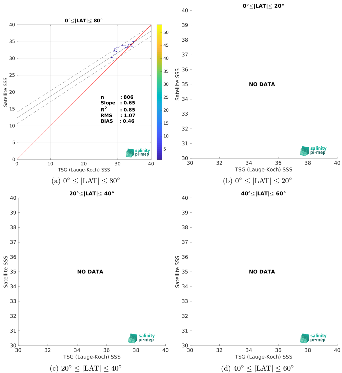
Figure 10: Contour maps of the concentration of CCI SSS L4 POLAR NH Merged-OI v4.41 - 7-day running (ESA) SSS (y-axis) versus TSG (Lauge-Koch) SSS (x-axis) at match-up pairs for different latitude bands. For each plot, the red line shows x=y . The black thin and dashed lines indicate a linear fit through the data cloud and the \pm 95\% confidence levels, respectively. The number match-up pairs n , the slope and R^2 coefficient of the linear fit, the root mean square (RMS) and the mean bias between satellite and in situ data are indicated for each latitude band in each plots.
