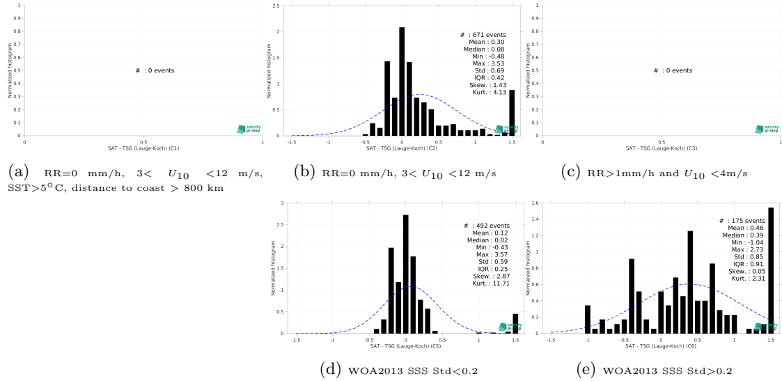
Figure 15: Normalized histogram of \Delta SSS (CCI SSS L4 POLAR NH Merged-OI v4.41 - 7-day running (ESA) - TSG (Lauge-Koch)) for 5 different subdatasets corresponding to: RR=0 mm/h, 3 < U_{10} < 12 m/s, SST > 5°C, distance to coast > 800 km (a), RR=0 mm/h, 3 < U_{10} < 12 m/s (b), RR > 1mm/h and U_{10} < 4 m/s (c), WOA2013 SSS Std < 0.2 (d), WOA2013 SSS Std > 0.2 (e).
