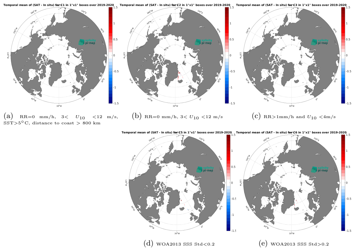
Figure 14: Temporal mean gridded over spatial boxes of size 1^\circ \times 1^\circ of \Delta SSS (CCI SSS L4 POLAR NH Merged-OI v4.41 - 7-day running (ESA) - TSG (Lauge-Koch)) for 5 different subdatasets corresponding to:RR=0 mm/h, 3 < U_{10} < 12 m/s, SST >5^\circ C, distance to coast > 800 km (a), RR=0 mm/h, 3 < U_{10} < 12 m/s (b), RR >1 mm/h and U_{10} < 4 m/s (c), WOA2013 SSS Std <0.2 (d), WOA2013 SSS Std >0.2 (e).
