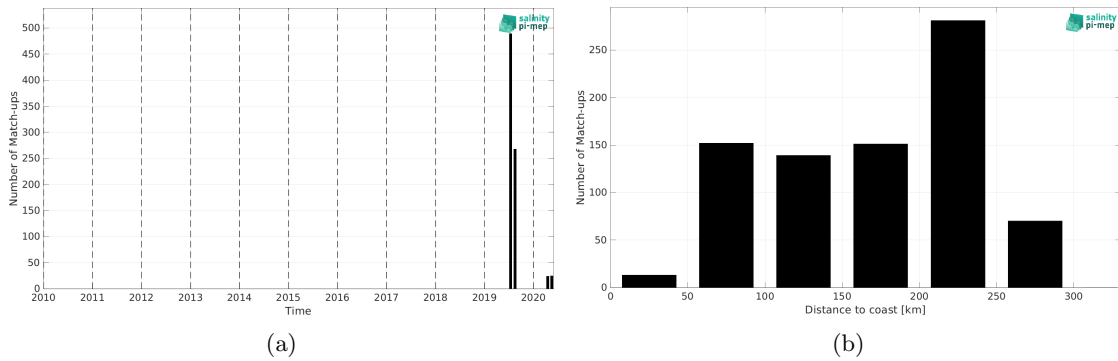
Figure 2: Number of match-ups between TSG (Lauge-Koch) and CCI SSS L4 POLAR NH Merged-OI v4.41 - 7-day running (ESA) SSS as a function of time (a) and as function of the distance to coast (b) over the Arctic Ocean Pi-MEP region and for the full satellite product period.
