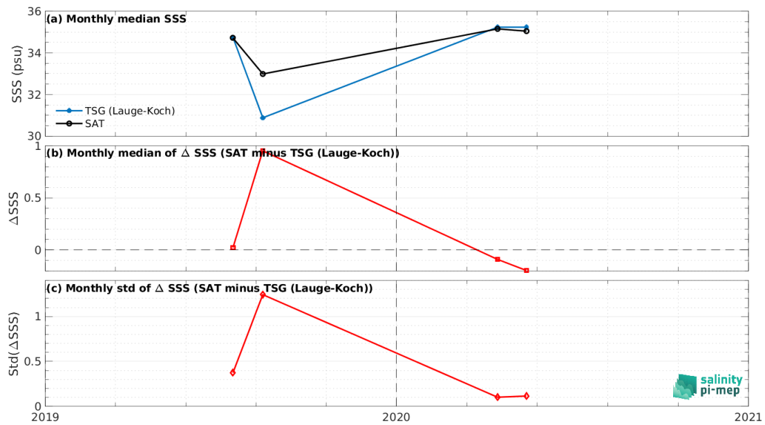
Figure 8: Time series of the monthly median SSS (top), median of \Delta SSS (Satellite - TSG (Lauge-Koch)) and Std of \Delta SSS (Satellite - TSG (Lauge-Koch)) over the Arctic Ocean Pi-MEP region considering all match-ups collected by the Pi-MEP.
