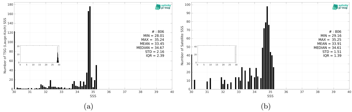
Figure 3: Histograms of SSS from TSG (Lauge-Koch) (a) and CCI SSS L4 POLAR NH Merged-OI v4.41 - 7-day running (ESA) (b) considering all match-up pairs per bins of 0.1 over the Arctic Ocean Pi-MEP region and for the full satellite product period.
