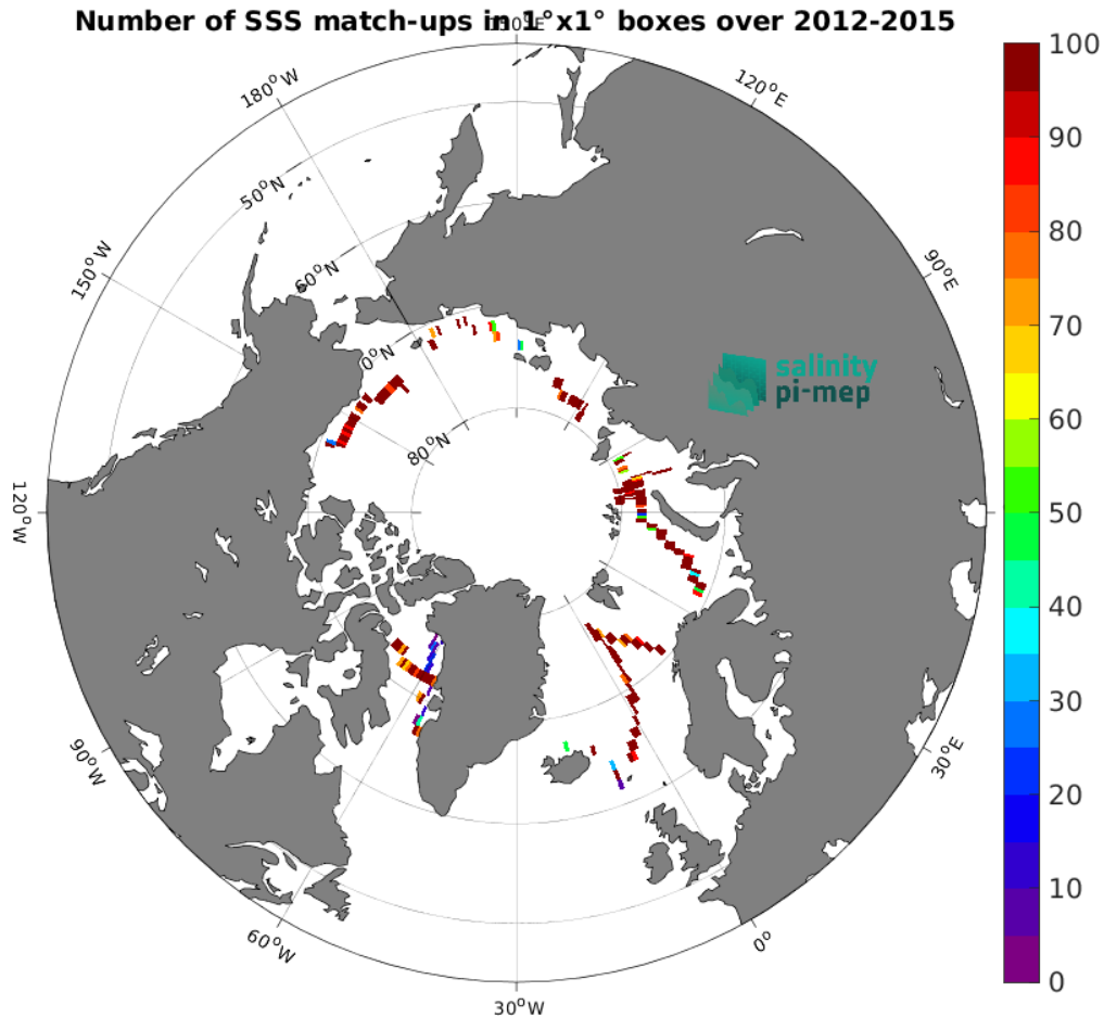
Figure 5: Number of SSS match-ups between TSG (GOSUD-Sailing-ship) SSS and the CCI SSS L4 POLAR NH Merged-OI v4.41 - 7-day running (ESA) SSS product for the Arctic Ocean Pi-MEP region over 1^\circ \times 1^\circ boxes and for the full satellite product period.
