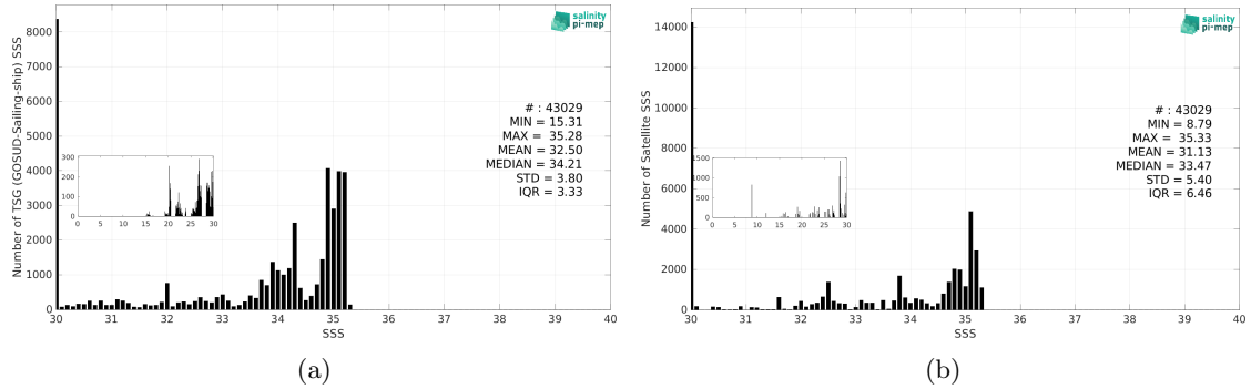
Figure 3: Histograms of SSS from TSG (GOSUD-Sailing-ship) (a) and CCI SSS L4 POLAR NH Merged-OI v4.41 - 7-day running (ESA) (b) considering all match-up pairs per bins of 0.1 over the Arctic Ocean Pi-MEP region and for the full satellite product period.
