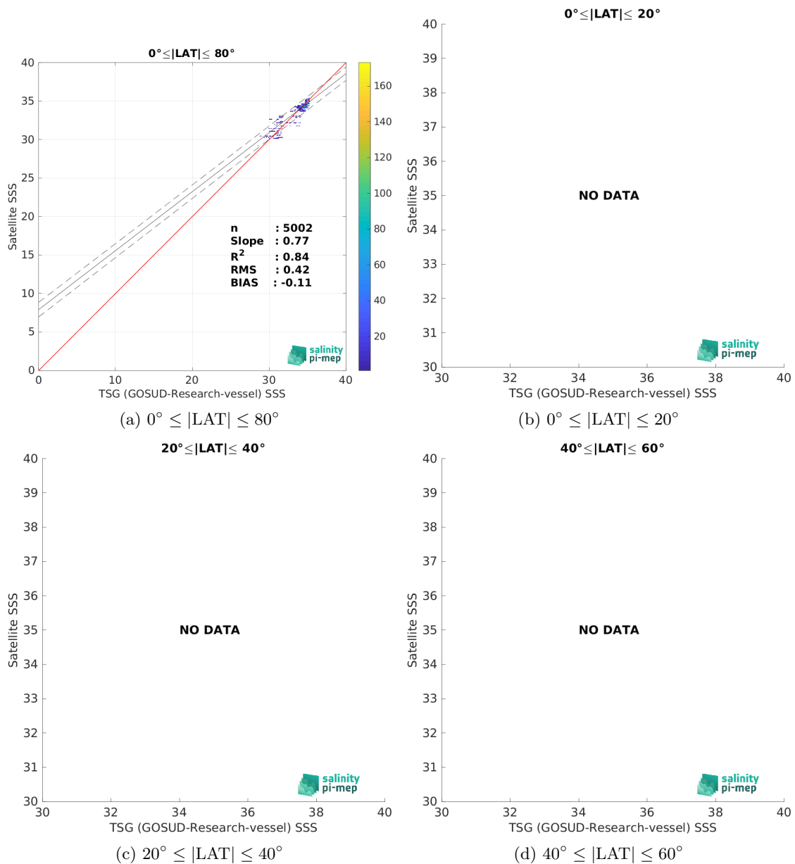
Figure 10: Contour maps of the concentration of CCI SSS L4 POLAR NH Merged-OI v4.41 - 7-day running (ESA) SSS (y-axis) versus TSG (GOSUD-Research-vessel) SSS (x-axis) at match-up pairs for different latitude bands. For each plot, the red line shows x=y . The black thin and dashed lines indicate a linear fit through the data cloud and the \pm 95\% confidence levels, respectively. The number match-up pairs n , the slope and R^2 coefficient of the linear fit, the root mean square (RMS) and the mean bias between satellite and in situ data are indicated for each latitude band in each plots.
