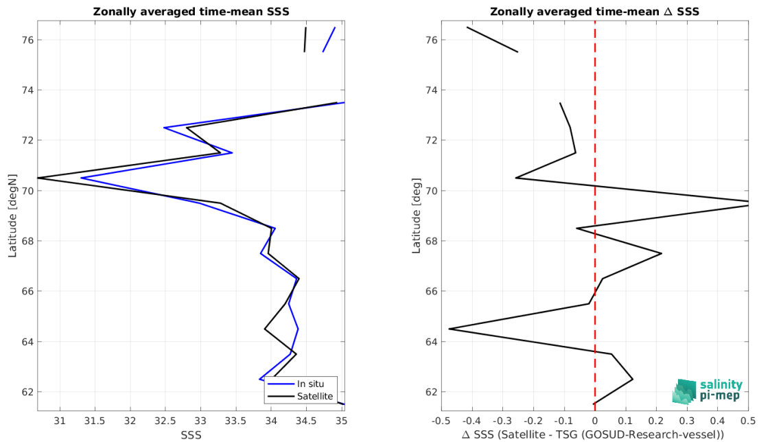
Figure 9: Left panel: Zonal mean SSS from CCI SSS L4 POLAR NH Merged-OI v4.41 - 7-day running (ESA) satellite product (black) and from TSG (GOSUD-Research-vessel) (blue). Right panel: Zonal mean of \Delta SSS (Satellite - TSG (GOSUD-Research-vessel)) for all the collected Pi-MEP match-up pairs estimated over the full satellite product period.
