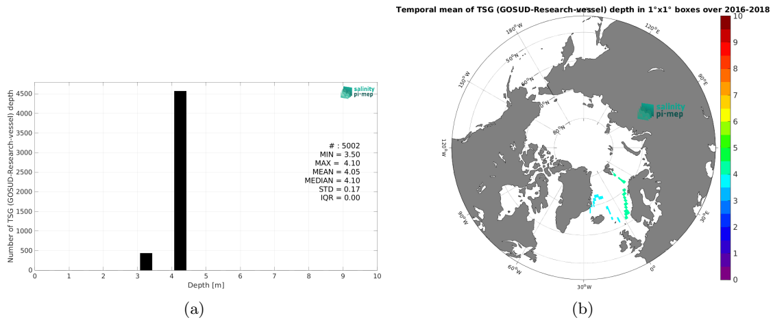
Figure 4: Histograms of the depth of the upper level SSS measurements from TSG (GOSUD-Research-vessel) in the Match-up DataBase for the Arctic Ocean Pi-MEP region (a) and temporal mean spatial distribution of pressure of the in situ SSS data over 1^\circ \times 1^\circ boxes and for the full satellite product period (b).
