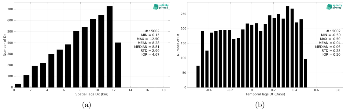
Figure 6: Histograms of the spatial (a) and temporal (b) lags between the location/time of the TSG (GOSUD-Research-vessel) measurement and the date of the corresponding CCI SSS L4 POLAR NH Merged-OI v4.41 - 7-day running (ESA) SSS pixel.
