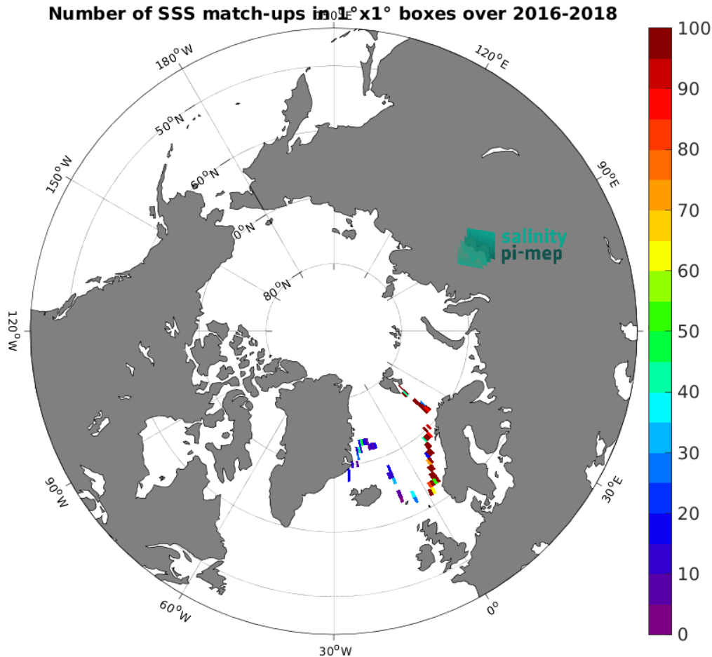
Figure 5: Number of SSS match-ups between TSG (GOSUD-Research-vessel) SSS and the CCI SSS L4 POLAR NH Merged-OI v4.41 - 7-day running (ESA) SSS product for the Arctic Ocean Pi-MEP region over 1^\circ \times 1^\circ boxes and for the full satellite product period.
