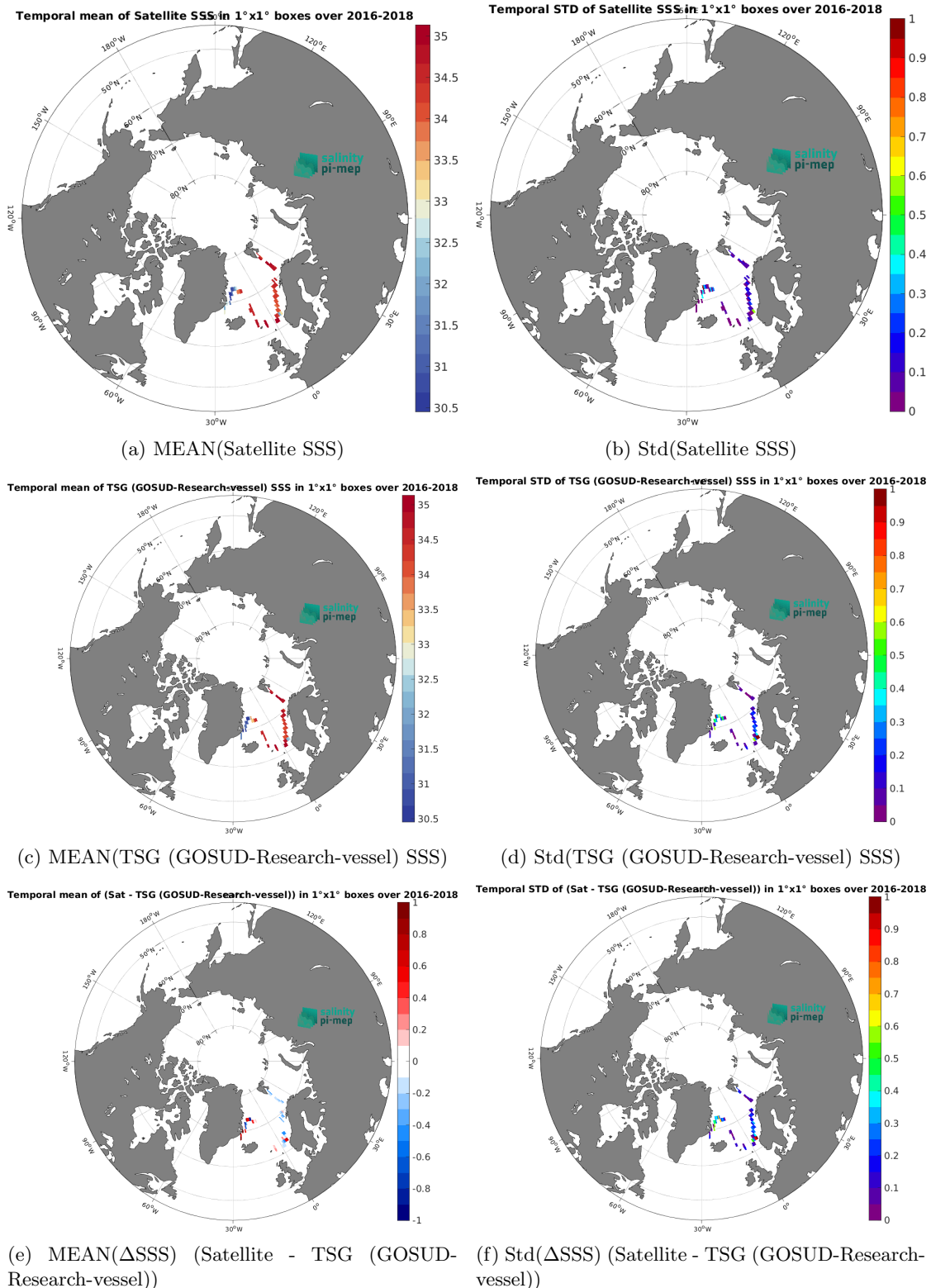
Figure 7: Temporal mean (left) and Std (right) of SSS from CCI SSS L4 POLAR NH Merged-OI v4.41 - 7-day running (ESA) (top), TSG (GOSUD-Research-vessel) (middle), and of \Delta SSS (Satellite - TSG (GOSUD-Research-vessel)). Only match-up pairs are used to generate these maps.
