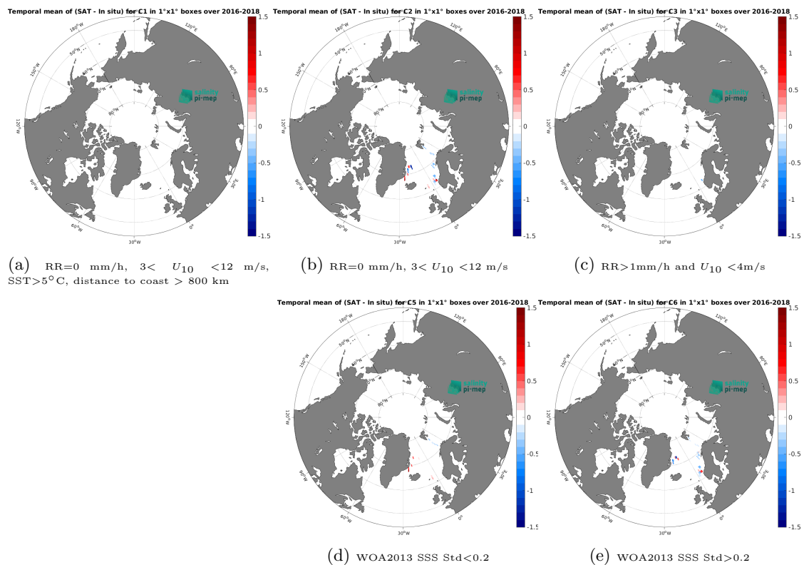
Figure 14: Temporal mean gridded over spatial boxes of size 1^\circ \times 1^\circ of \Delta SSS (CCI SSS L4 POLAR NH Merged-OI v4.41 - 7-day running (ESA) - TSG (GOSUD-Research-vessel)) for 5 different subdatasets corresponding to:RR=0 mm/h, 3 < U_{10} < 12 m/s, SST >5^\circ C, distance to coast > 800 km (a), RR=0 mm/h, 3 < U_{10} < 12 m/s (b), RR >1 mm/h and U_{10} < 4 m/s (c), WOA2013 SSS Std <0.2 (d), WOA2013 SSS Std >0.2 (e).
