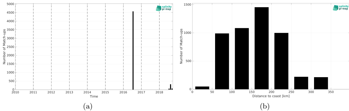
Figure 2: Number of match-ups between TSG (GOSUD-Research-vessel) and CCI SSS L4 POLAR NH Merged-OI v4.41 - 7-day running (ESA) SSS as a function of time (a) and as function of the distance to coast (b) over the Arctic Ocean Pi-MEP region and for the full satellite product period.
