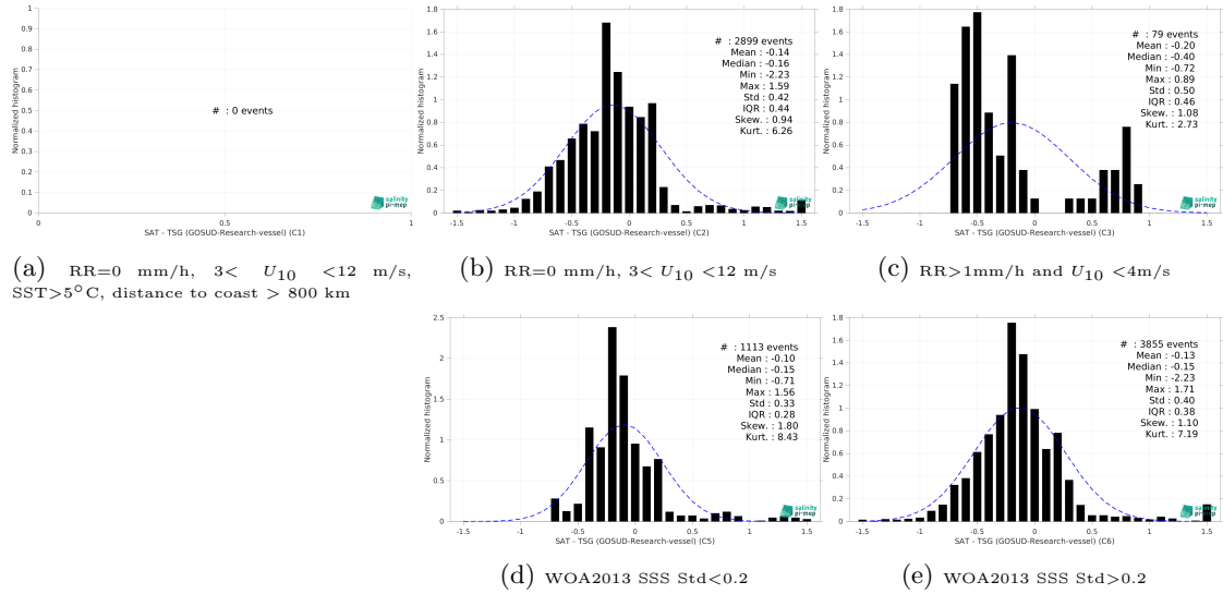
Figure 15: Normalized histogram of \Delta SSS (CCI SSS L4 POLAR NH Merged-OI v4.41 - 7-day running (ESA) - TSG (GOSUD-Research-vessel)) for 5 different subdatasets corresponding to: RR=0 mm/h, 3 < U_{10} < 12 m/s, SST>5°C, distance to coast > 800 km (a), RR=0 mm/h, 3 < U_{10} < 12 m/s (b), RR>1mm/h and U_{10} < 4 m/s (c), WOA2013 SSS Std<0.2 (d), WOA2013 SSS Std>0.2 (e).
