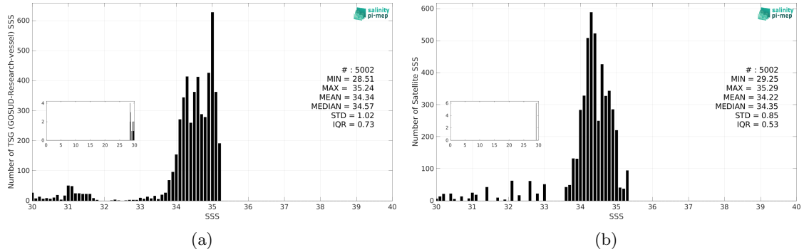
Figure 3: Histograms of SSS from TSG (GOSUD-Research-vessel) (a) and CCI SSS L4 POLAR NH Merged-OI v4.41 - 7-day running (ESA) (b) considering all match-up pairs per bins of 0.1 over the Arctic Ocean Pi-MEP region and for the full satellite product period.
