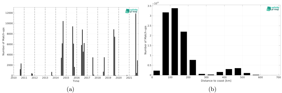
Figure 2: Number of match-ups between TSG (Amundsen) and CCI SSS L4 POLAR NH Merged-OI v4.41 - 7-day running (ESA) SSS as a function of time (a) and as function of the distance to coast (b) over the Arctic Ocean Pi-MEP region and for the full satellite product period.
