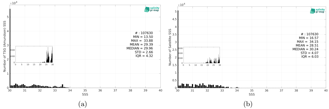
Figure 3: Histograms of SSS from TSG (Amundsen) (a) and CCI SSS L4 POLAR NH Merged-OI v4.41 - 7-day running (ESA) (b) considering all match-up pairs per bins of 0.1 over the Arctic Ocean Pi-MEP region and for the full satellite product period.
