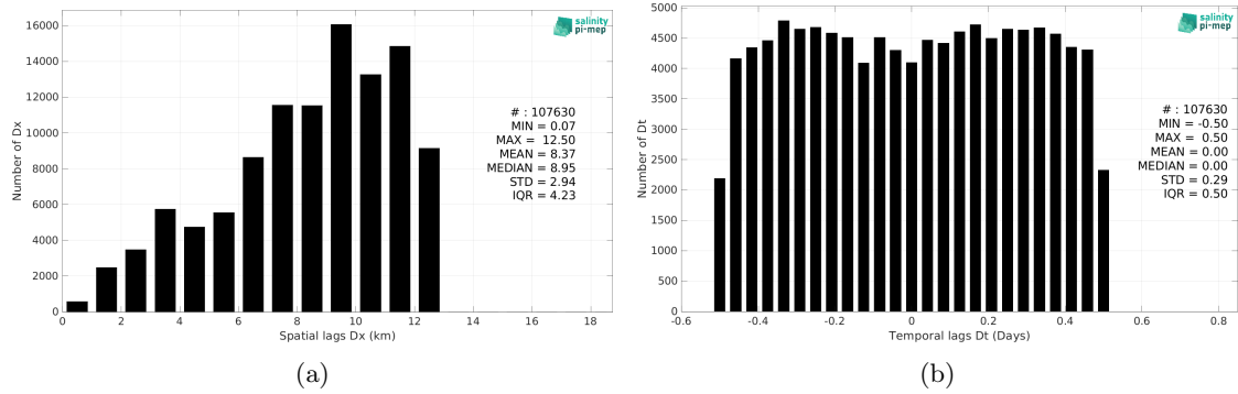
Figure 6: Histograms of the spatial (a) and temporal (b) lags between the location/time of the TSG (Amundsen) measurement and the date of the corresponding CCI SSS L4 POLAR NH Merged-OI v4.41 - 7-day running (ESA) SSS pixel.
