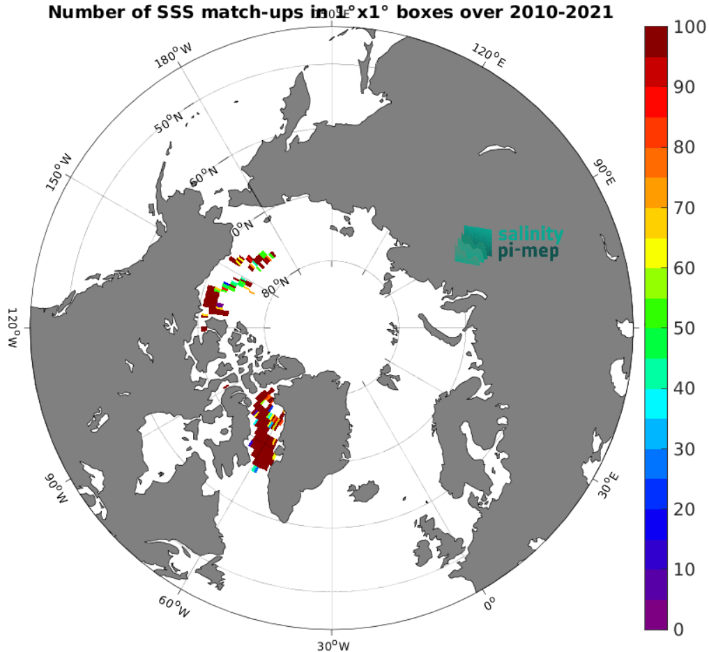
Figure 5: Number of SSS match-ups between TSG (Amundsen) SSS and the CCI SSS L4 POLAR NH Merged-OI v4.41 - 7-day running (ESA) SSS product for the Arctic Ocean Pi-MEP region over 1^\circ \times 1^\circ boxes and for the full satellite product period.
