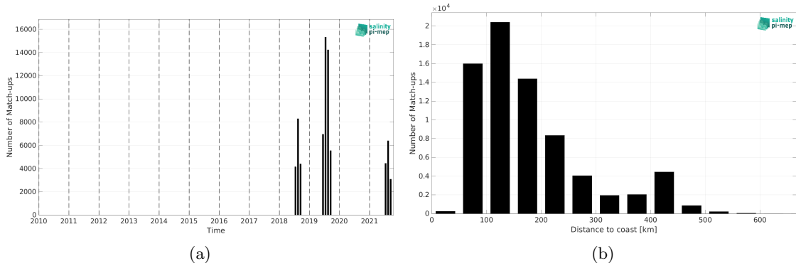
Figure 2: Number of match-ups between Saildrone and CCI SSS L4 POLAR NH Merged-OI v4.41 - 7-day running (ESA) SSS as a function of time (a) and as function of the distance to coast (b) over the Arctic Ocean Pi-MEP region and for the full satellite product period.
