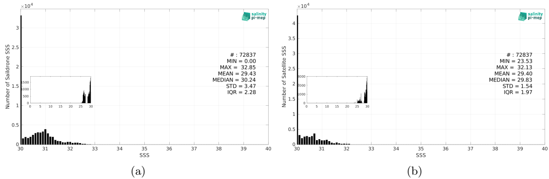
Figure 3: Histograms of SSS from Saildrone (a) and CCI SSS L4 POLAR NH Merged-OI v4.41 - 7-day running (ESA) (b) considering all match-up pairs per bins of 0.1 over the Arctic Ocean Pi-MEP region and for the full satellite product period.
