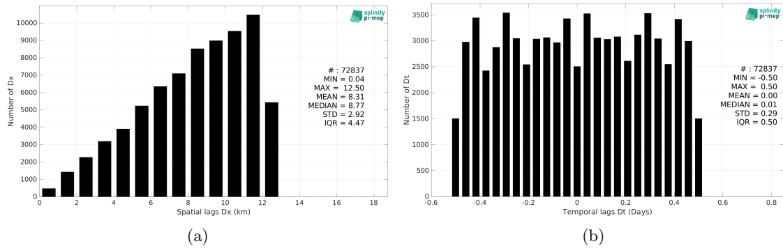
Figure 6: Histograms of the spatial (a) and temporal (b) lags between the location/time of the Saildrone measurement and the date of the corresponding CCI SSS L4 POLAR NH Merged-OI v4.41 - 7-day running (ESA) SSS pixel.
