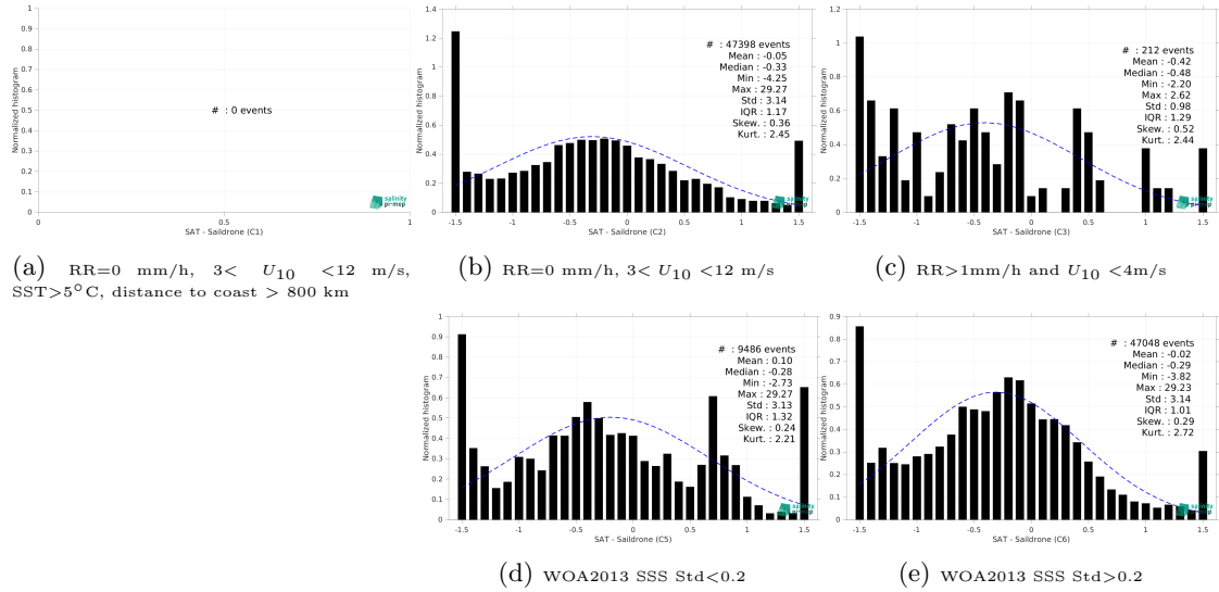
Figure 15: Normalized histogram of \Delta SSS (CCI SSS L4 POLAR NH Merged-OI v4.41 - 7-day running (ESA) - Saldrone) for 5 different subdatasets corresponding to: RR=0 mm/h, 3 < U_{10} < 12 m/s, SST > 5°C, distance to coast > 800 km (a), RR=0 mm/h, 3 < U_{10} < 12 m/s (b), RR > 1mm/h and U_{10} < 4 m/s (c), WOA2013 SSS Std < 0.2 (d), WOA2013 SSS Std > 0.2 (e).
