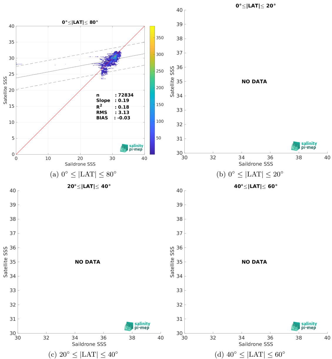
Figure 10: Contour maps of the concentration of CCI SSS L4 POLAR NH Merged-OI v4.41 - 7-day running (ESA) SSS (y-axis) versus Sailldrone SSS (x-axis) at match-up pairs for different latitude bands. For each plot, the red line shows x=y . The black thin and dashed lines indicate a linear fit through the data cloud and the \pm 95\% confidence levels, respectively. The number match-up pairs n , the slope and R^2 coefficient of the linear fit, the root mean square (RMS) and the mean bias between satellite and in situ data are indicated for each latitude band in each plots.
