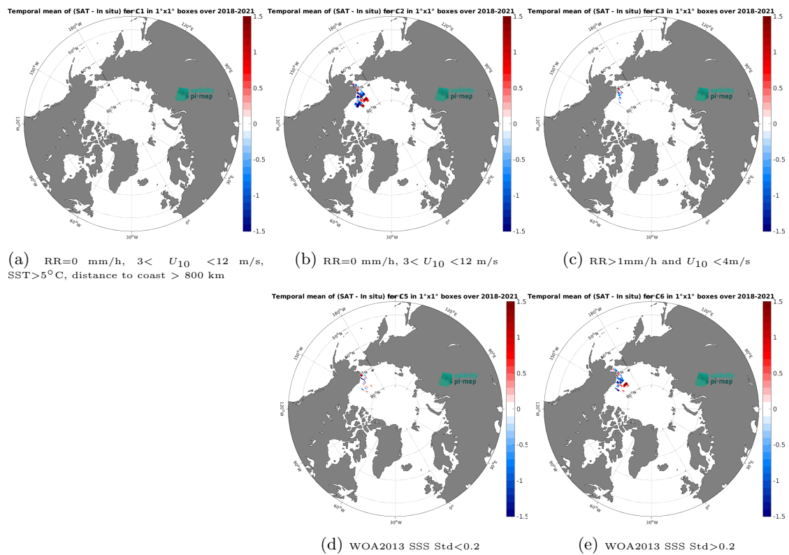
Figure 14: Temporal mean gridded over spatial boxes of size 1^\circ \times 1^\circ of \Delta SSS (CCI SSS L4 POLAR NH Merged-OI v4.41 - 7-day running (ESA) - Sailability) for 5 different subdatasets corresponding to:RR=0 mm/h, 3 < U_{10} < 12 m/s, SST >5^\circ C, distance to coast > 800 km (a), RR=0 mm/h, 3 < U_{10} < 12 m/s (b), RR >1 mm/h and U_{10} < 4 m/s (c), WOA2013 SSS Std <0.2 (d), WOA2013 SSS Std >0.2 (e).
