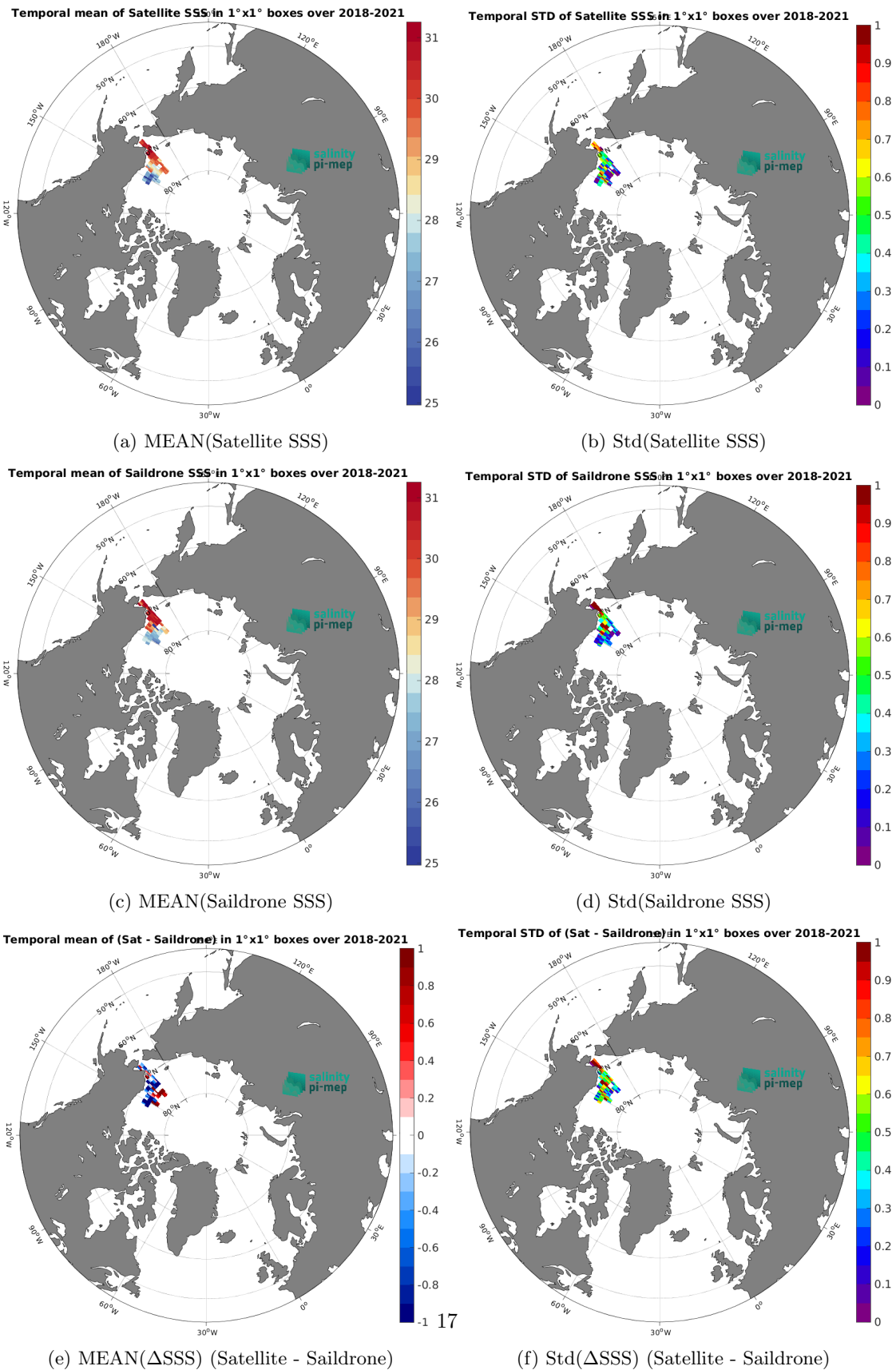
Figure 7: Temporal mean (left) and Std (right) of SSS from CCI SSS L4 POLAR NH Merged-OI v4.41 - 7-day running (ESA) (top), Saildrone (middle), and of \Delta SSS (Satellite - Saildrone). Only match-up pairs are used to generate these maps.
