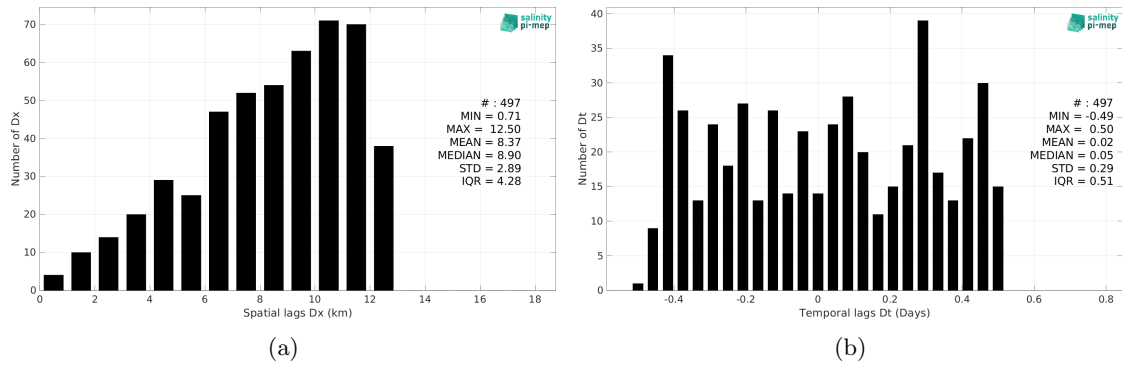
Figure 6: Histograms of the spatial (a) and temporal (b) lags between the location/time of the Marine mammals measurement and the date of the corresponding CCI SSS L4 POLAR NH Merged-OI v4.41 - 7-day running (ESA) SSS pixel.
