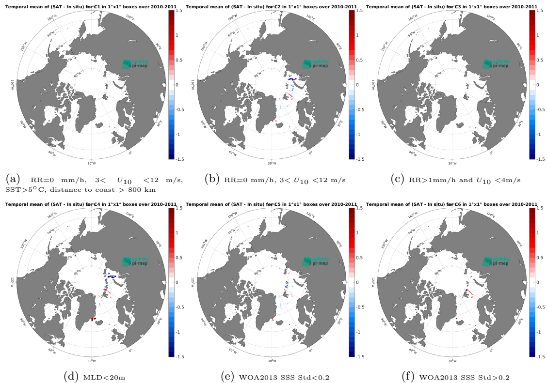
Figure 14: Temporal mean gridded over spatial boxes of size 1^\circ \times 1^\circ of \Delta SSS (CCI SSS L4 POLAR NH Merged-OI v4.41 - 7-day running (ESA) - Marine mammals) for 6 different subdatasets corresponding to:RR=0 mm/h, 3 < U_{10} < 12 m/s, SST > 5^\circ\text{C} , distance to coast > 800 km (a), RR=0 mm/h, 3 < U_{10} < 12 m/s (b), RR > 1 mm/h and U_{10} < 4 m/s (c),MLD < 20 m (d),WOA2013 SSS Std < 0.2 (e),WOA2013 SSS Std > 0.2 (f).
