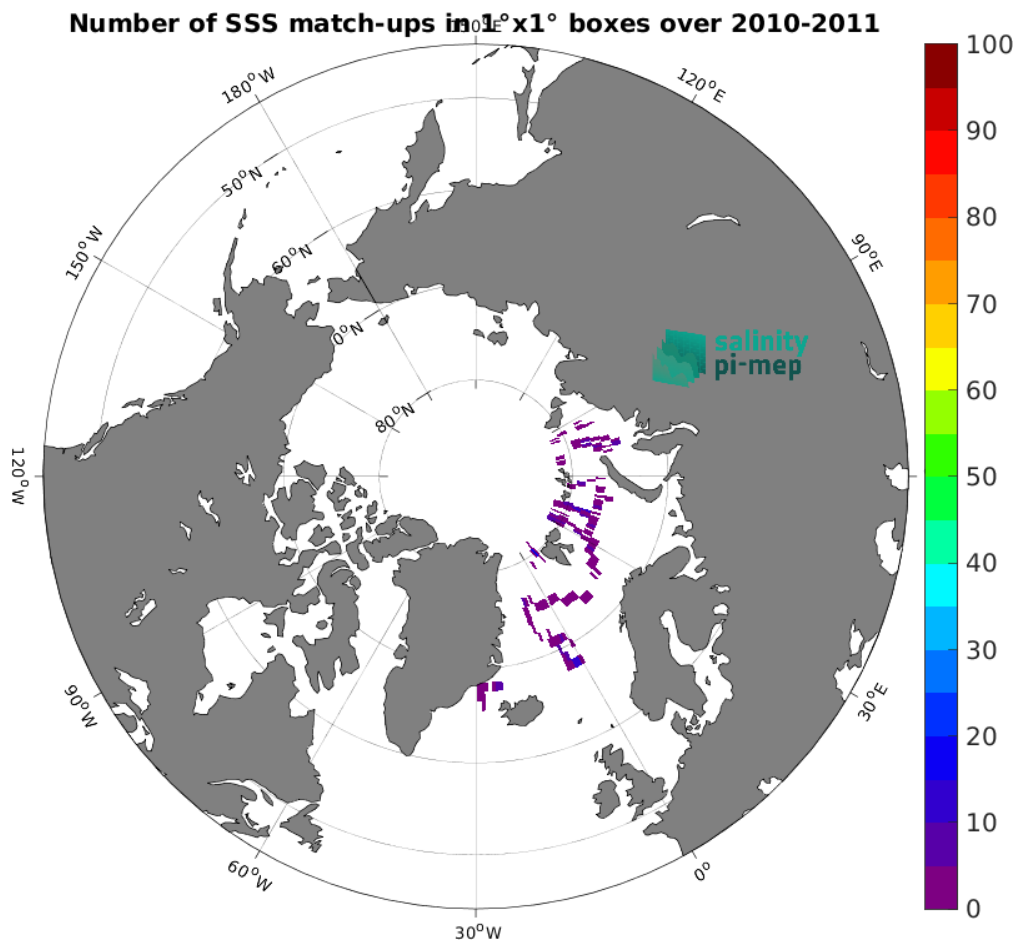
Figure 5: Number of SSS match-ups between Marine mammals SSS and the CCI SSS L4 POLAR NH Merged-OI v4.41 - 7-day running (ESA) SSS product for the Arctic Ocean Pi-MEP region over 1^{\circ} \times 1^{\circ} boxes and for the full satellite product period.
