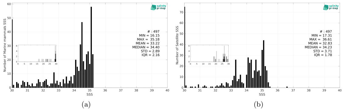
Figure 3: Histograms of SSS from Marine mammals (a) and CCI SSS L4 POLAR NH Merged-OI v4.41 - 7-day running (ESA) (b) considering all match-up pairs per bins of 0.1 over the Arctic Ocean Pi-MEP region and for the full satellite product period.
