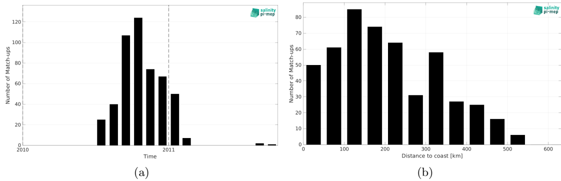
Figure 2: Number of match-ups between Marine mammals and CCI SSS L4 POLAR NH Merged-OI v4.41 - 7-day running (ESA) SSS as a function of time (a) and as function of the distance to coast (b) over the Arctic Ocean Pi-MEP region and for the full satellite product period.
