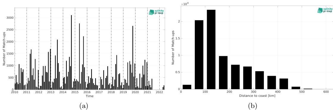
Figure 2: Number of match-ups between ICES and CCI SSS L4 POLAR NH Merged-OI v4.41 - 7-day running (ESA) SSS as a function of time (a) and as function of the distance to coast (b) over the Arctic Ocean Pi-MEP region and for the full satellite product period.
