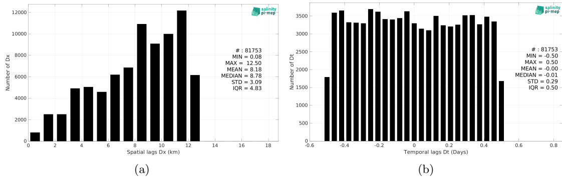
Figure 6: Histograms of the spatial (a) and temporal (b) lags between the location/time of the ICES measurement and the date of the corresponding CCI SSS L4 POLAR NH Merged-OI v4.41 - 7-day running (ESA) SSS pixel.
