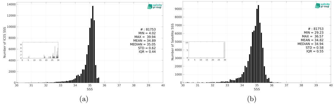
Figure 3: Histograms of SSS from ICES (a) and CCI SSS L4 POLAR NH Merged-OI v4.41 - 7-day running (ESA) (b) considering all match-up pairs per bins of 0.1 over the Arctic Ocean Pi-MEP region and for the full satellite product period.
