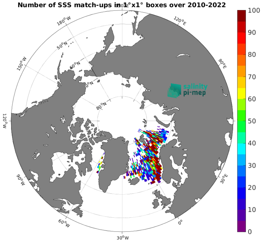
Figure 5: Number of SSS match-ups between ICES SSS and the CCI SSS L4 POLAR NH Merged-OI v4.41 - 7-day running (ESA) SSS product for the Arctic Ocean Pi-MEP region over 1^\circ \times 1^\circ boxes and for the full satellite product period.
