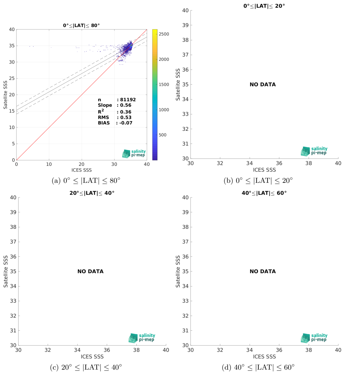
Figure 10: Contour maps of the concentration of CCI SSS L4 POLAR NH Merged-OI v4.41 - 7-day running (ESA) SSS (y-axis) versus ICES SSS (x-axis) at match-up pairs for different latitude bands. For each plot, the red line shows x=y . The black thin and dashed lines indicate a linear fit through the data cloud and the \pm 95\% confidence levels, respectively. The number match-up pairs n , the slope and R^2 coefficient of the linear fit, the root mean square (RMS) and the mean bias between satellite and in situ data are indicated for each latitude band in each plots.
