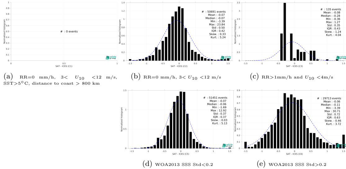
Figure 15: Normalized histogram of \Delta SSS (CCI SSS L4 POLAR NH Merged-OI v4.41 - 7-day running (ESA) - ICES) for 5 different subdatasets corresponding to: RR=0 mm/h, 3 < U_{10} < 12 m/s, SST > 5°C, distance to coast > 800 km (a), RR=0 mm/h, 3 < U_{10} < 12 m/s (b), RR > 1mm/h and U_{10} < 4 m/s (c), WOA2013 SSS Std < 0.2 (d), WOA2013 SSS Std > 0.2 (e).
