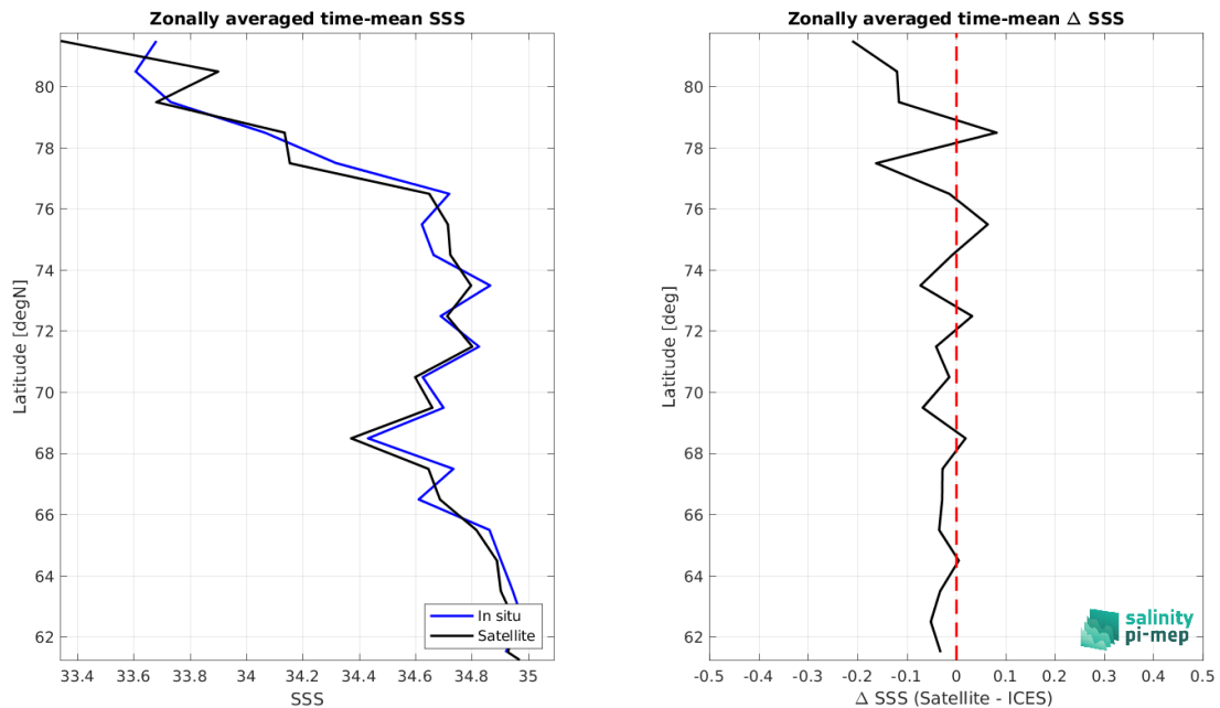
Figure 9: Left panel: Zonal mean SSS from CCI SSS L4 POLAR NH Merged-OI v4.41 - 7-day running (ESA) satellite product (black) and from ICES (blue). Right panel: Zonal mean of \Delta SSS (Satellite - ICES) for all the collected Pi-MEP match-up pairs estimated over the full satellite product period.
