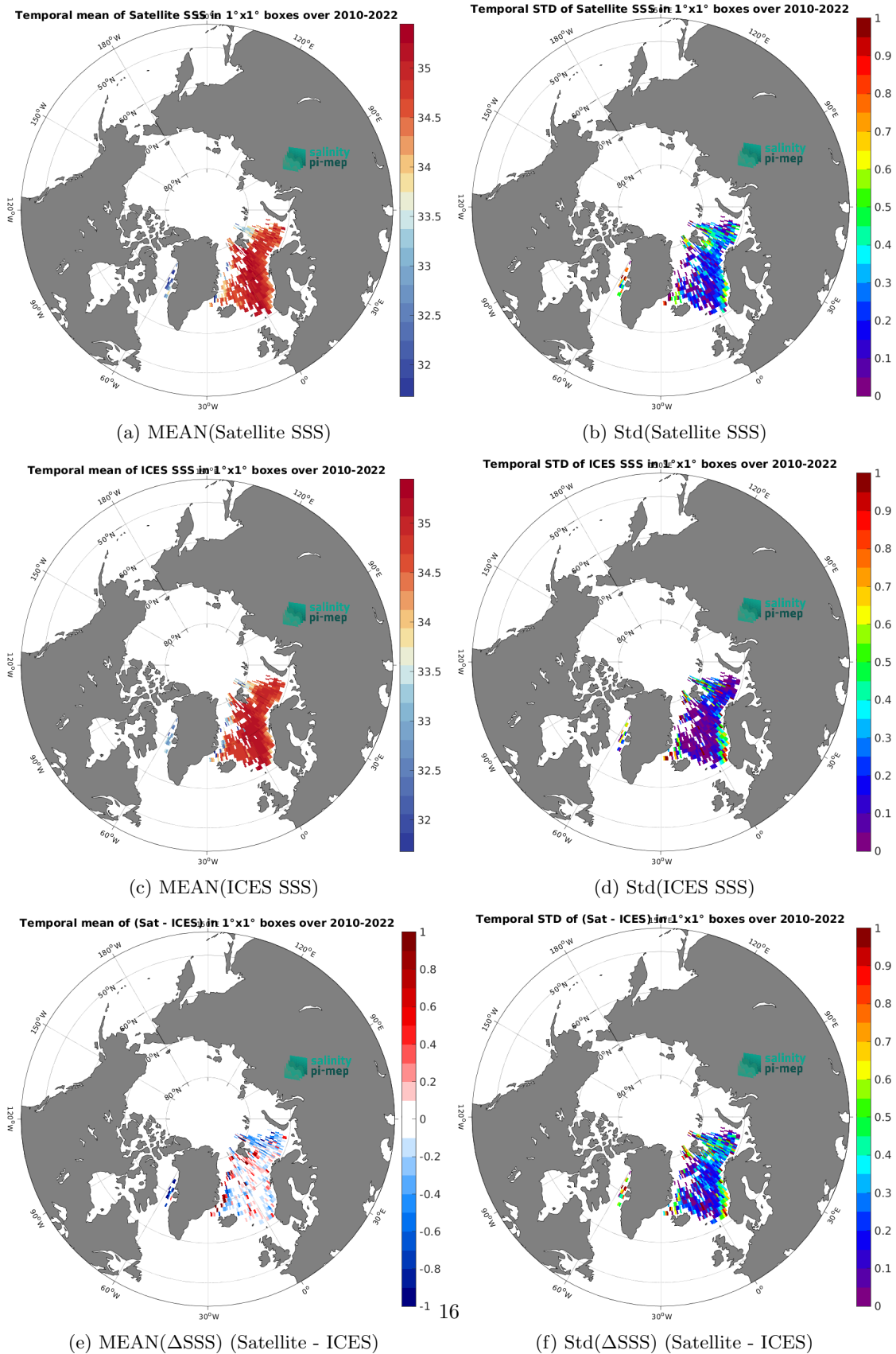
Figure 7: Temporal mean (left) and Std (right) of SSS from CCI SSS L4 POLAR NH Merged-OI v4.41 - 7-day running (ESA) (top), ICES (middle), and of \Delta SSS (Satellite - ICES). Only match-up pairs are used to generate these maps.
