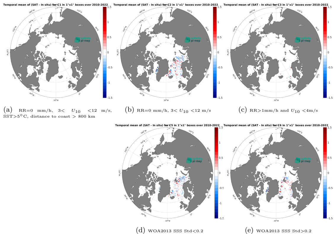
Figure 14: Temporal mean gridded over spatial boxes of size 1^\circ \times 1^\circ of \Delta SSS (CCI SSS L4 POLAR NH Merged-OI v4.41 - 7-day running (ESA) - ICES) for 5 different subdatasets corresponding to:RR=0 mm/h, 3 < U_{10} < 12 m/s, SST >5^\circ C, distance to coast > 800 km (a), RR=0 mm/h, 3 < U_{10} < 12 m/s (b), RR >1 mm/h and U_{10} < 4 m/s (c), WOA2013 SSS Std <0.2 (d), WOA2013 SSS Std >0.2 (e).
