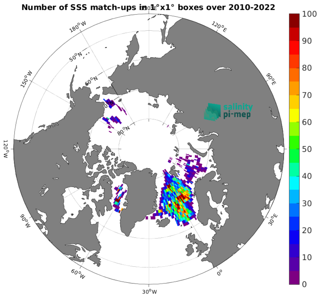
Figure 5: Number of SSS match-ups between Argo SSS and the CCI SSS L4 POLAR NH Merged-OI v4.41 - 7-day running (ESA) SSS product for the Arctic Ocean Pi-MEP region over 1^{\circ} \times 1^{\circ} boxes and for the full satellite product period.
