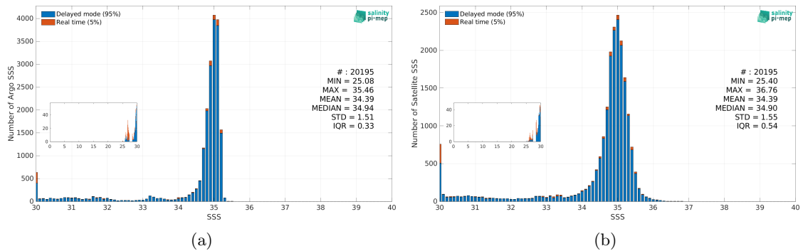
Figure 3: Histograms of SSS from Argo (a) and CCI SSS L4 POLAR NH Merged-OI v4.41 - 7-day running (ESA) (b) considering all match-up pairs per bins of 0.1 over the Arctic Ocean Pi-MEP region and for the full satellite product period.
