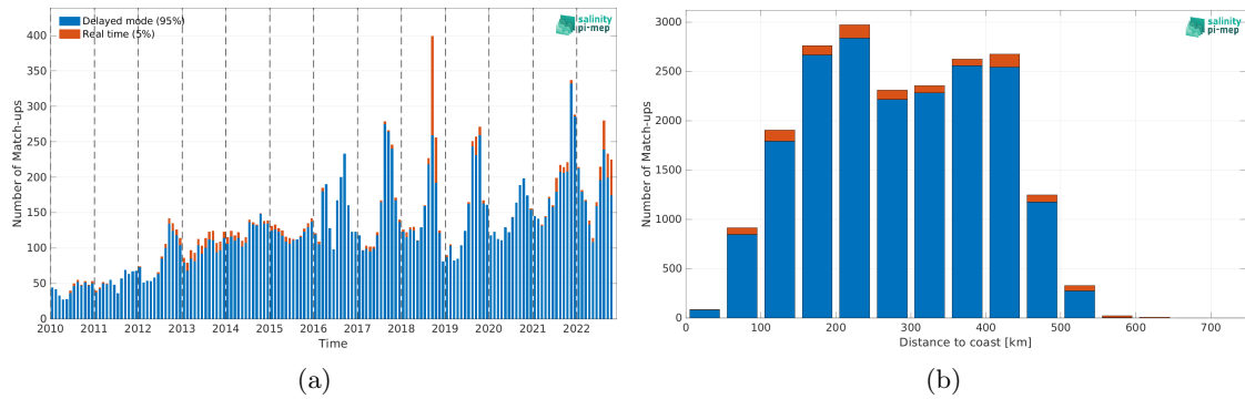
Figure 2: Number of match-ups between Argo and CCI SSS L4 POLAR NH Merged-OI v4.41 - 7-day running (ESA) SSS as a function of time (a) and as function of the distance to coast (b) over the Arctic Ocean Pi-MEP region and for the full satellite product period.
