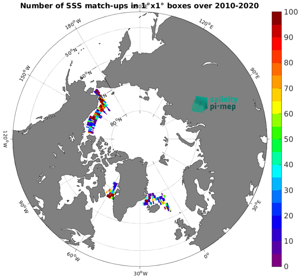
Figure 5: Number of SSS match-ups between TSG (SAMOS) SSS and the CCI SSS L4 POLAR NH Merged-OI v4.41 - 30-day running (ESA) SSS product for the Arctic Ocean Pi-MEP region over 1^\circ \times 1^\circ boxes and for the full satellite product period.
