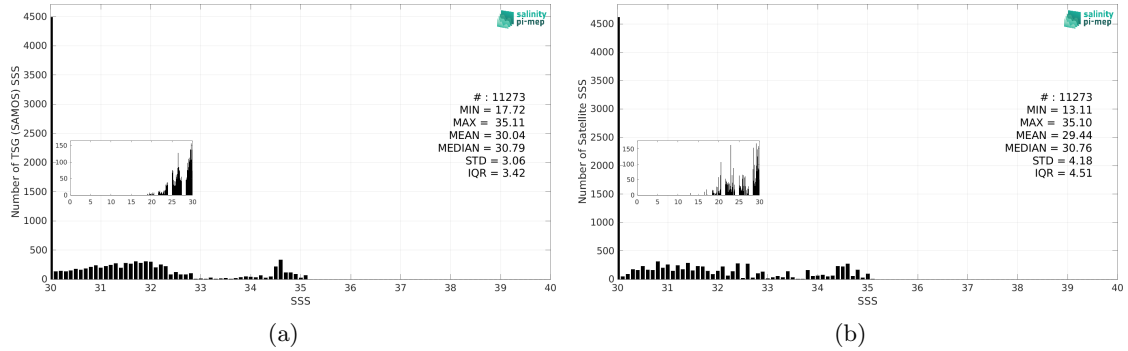
Figure 3: Histograms of SSS from TSG (SAMOS) (a) and CCI SSS L4 POLAR NH Merged-OI v4.41 - 30-day running (ESA) (b) considering all match-up pairs per bins of 0.1 over the Arctic Ocean Pi-MEP region and for the full satellite product period.
