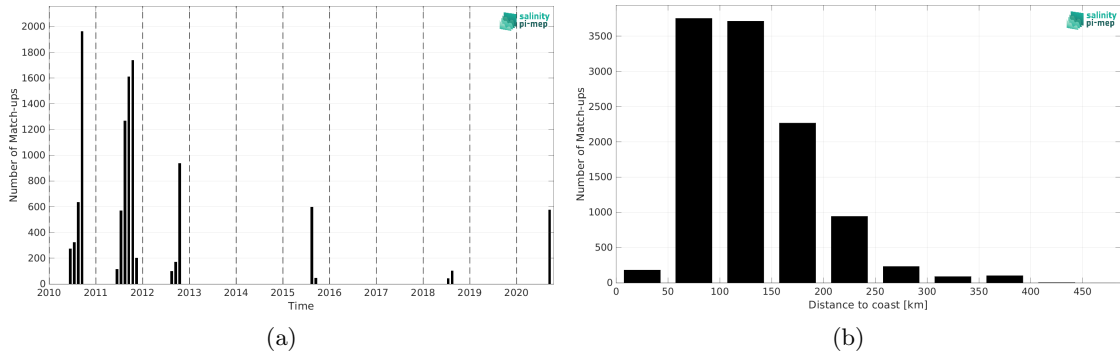
Figure 2: Number of match-ups between TSG (SAMOS) and CCI SSS L4 POLAR NH Merged-OI v4.41 - 30-day running (ESA) SSS as a function of time (a) and as function of the distance to coast (b) over the Arctic Ocean Pi-MEP region and for the full satellite product period.
