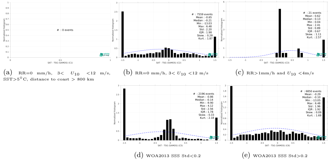
Figure 15: Normalized histogram of \Delta\text{SSS} (CCI SSS L4 POLAR NH Merged-OI v4.41 - 30-day running (ESA) - TSG (SAMOS)) for 5 different subdatasets corresponding to: RR=0 mm/h, 3 < U_{10} < 12 m/s, SST > 5^\circ\text{C} , distance to coast > 800 km (a), RR=0 mm/h, 3 < U_{10} < 12 m/s (b), RR > 1\text{mm/h} and U_{10} < 4\text{m/s} (c), WOA2013 SSS Std < 0.2 (d), WOA2013 SSS Std > 0.2 (e).
