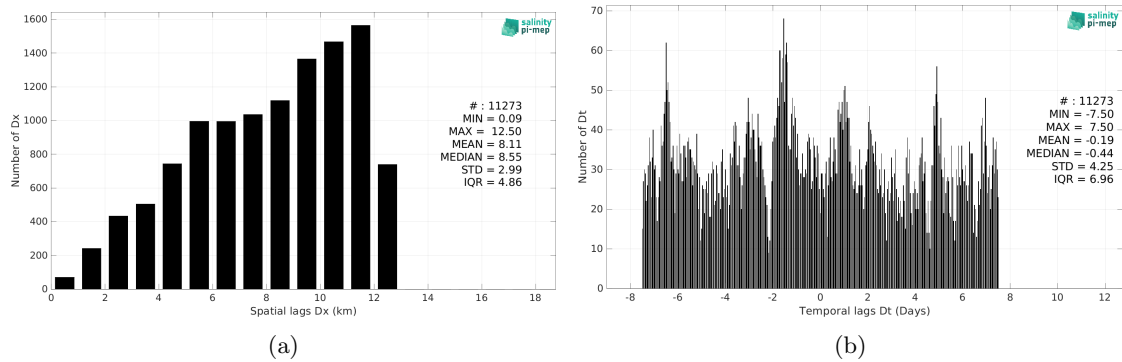
Figure 6: Histograms of the spatial (a) and temporal (b) lags between the location/time of the TSG (SAMOS) measurement and the date of the corresponding CCI SSS L4 POLAR NH Merged-OI v4.41 - 30-day running (ESA) SSS pixel.
