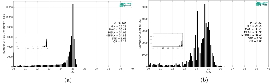
Figure 3: Histograms of SSS from TSG (Polarstern) (a) and CCI SSS L4 POLAR NH Merged-OI v4.41 - 30-day running (ESA) (b) considering all match-up pairs per bins of 0.1 over the Arctic Ocean Pi-MEP region and for the full satellite product period.
